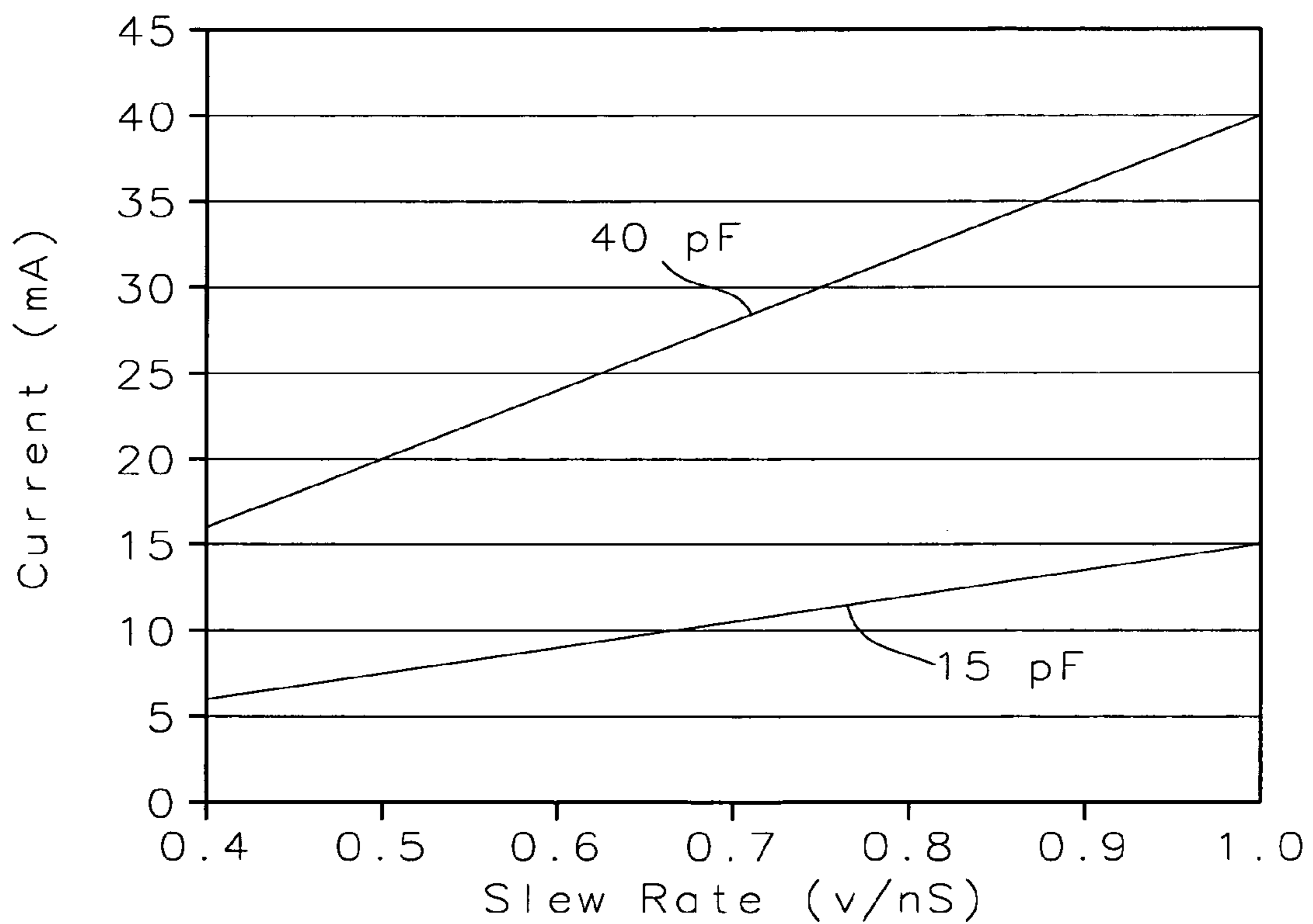
FIG. 5 Prior Art
