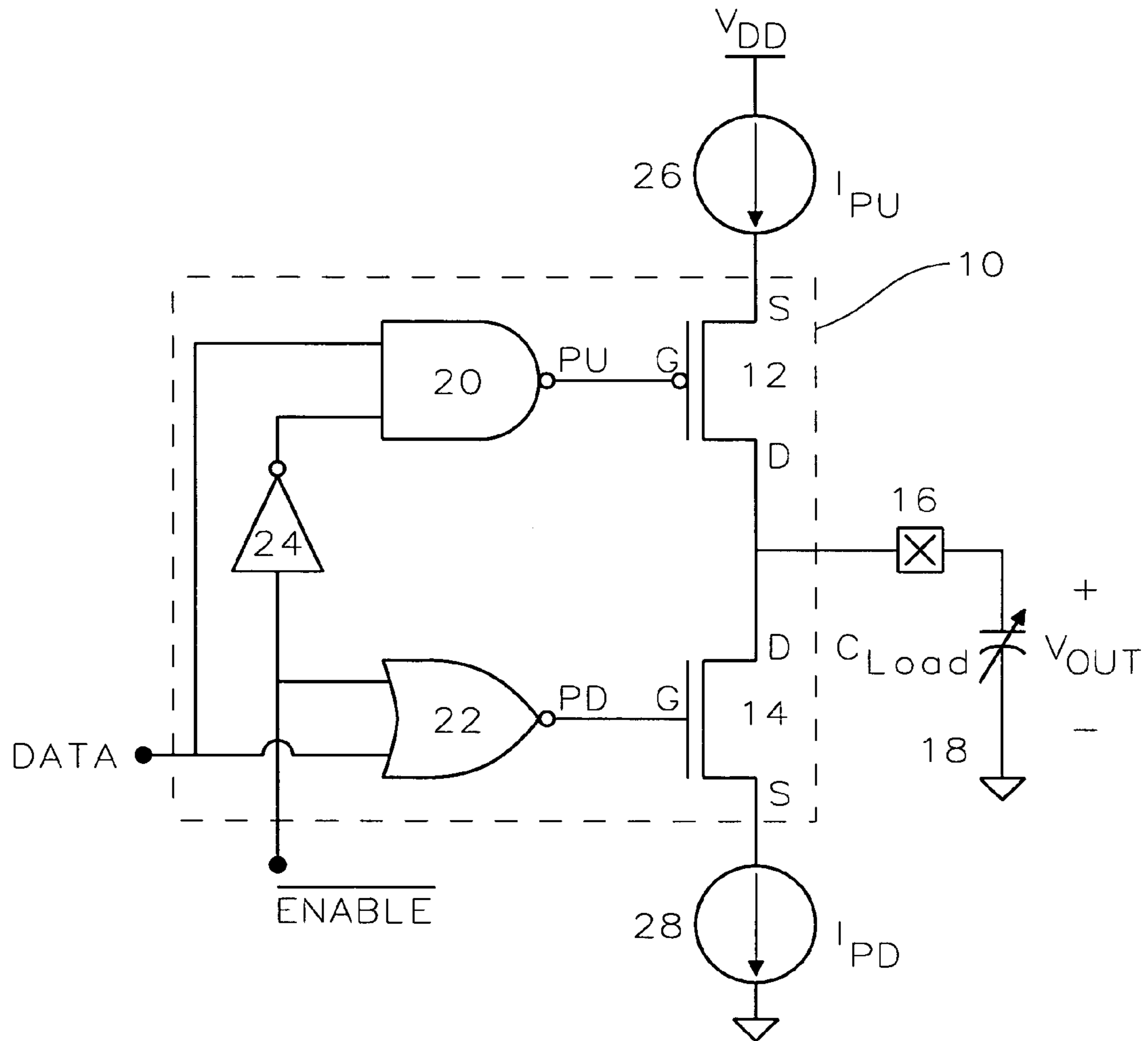
FIG. 3 Prior Art
