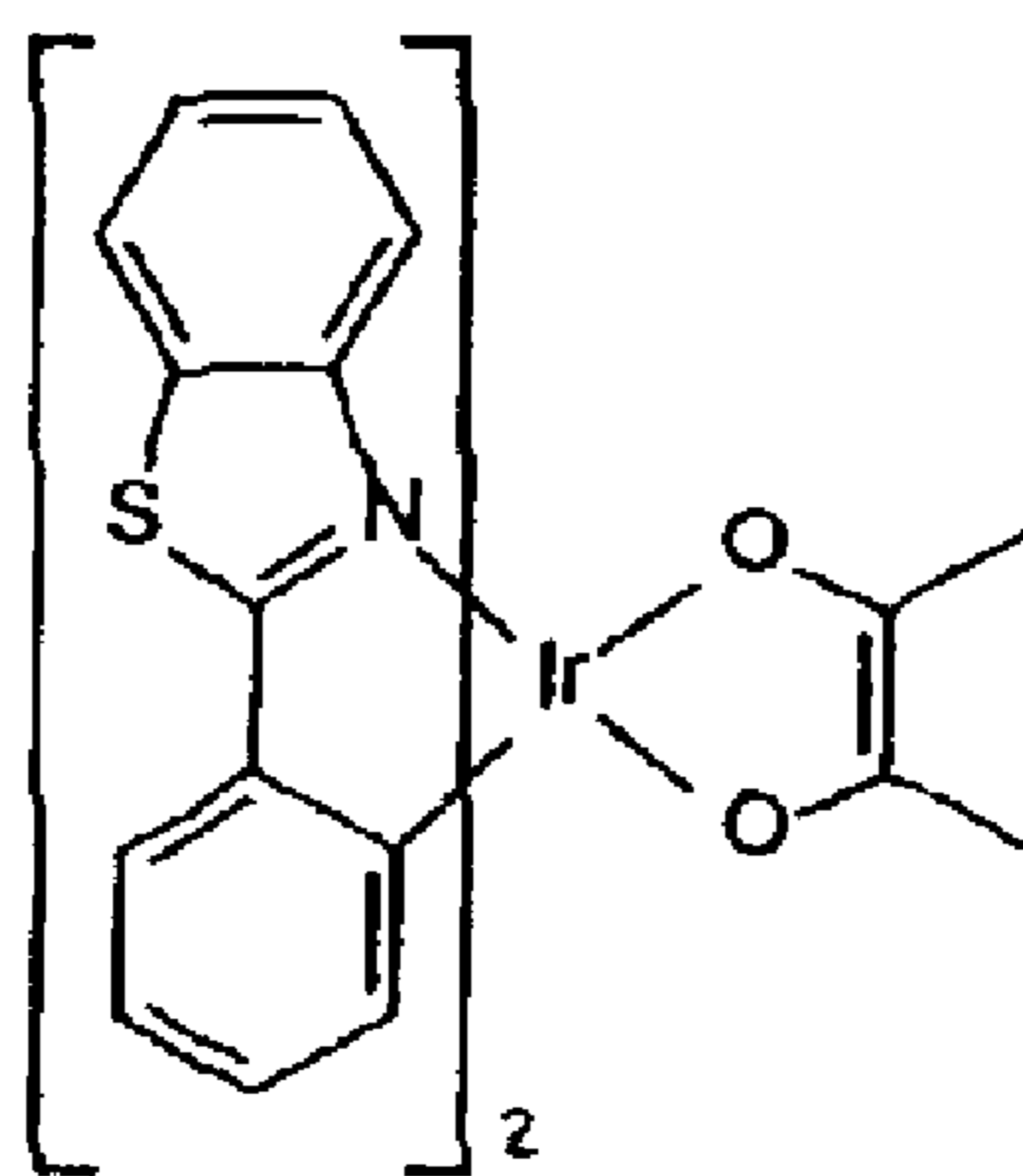
Bt 2 (acac)
