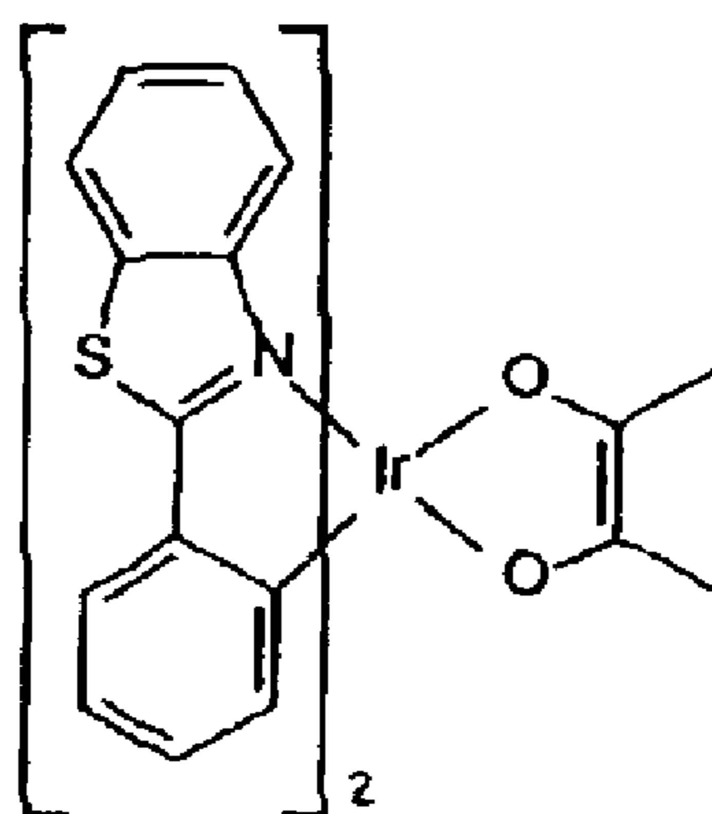
Bt 2 (acac)
