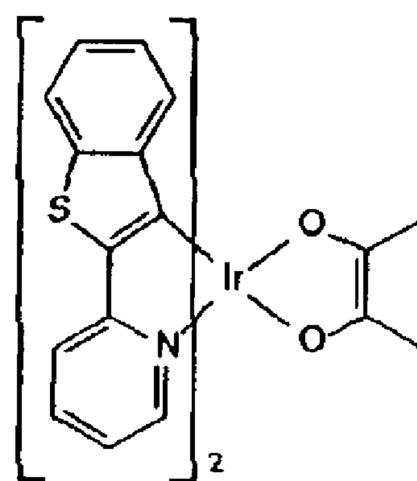
Btp 2 (acac)
