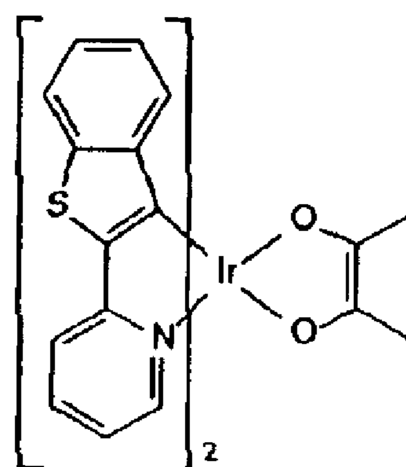
Btp 2 (acac)
