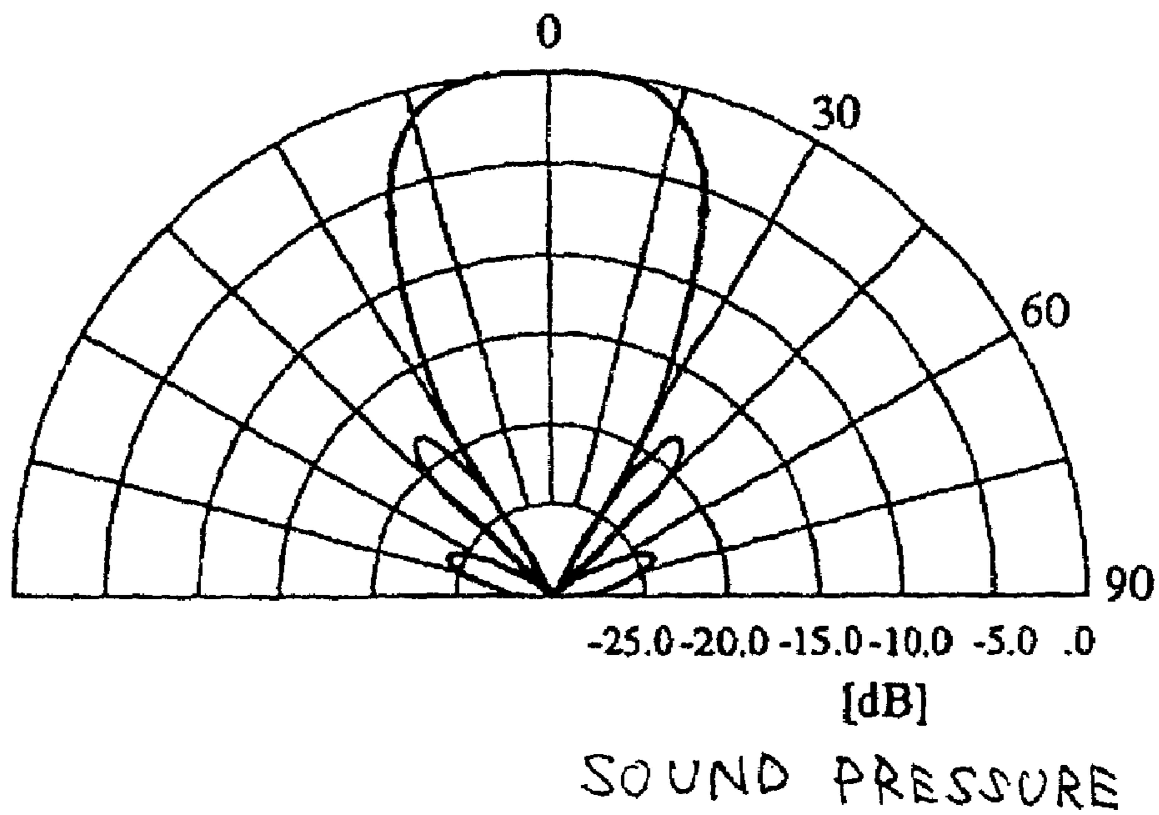
DIRECTIVITY CHARACTERISTICS
