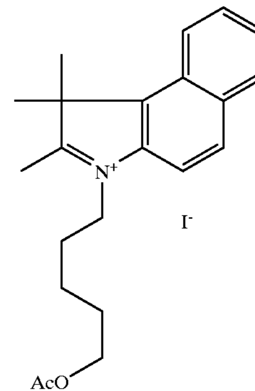
1,1,2-Trimethyl-3-(5-methylcarboxyloxy)pentyl-1H-naphtho[2,1-b]azolium iodide
