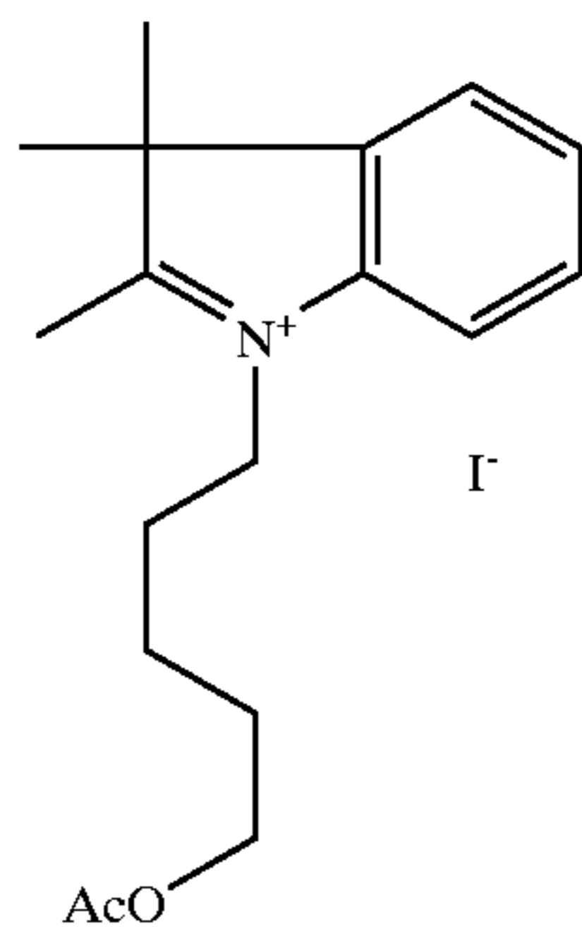
2,3,3-Trimethyl-1-(5-methylcarboxyloxy)pentyl-3H-benzo[b]azolium iodide
