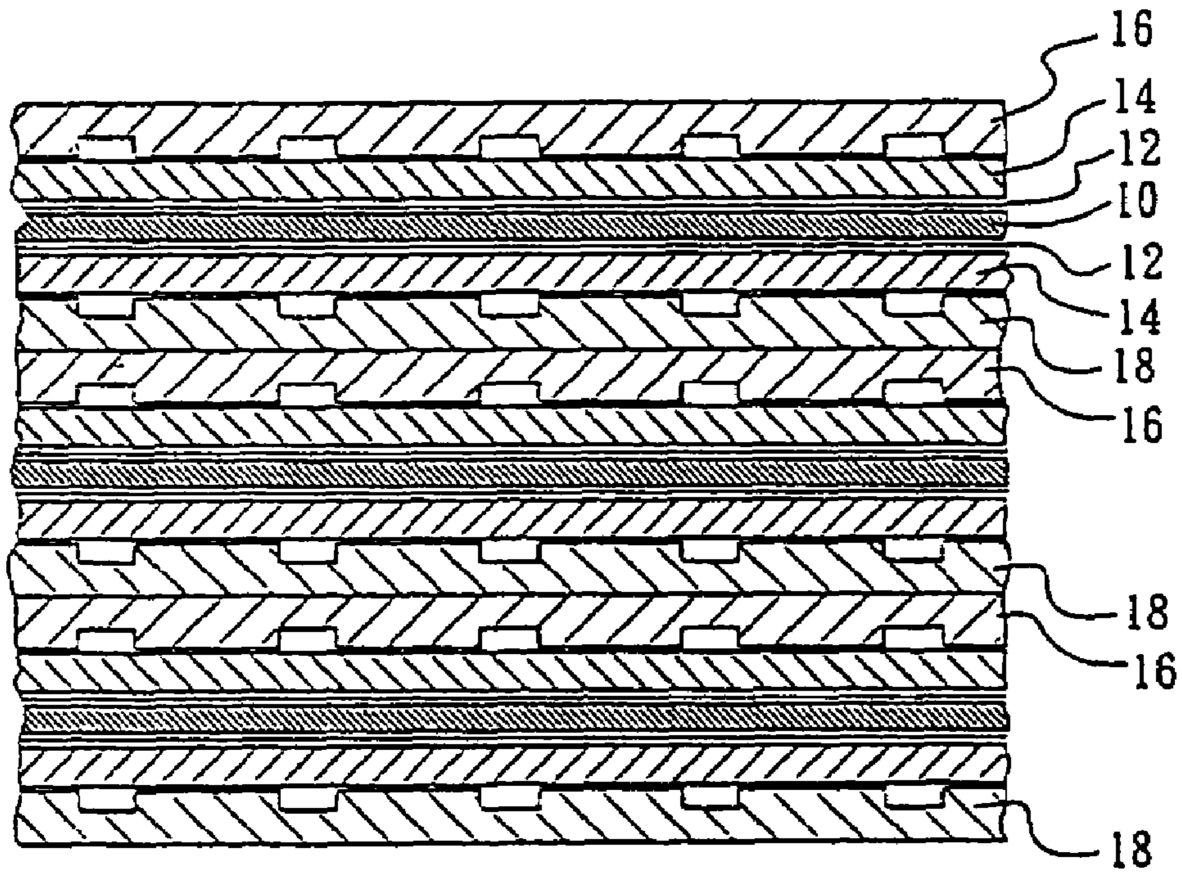
FIG. 2 (PRIOR ART)
