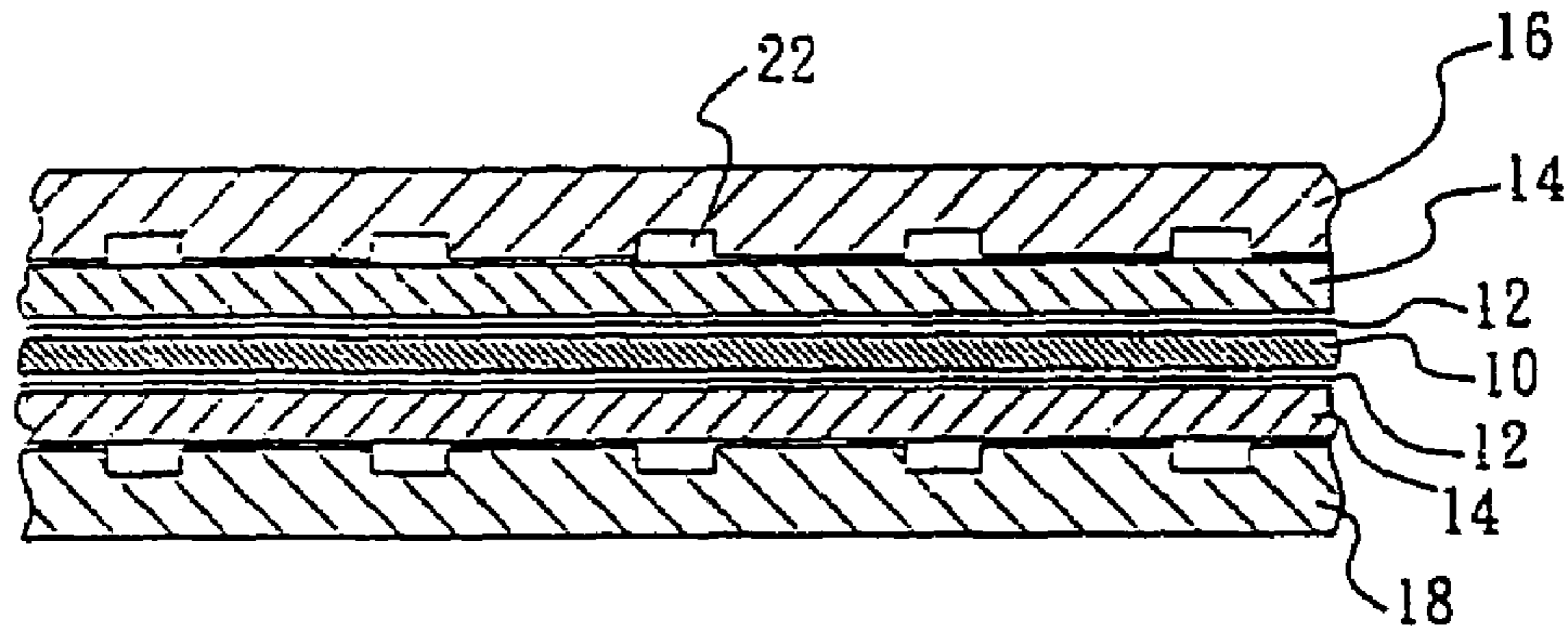
FIG. 1 (PRIOR ART)
