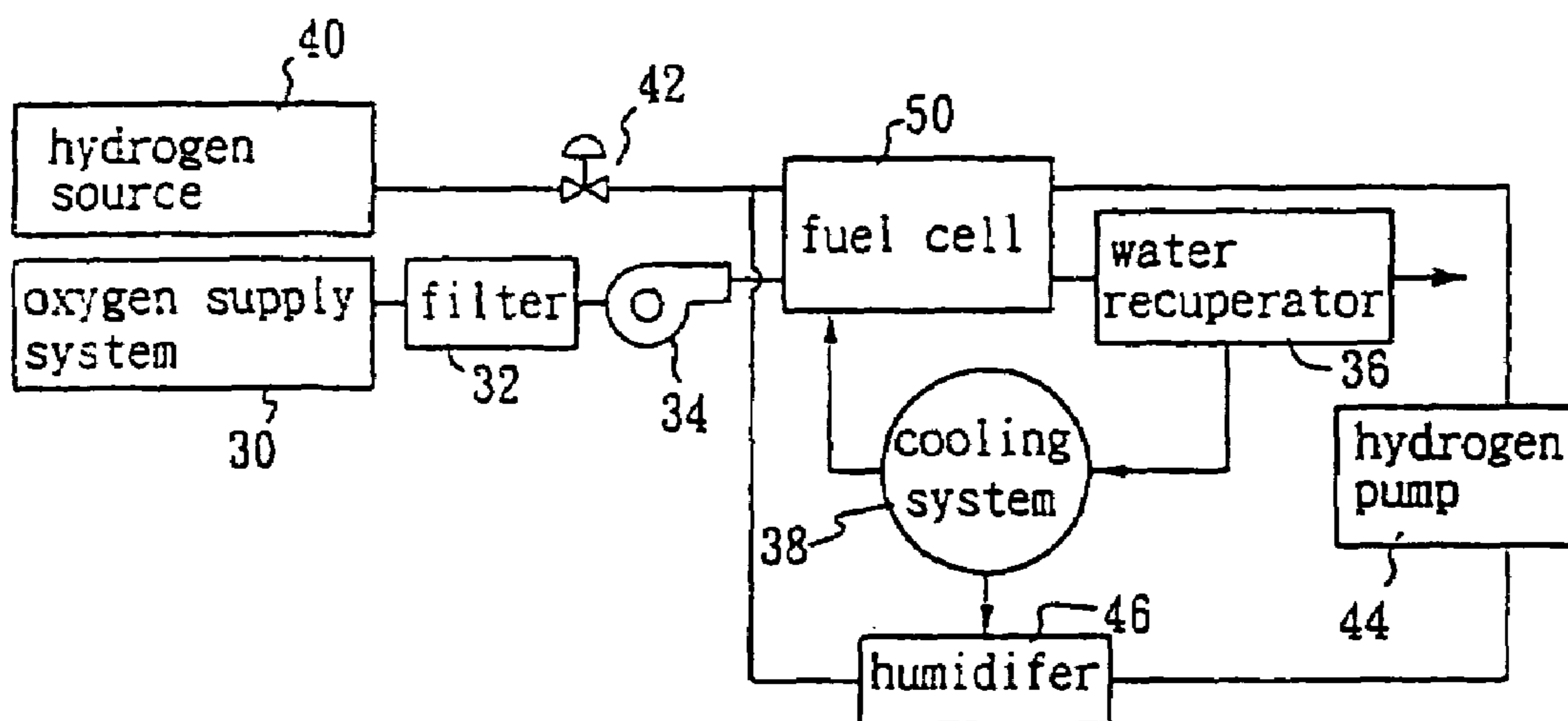
FIG. 4 (PRIOR ART)
