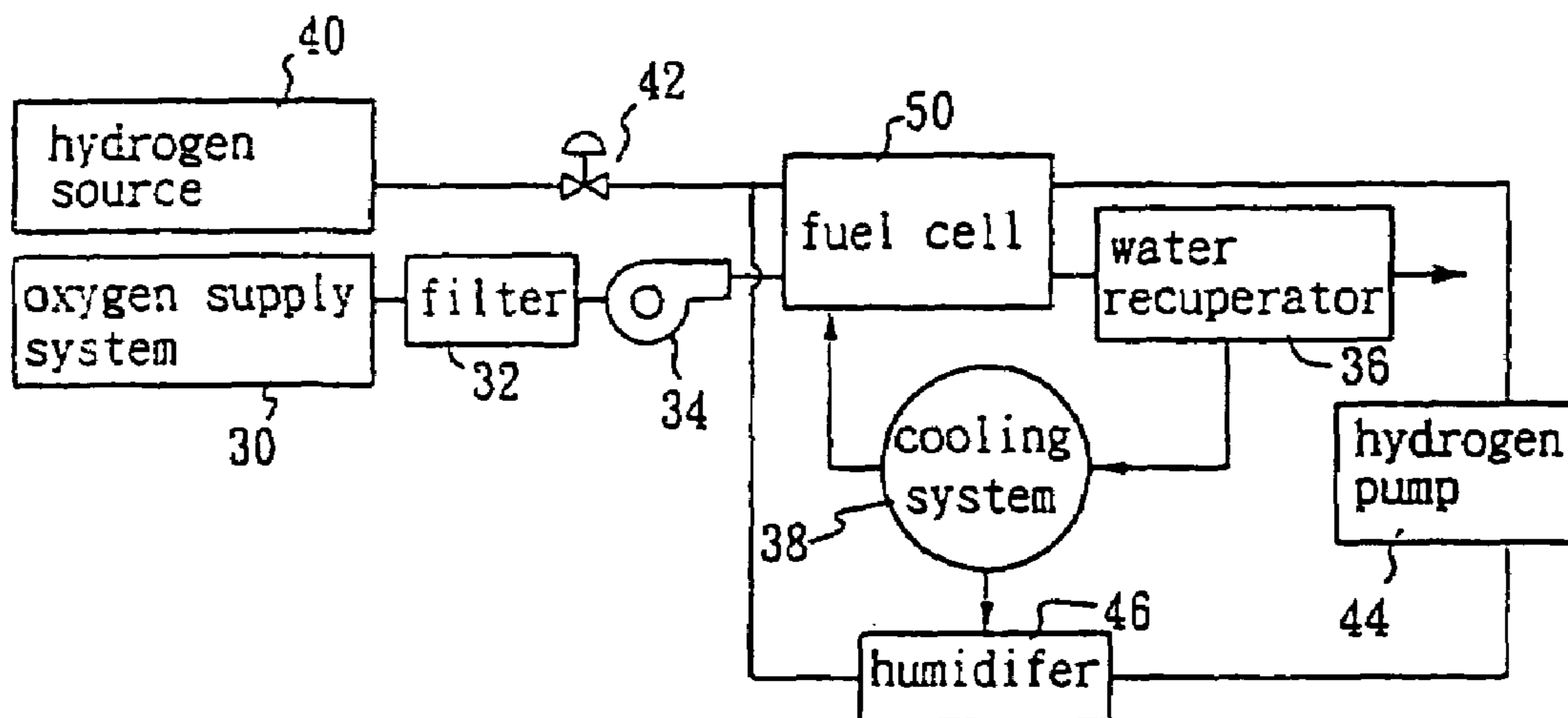
FIG. 4 (PRIOR ART)
