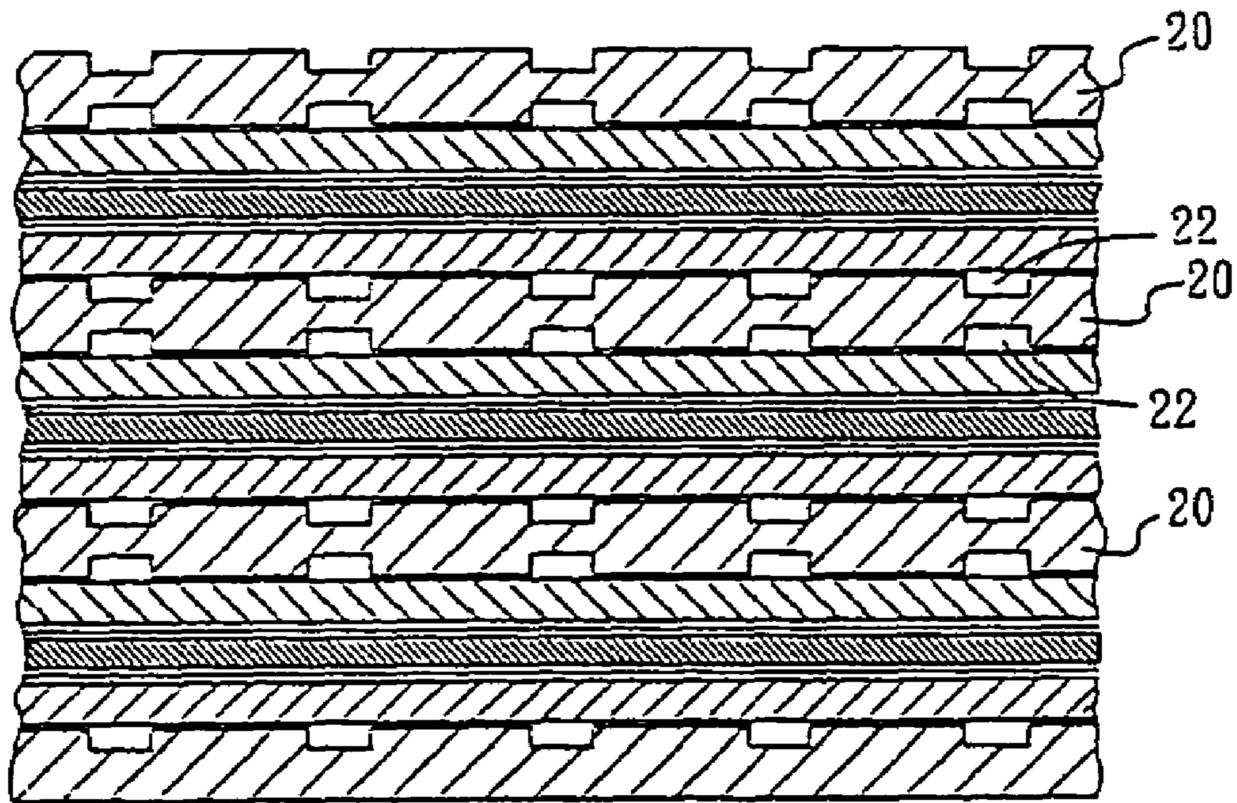
FIG. 3 (PRIOR ART)
