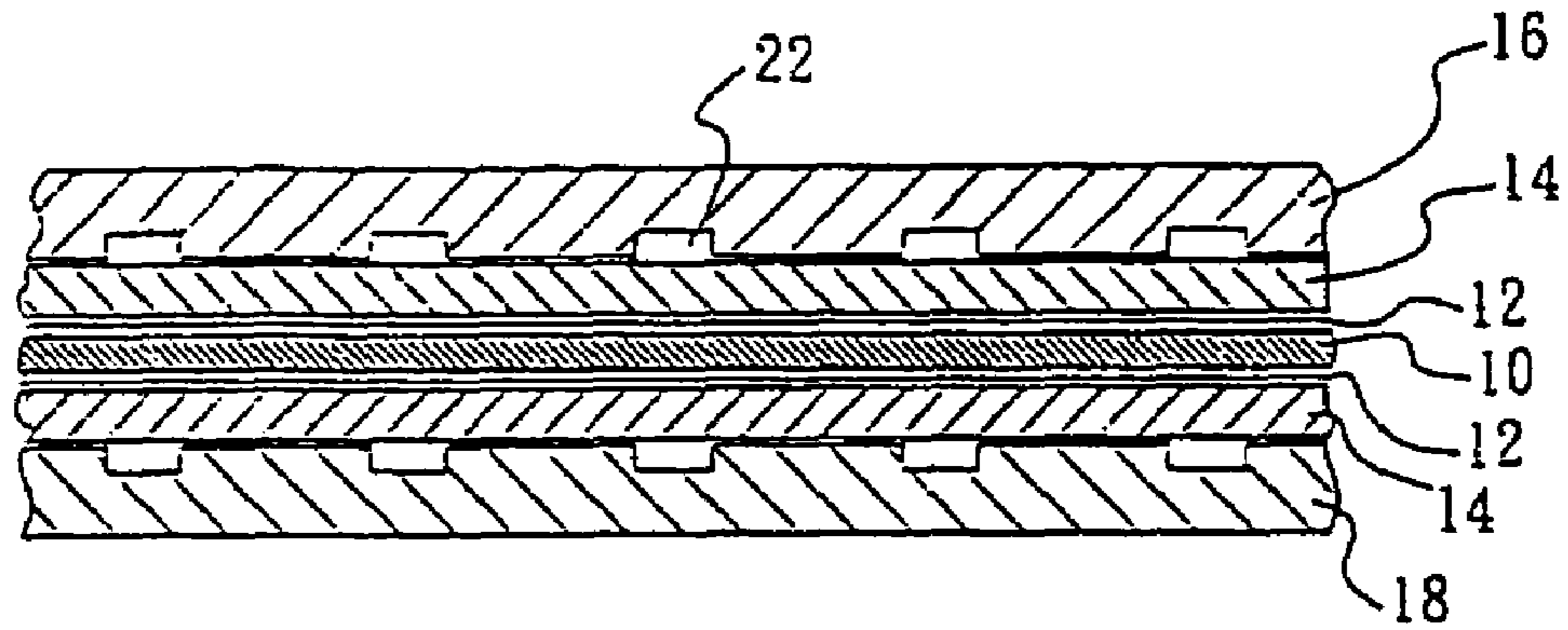
FIG. 1 (PRIOR ART)
