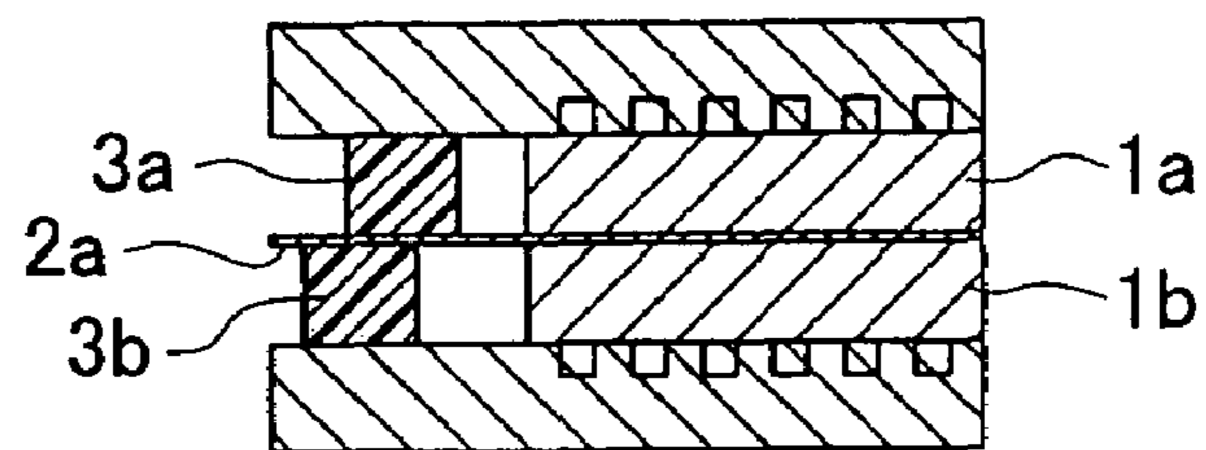
FIG. 19 (Prior Art)
