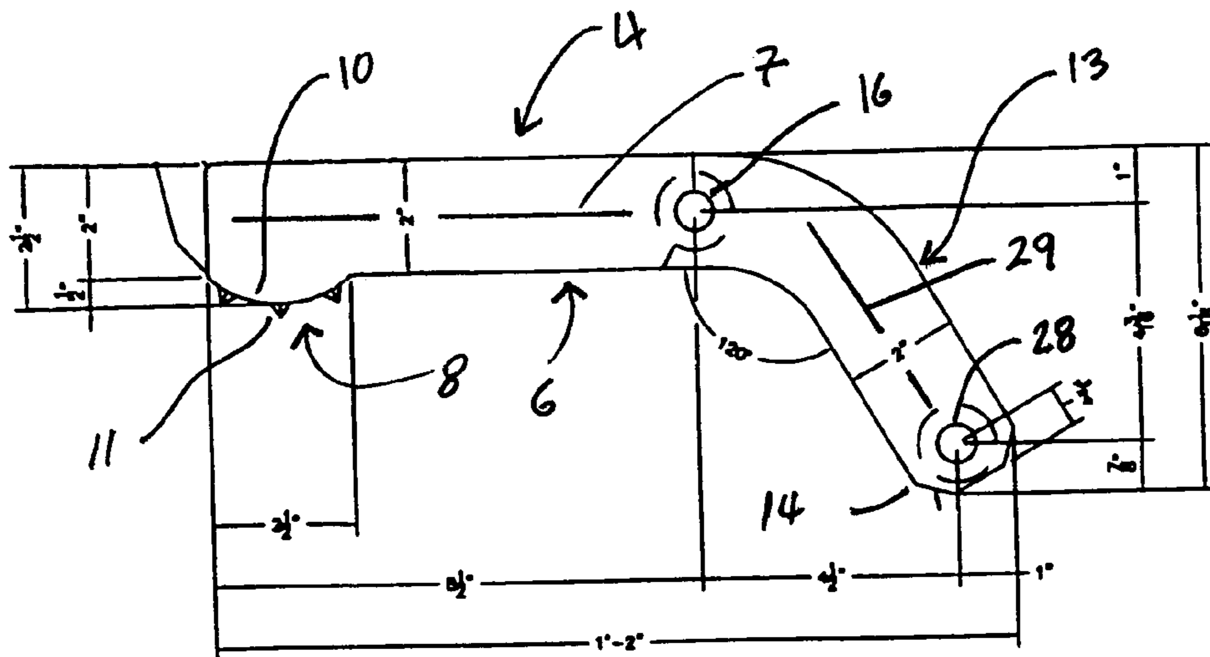
PART "A" Half Scale (2 Required)
