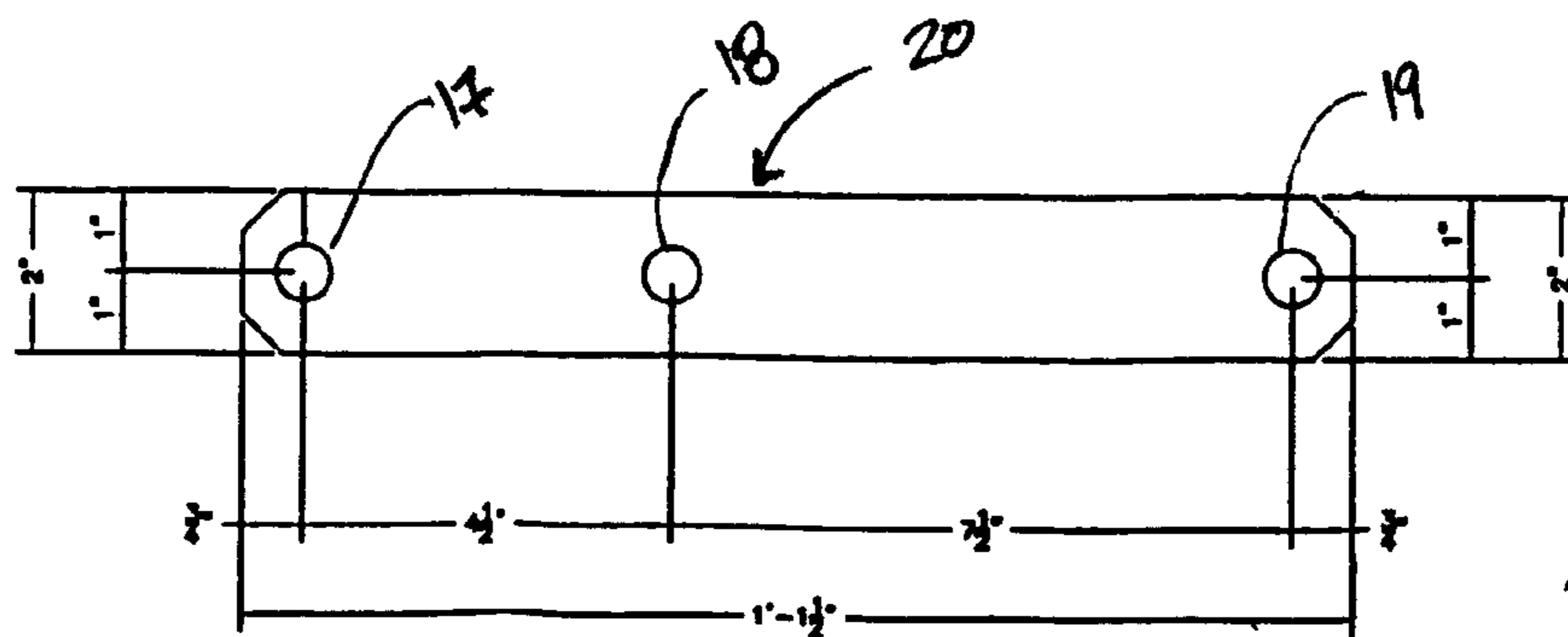
PART "B" Half Scale (2 Required)
