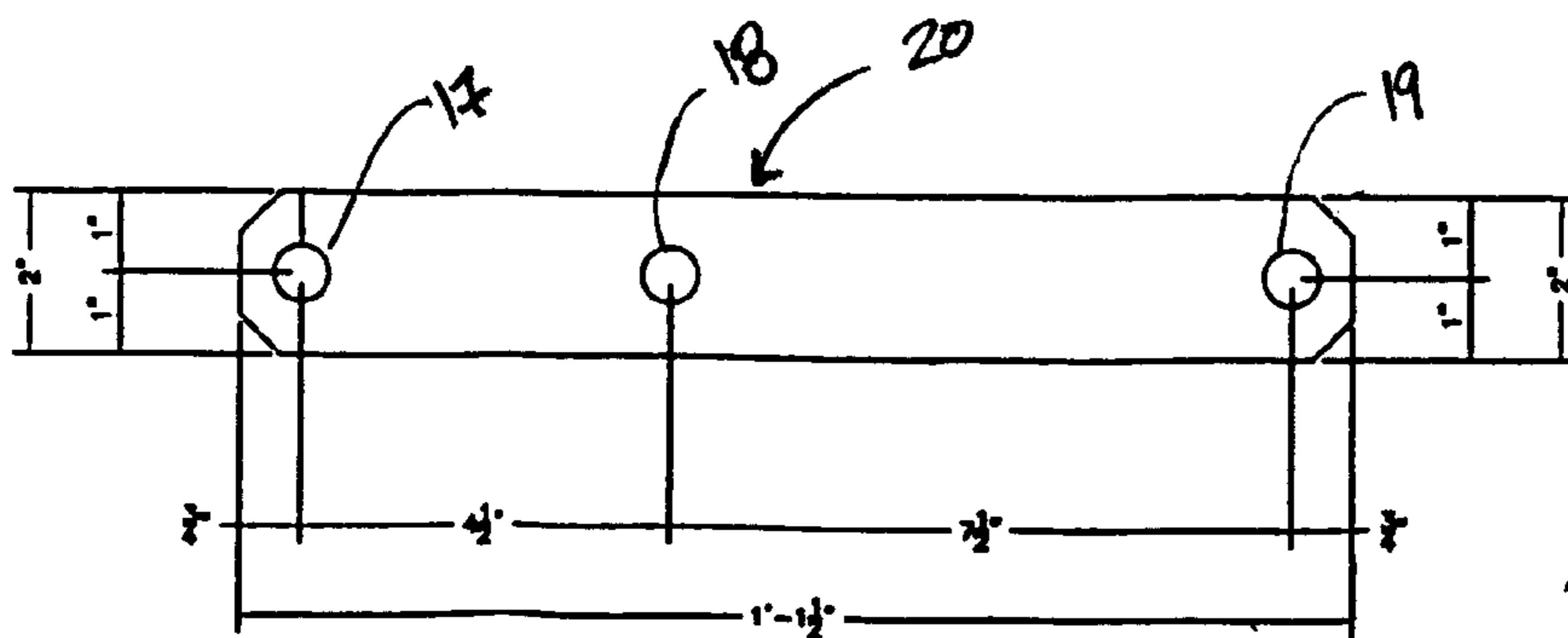
PART "B" Half Scale (2 Required)
