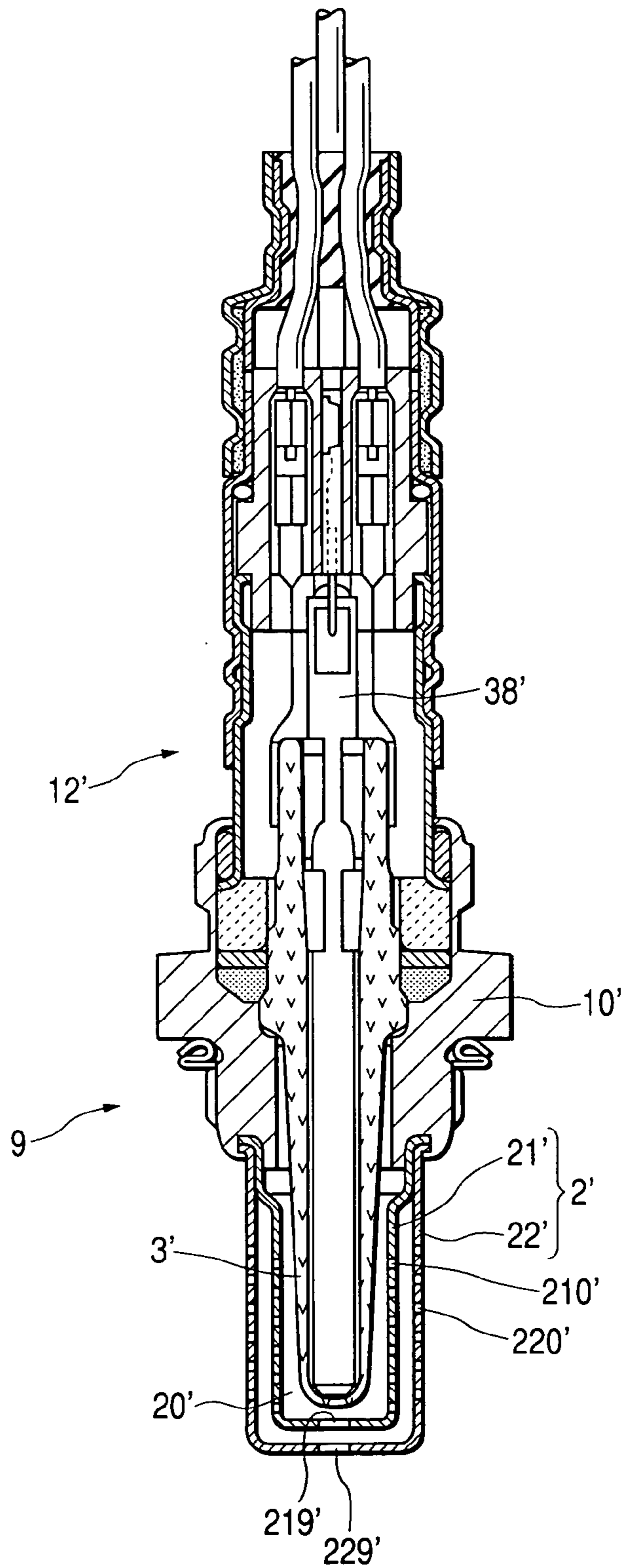
FIG. 25 (PRIOR ART)
