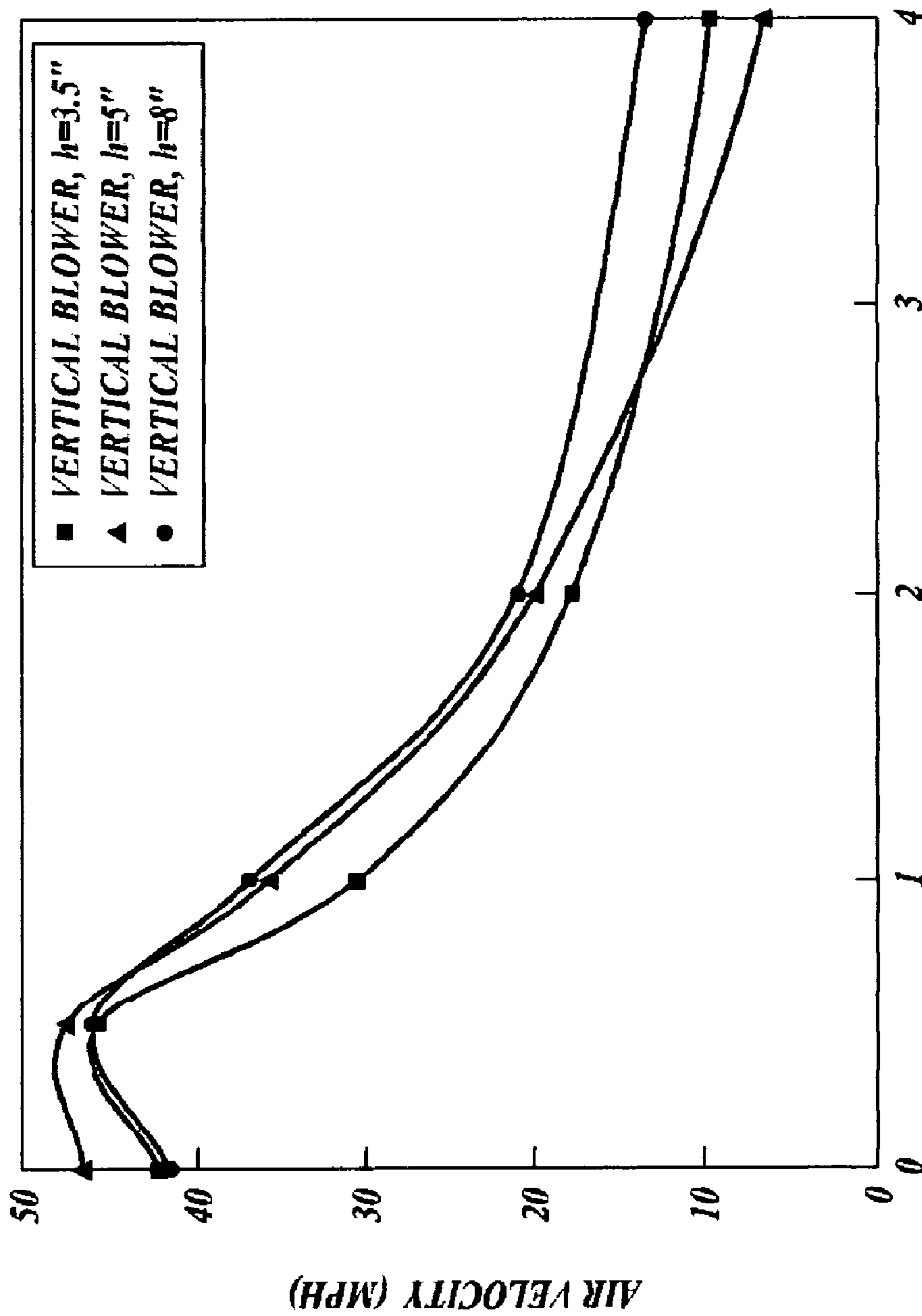
DISTANCE FROM BLOWER LIP (ALONG "X-AXIS", REF. FIG. 5), FT.
