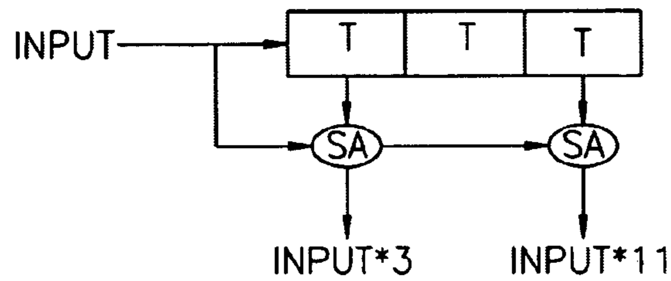
REALIZATION OF COEFFICIENT USING SHARE-ABLE MULTIPLIER (COEFF.=3.11)
