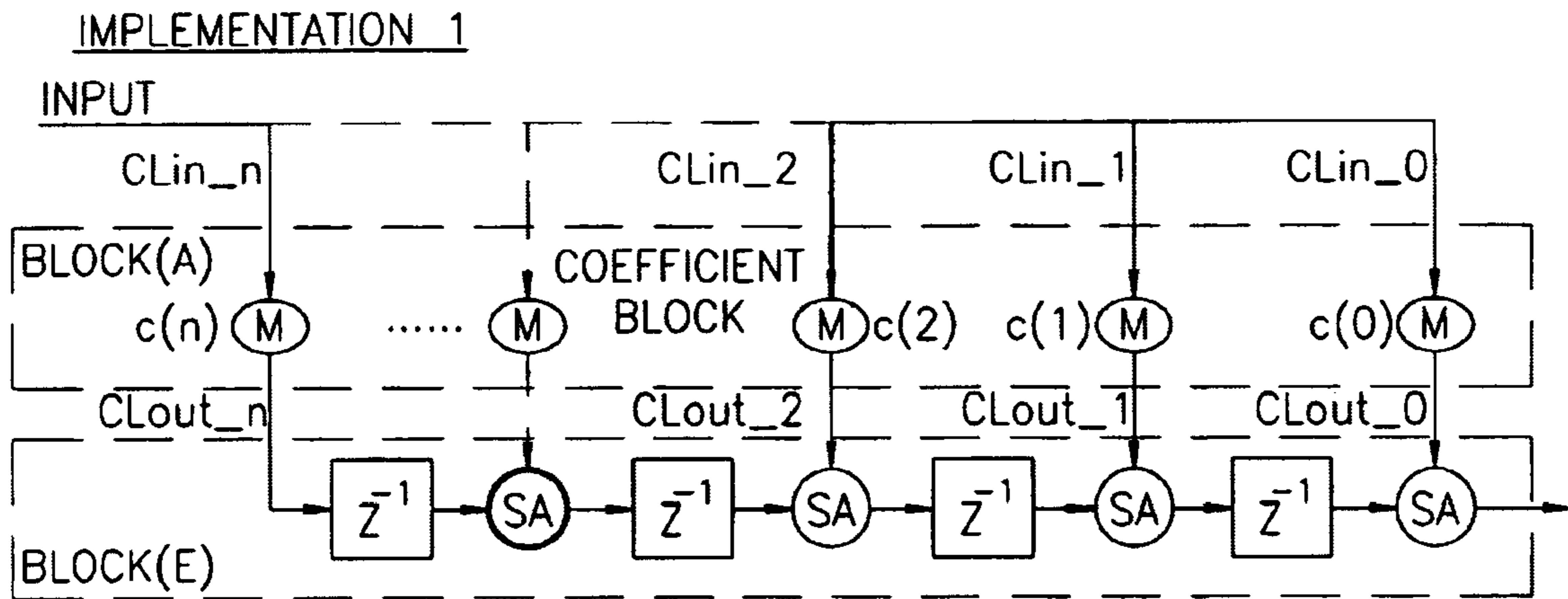
REALIZATION OF COEFFICIENT USING SHARE-ABLE MULTIPLIER (COEFF.=3.11)
