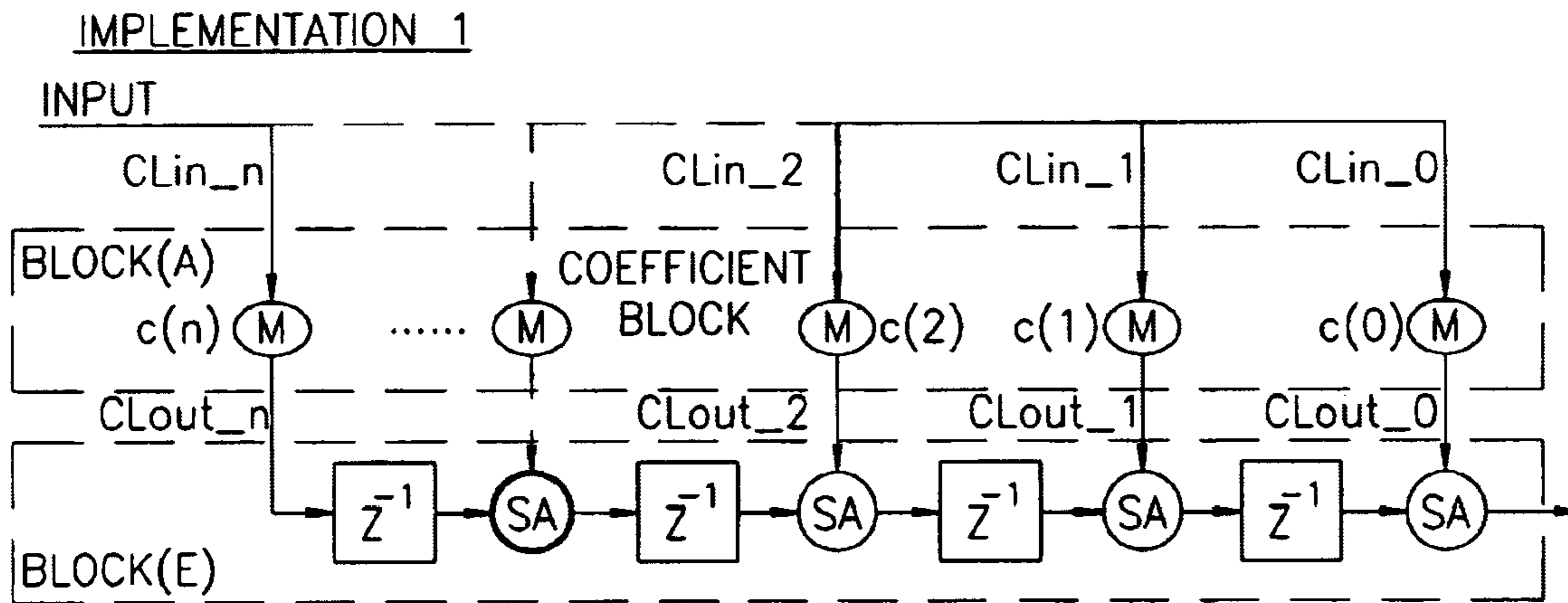
REALIZATION OF COEFFICIENT USING SHARE-ABLE MULTIPLIER (COEFF.=3.11)
