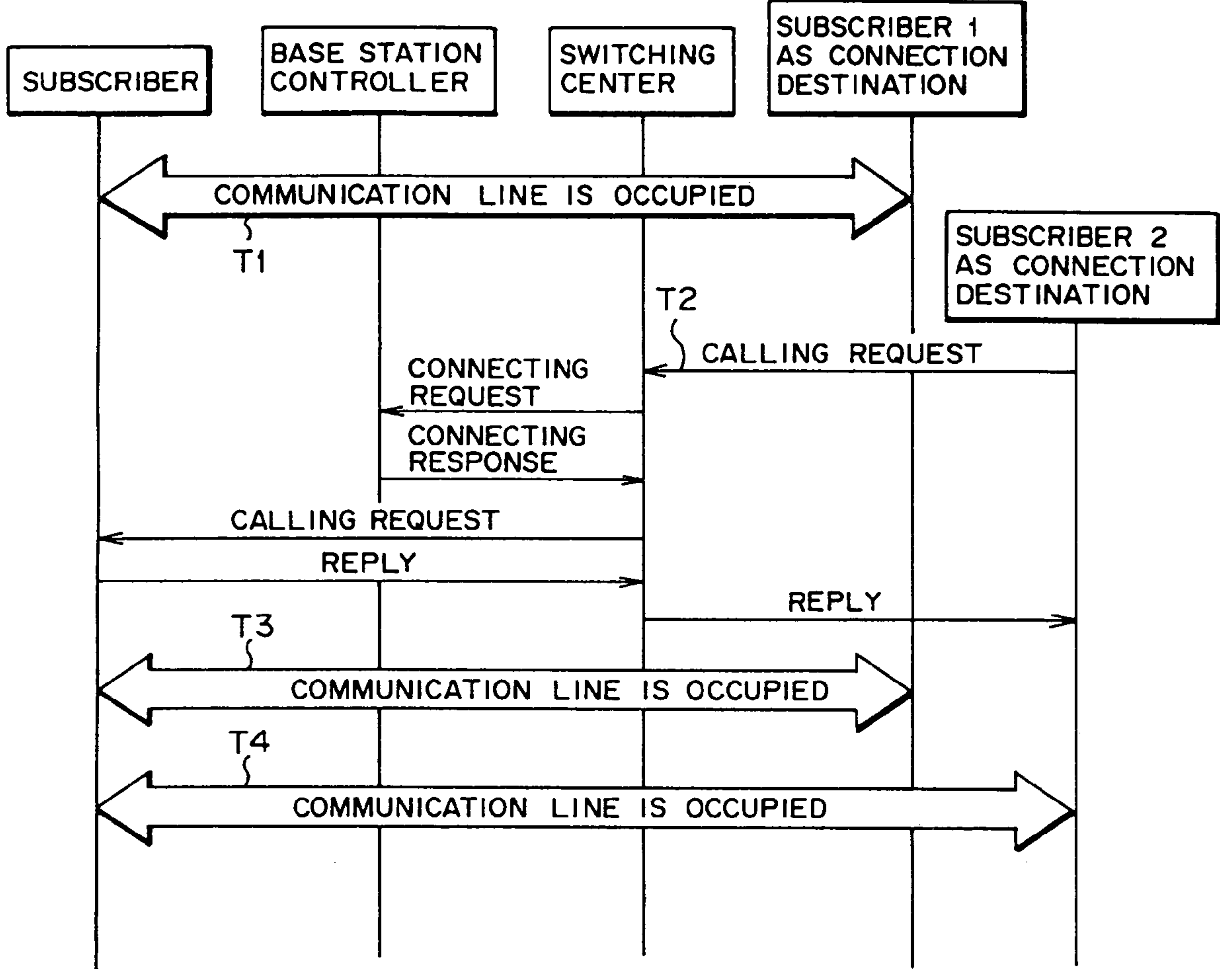
EXAMPLE OF CONNECTION SEQUENCE OF MULTI-SESSION (MULTICALL)
