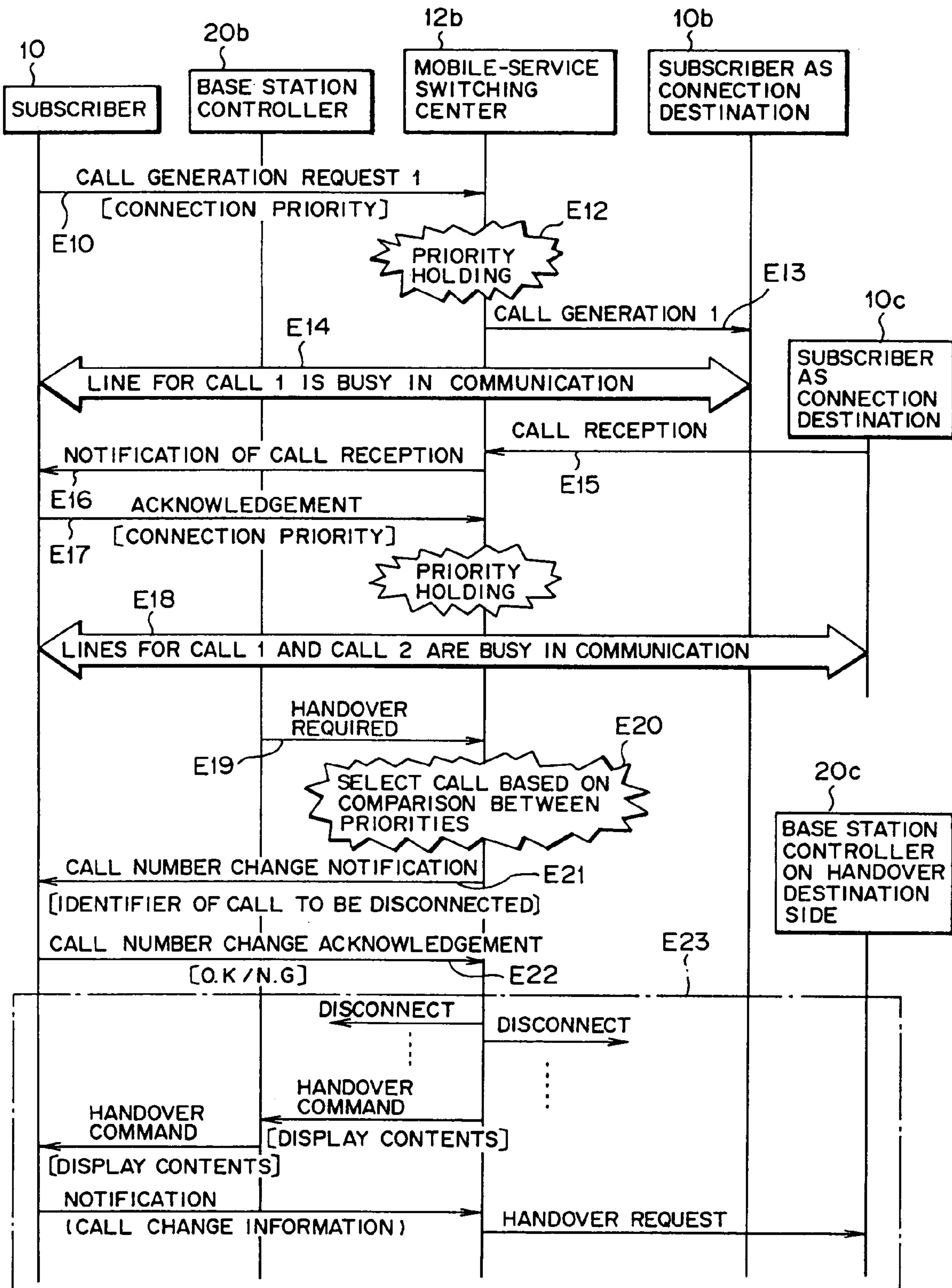
EXAMPLE OF SIGNALING SEQUENCE
