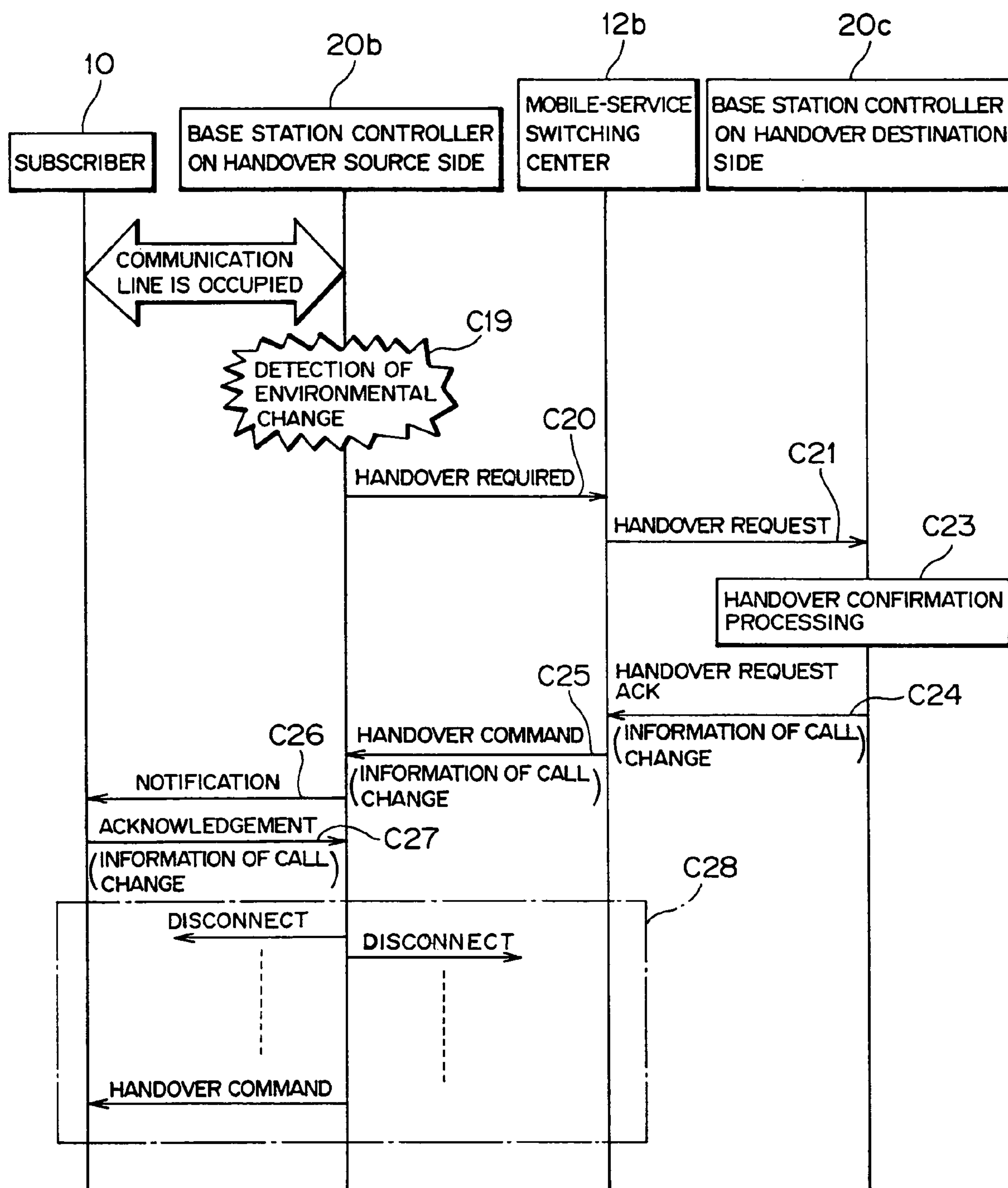
EXAMPLE OF SIGNALING SEQUENCE
