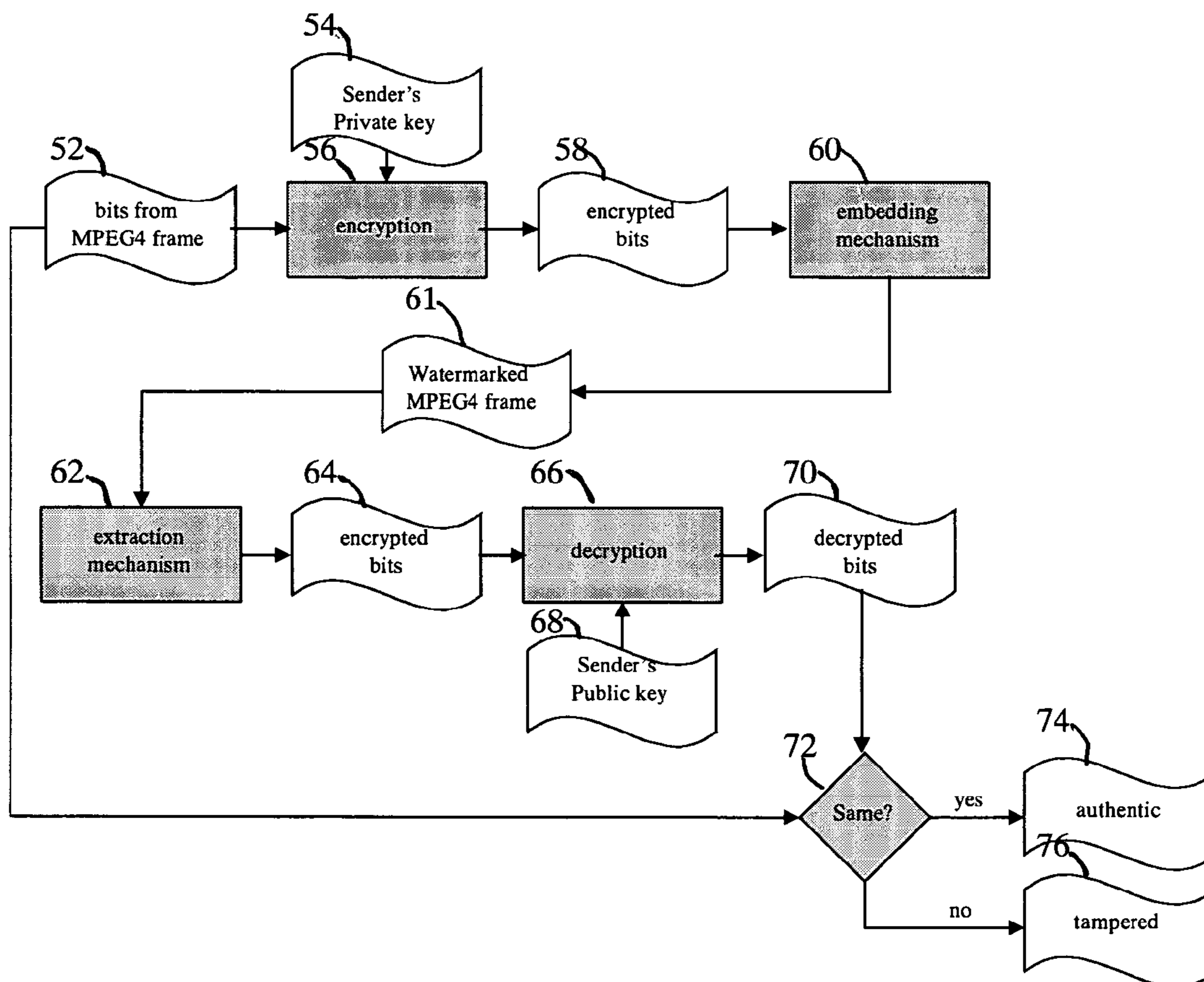
FIG - 1 Method of Embedding Data for Authentication Purposes
