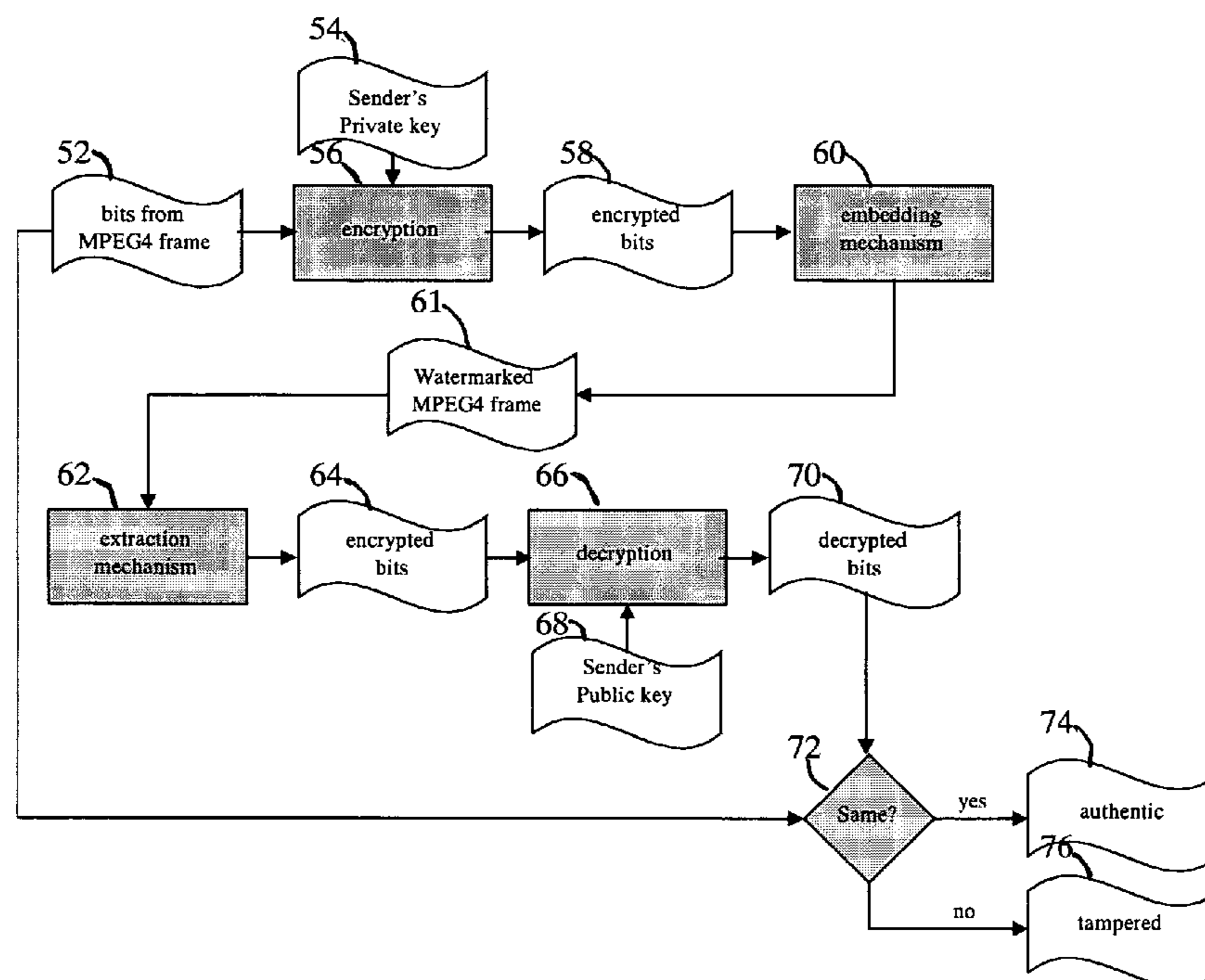
Method of Embedding Data for Authentication Purposes
