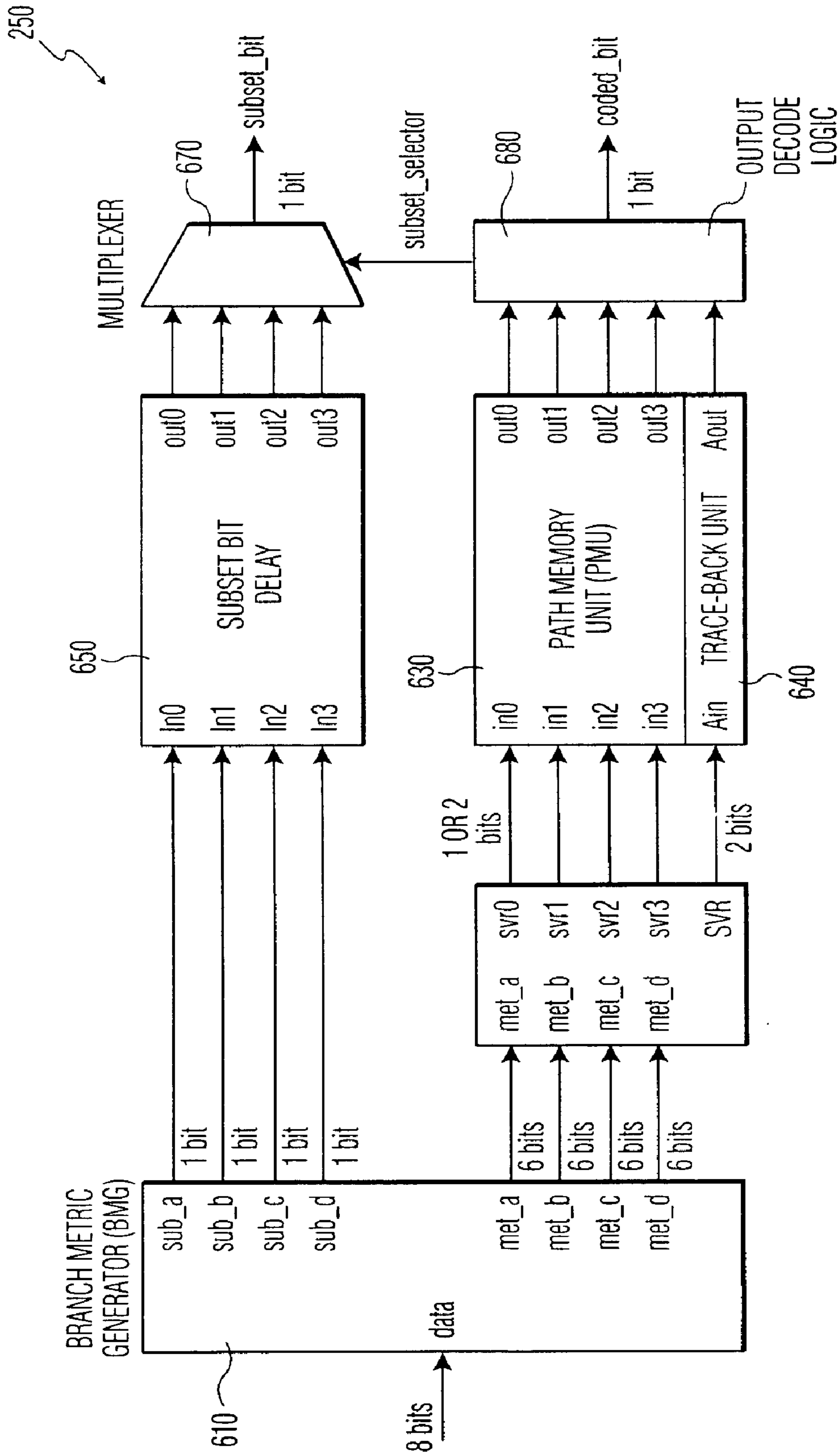
FIG. 6 PRIOR ART
