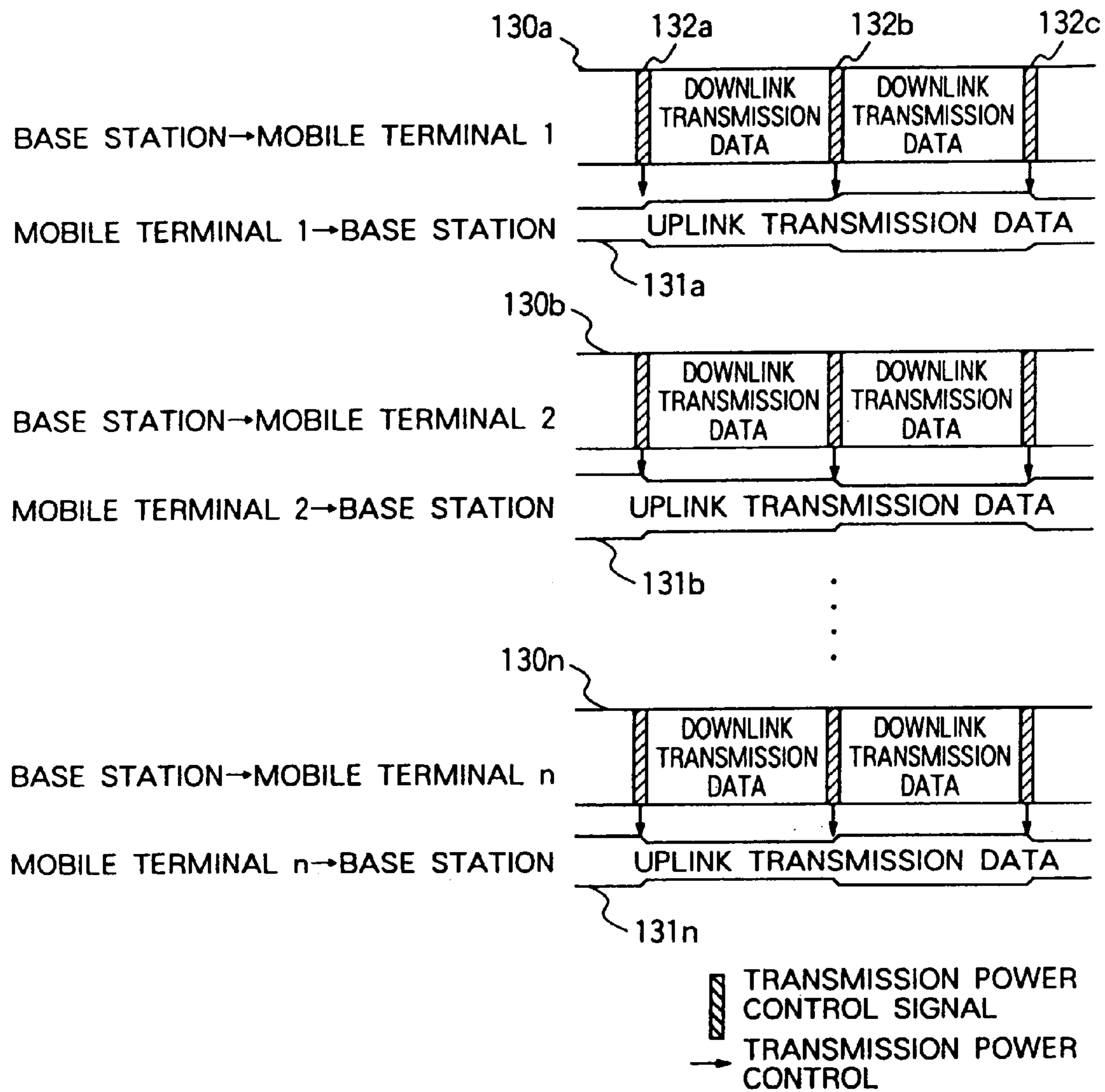
FIG. 12 PRIOR ART
