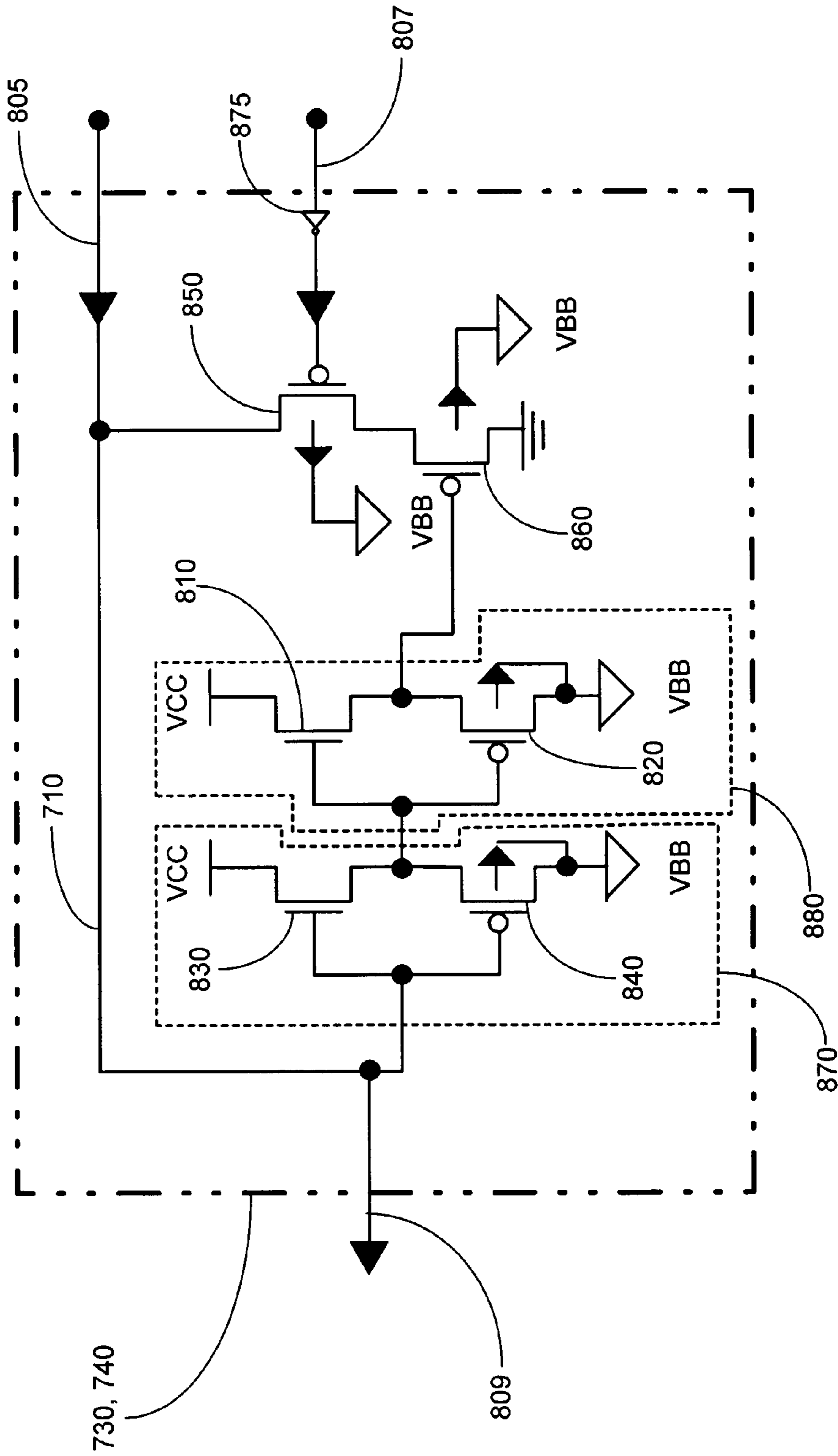
N-Channel Implementation of the One-Shot
