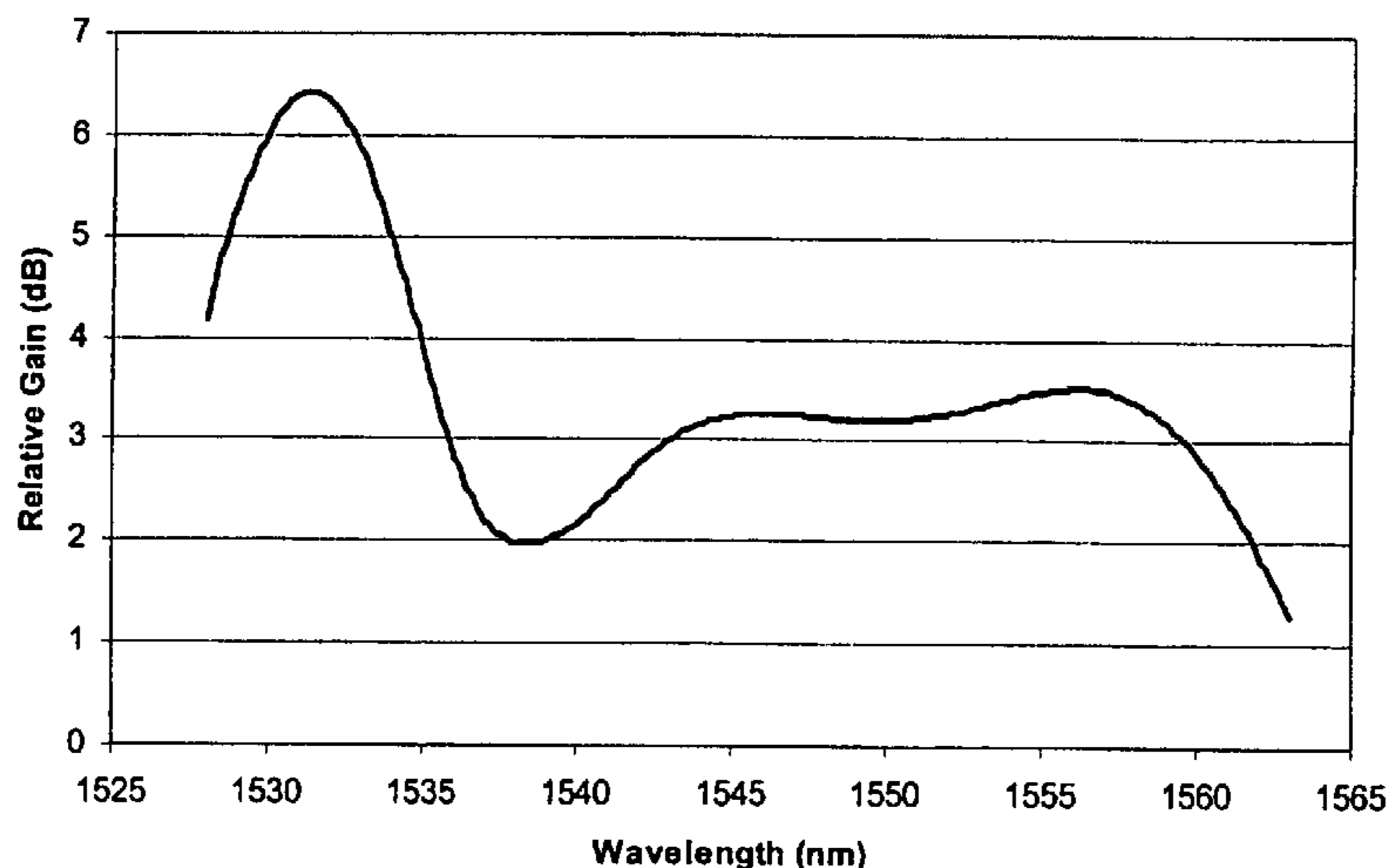
Gain Spectrum of a typical EDFA
