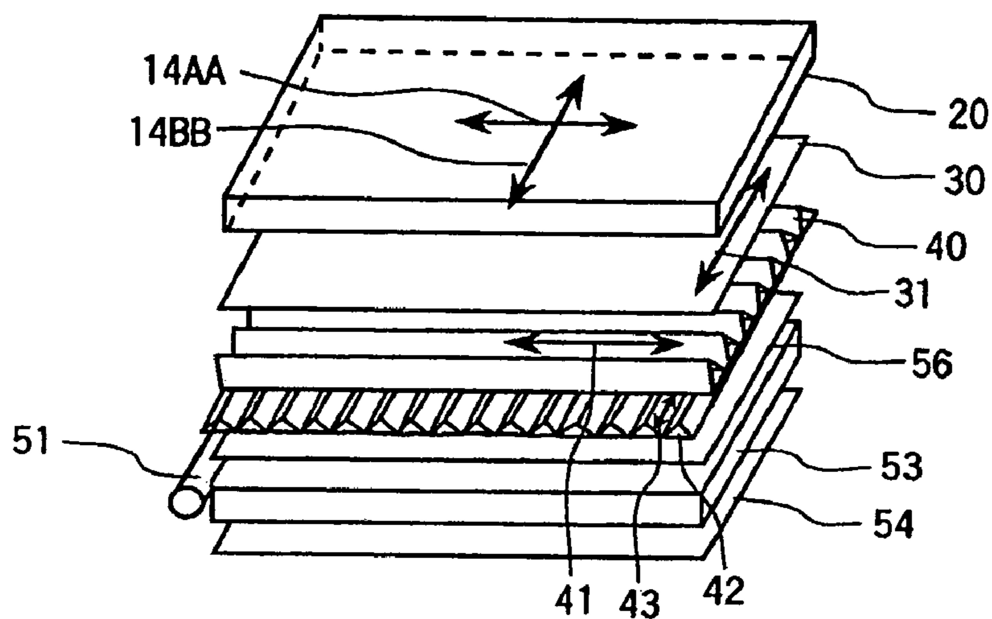
FIG.36 (PRIOR ART)
