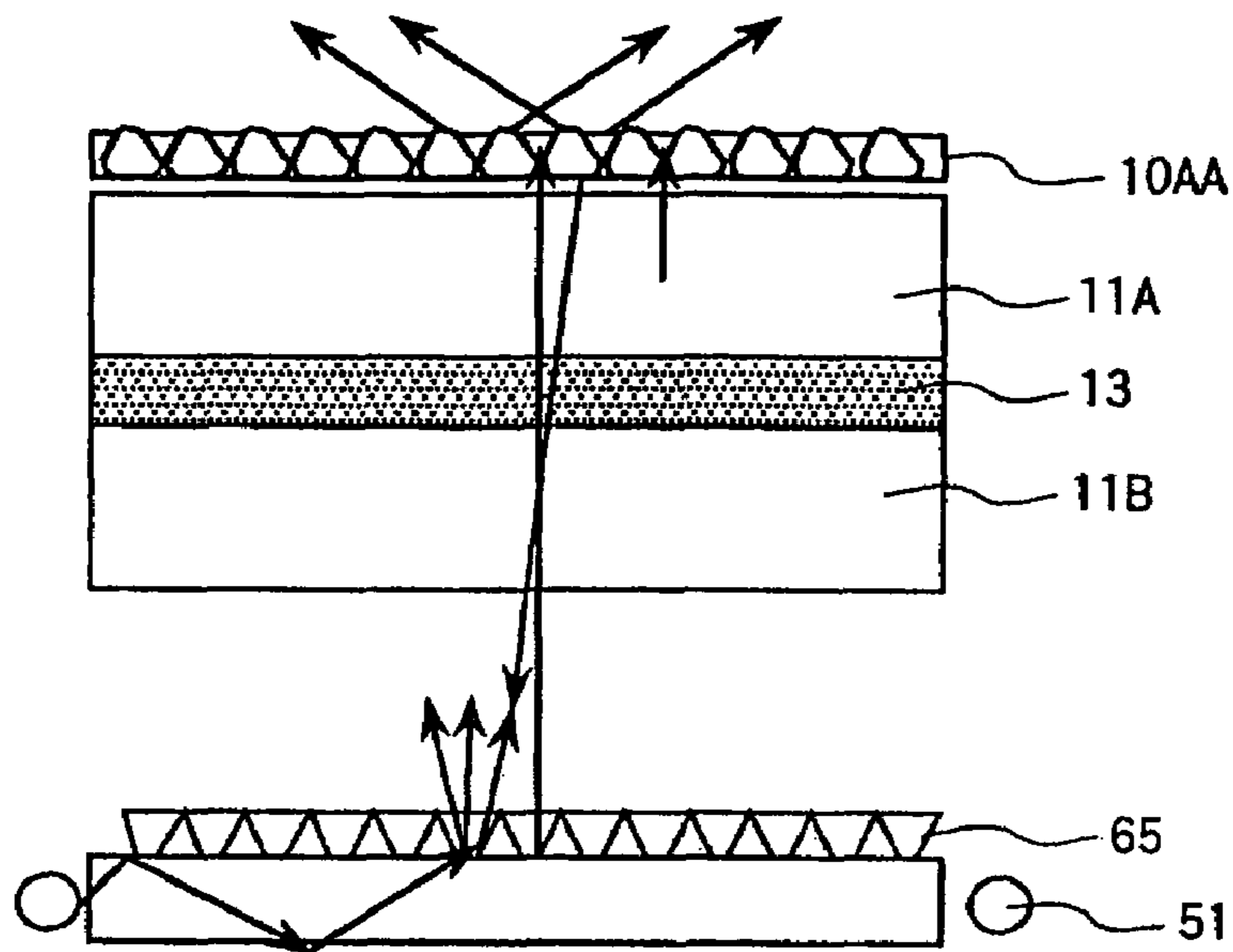
FIG.32 (PRIOR ART)
