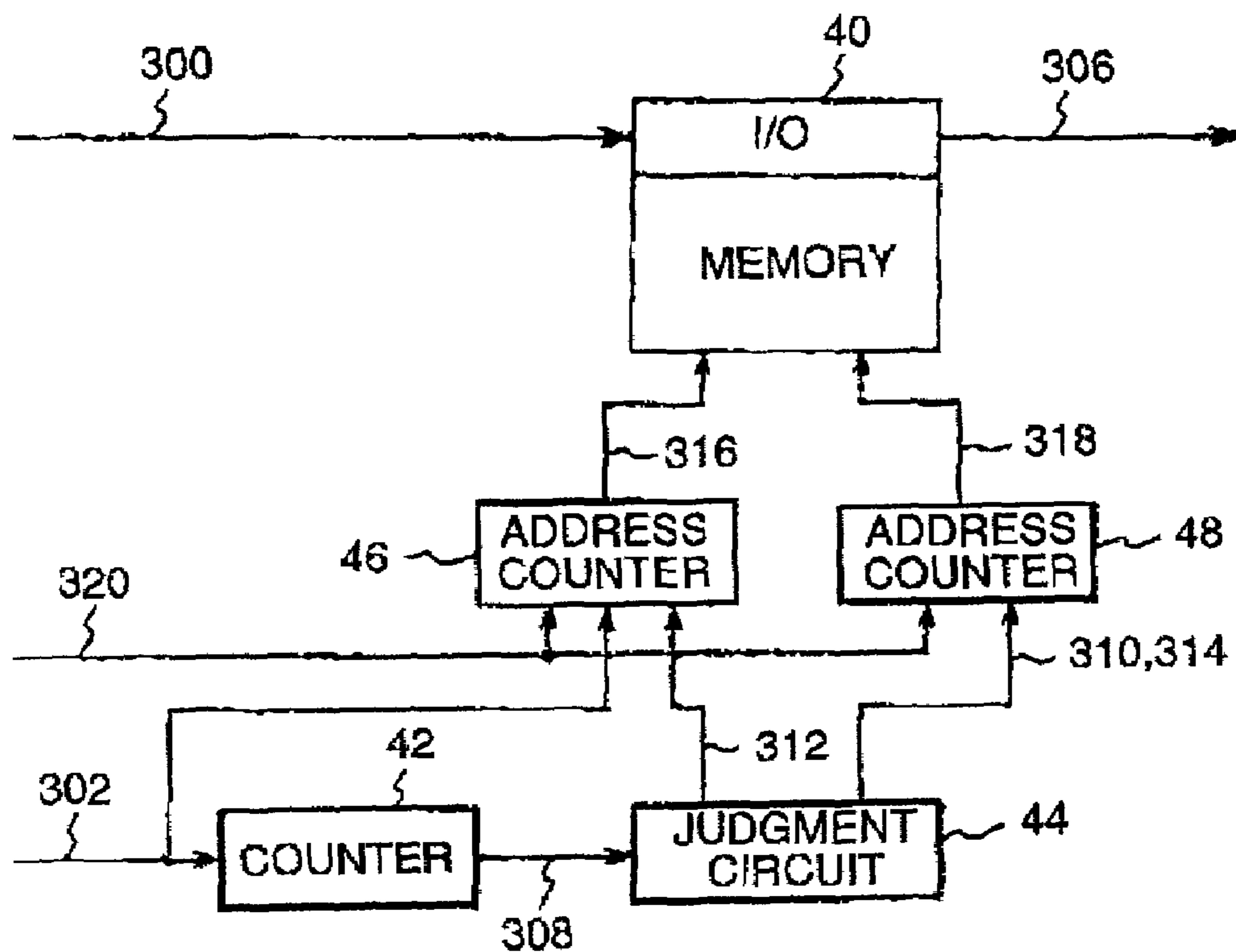
VIDEO SIGNAL CONTROL CIRCUIT OF THE THIRD EMBODIMENT
