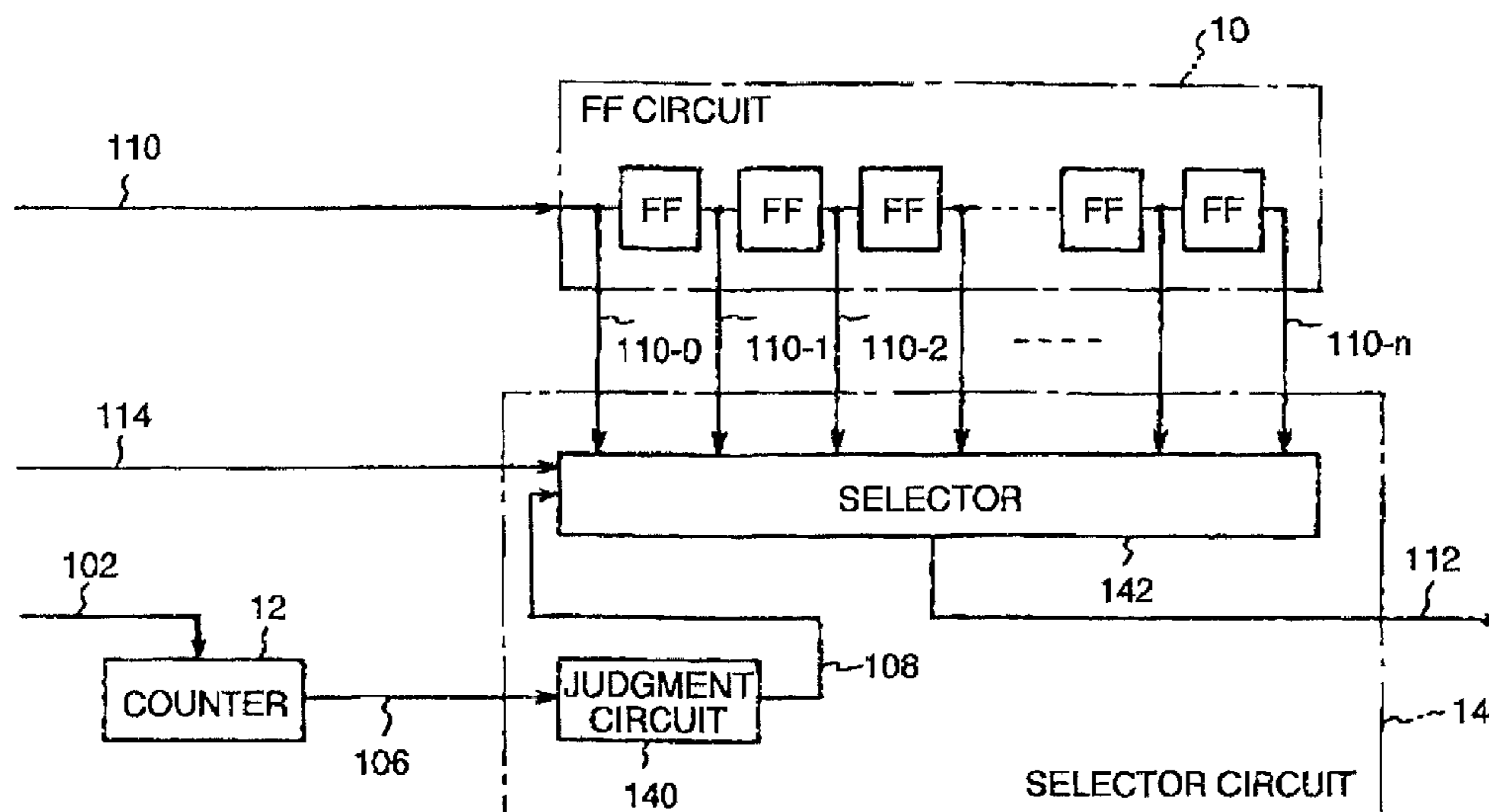
VIDEO SIGNAL CONTROL CIRCUIT OF THE FIRST EMBODIMENT
