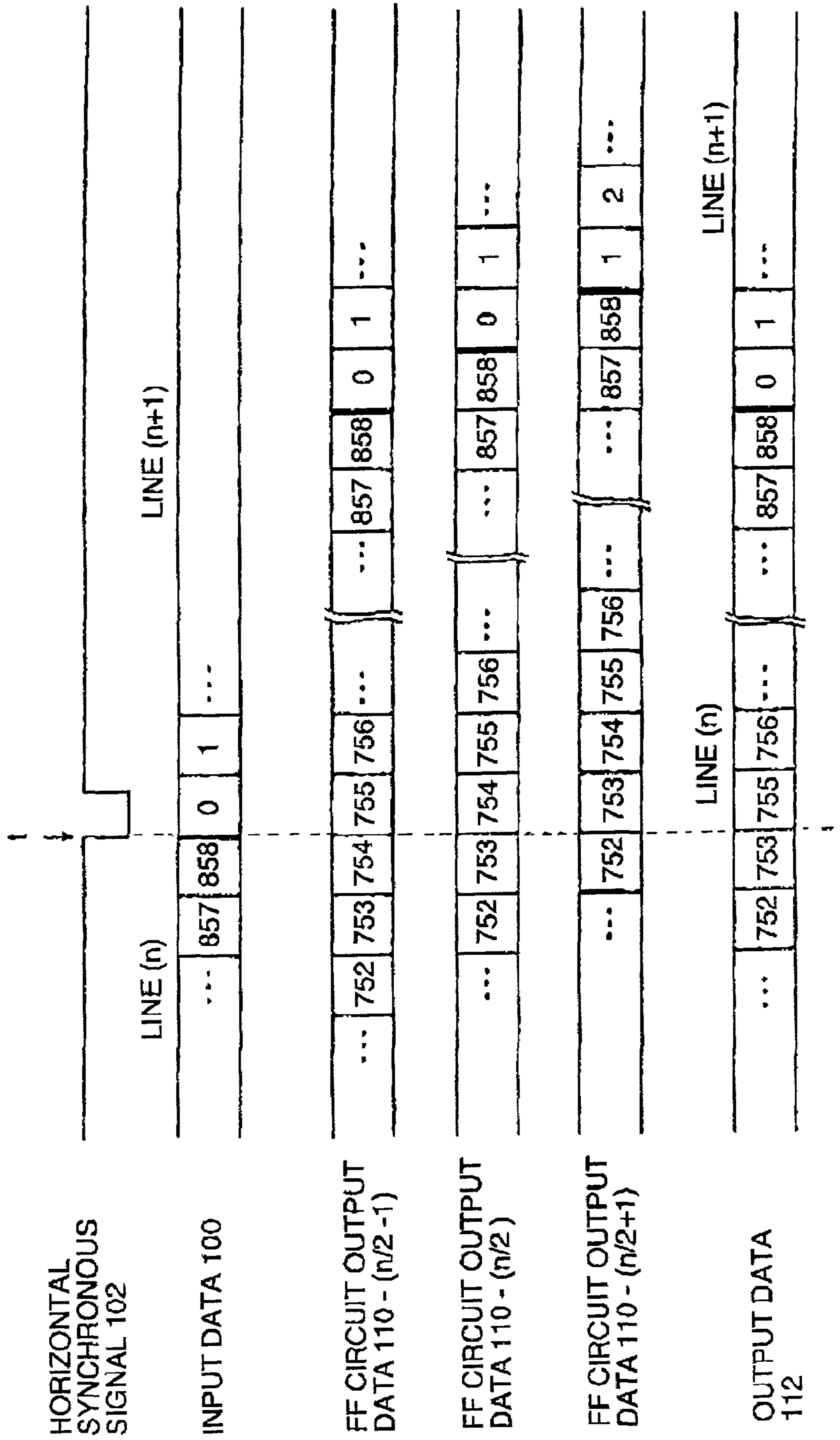
TIMING CHART (2) OF THE FIRST EMBODIMENT
