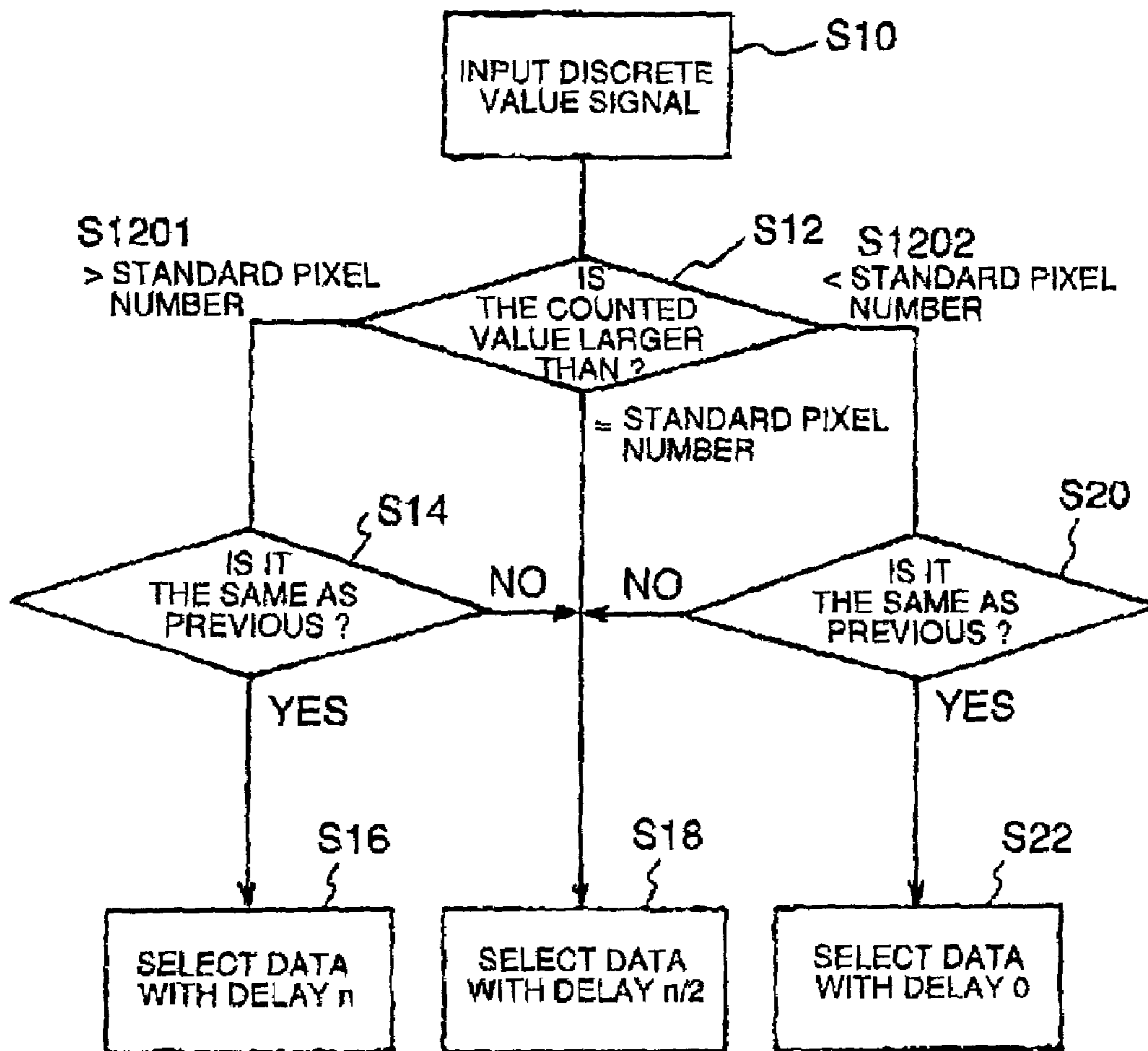
OPERATION OF THE INITIAL VALUE JUDGMENT CIRCUIT
