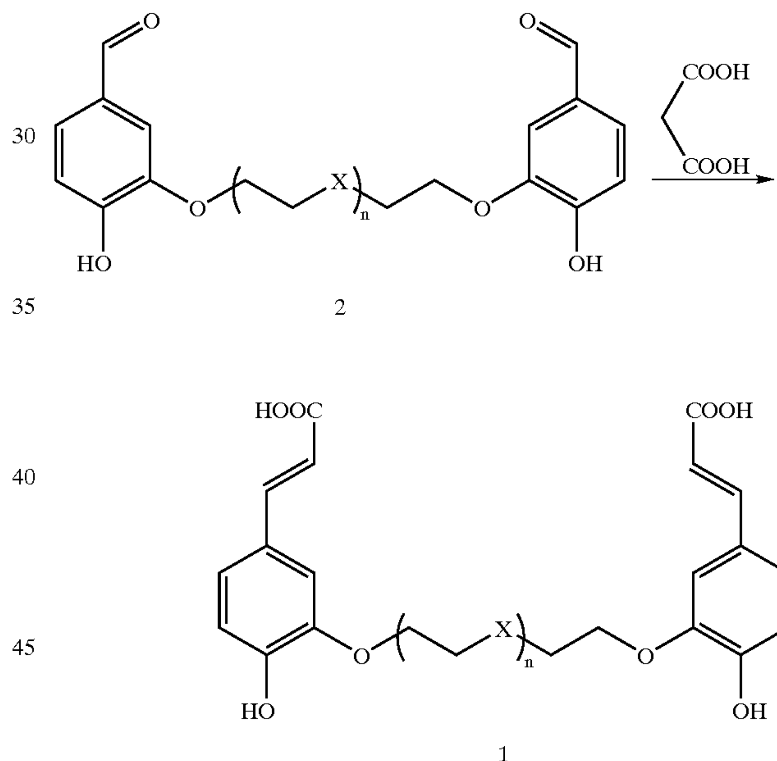
Reaction scheme 1
