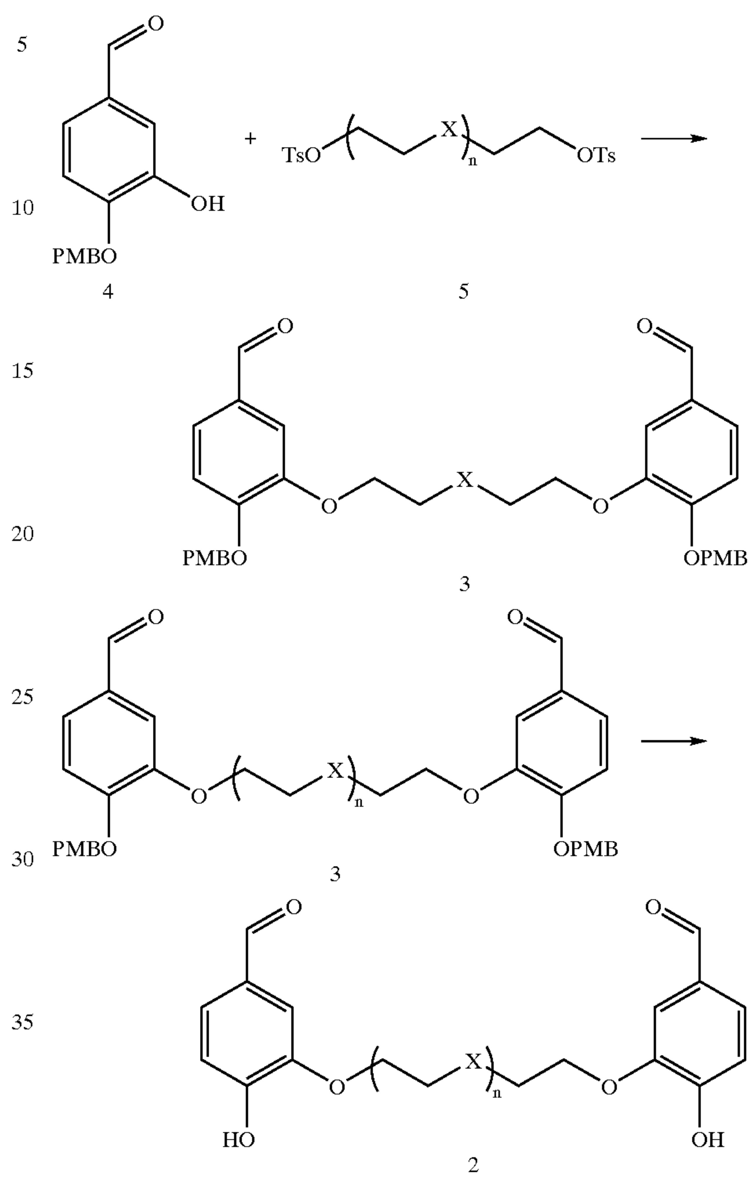
Reaction scheme 2
