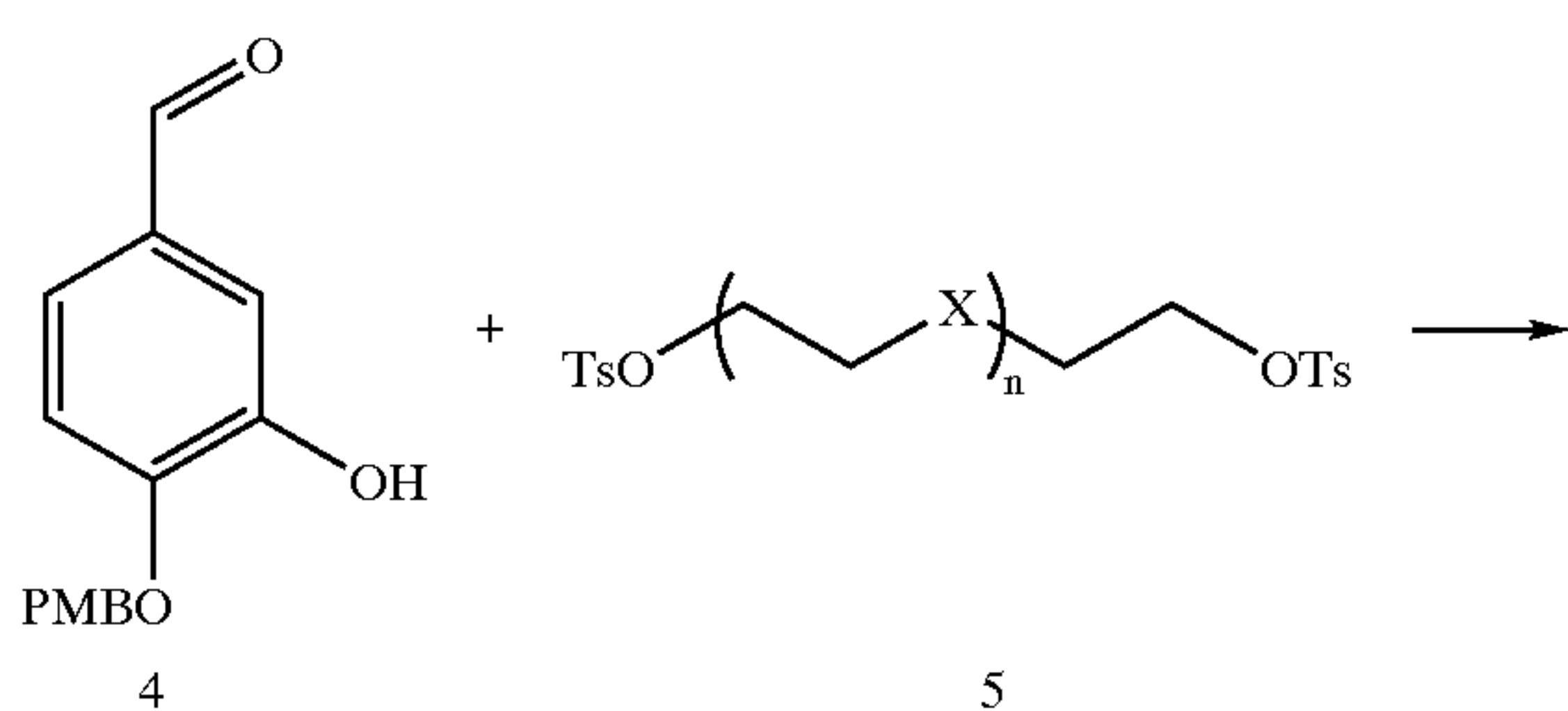
Reaction scheme 2
