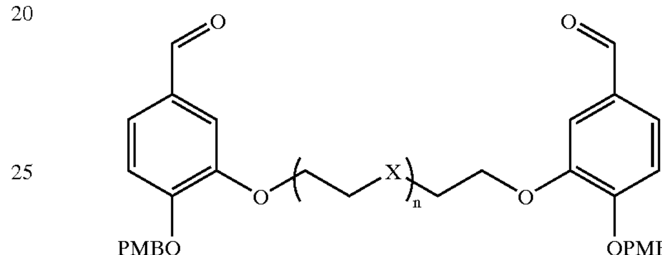
Formula 3
