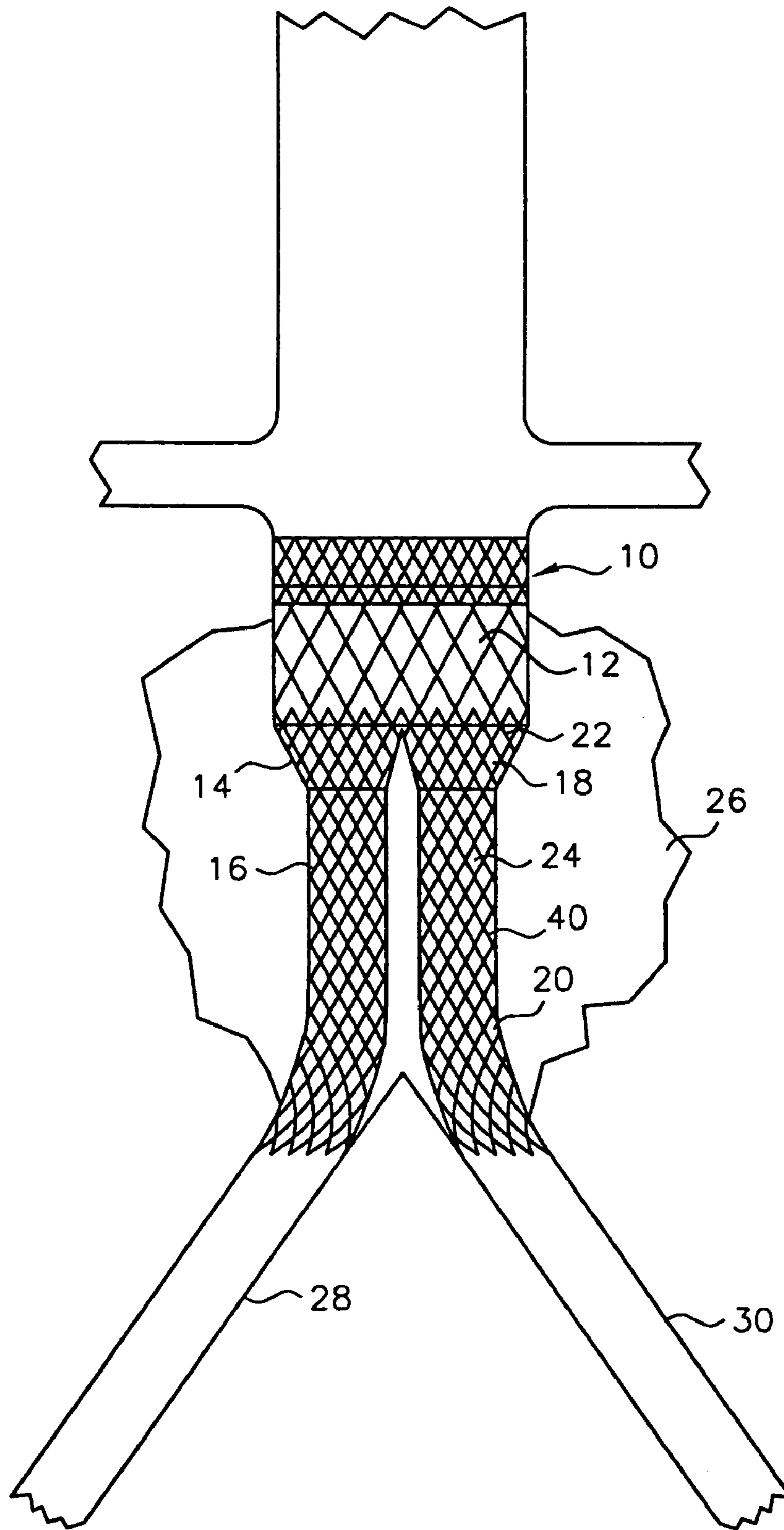
FIG. 2 (Prior Art)
