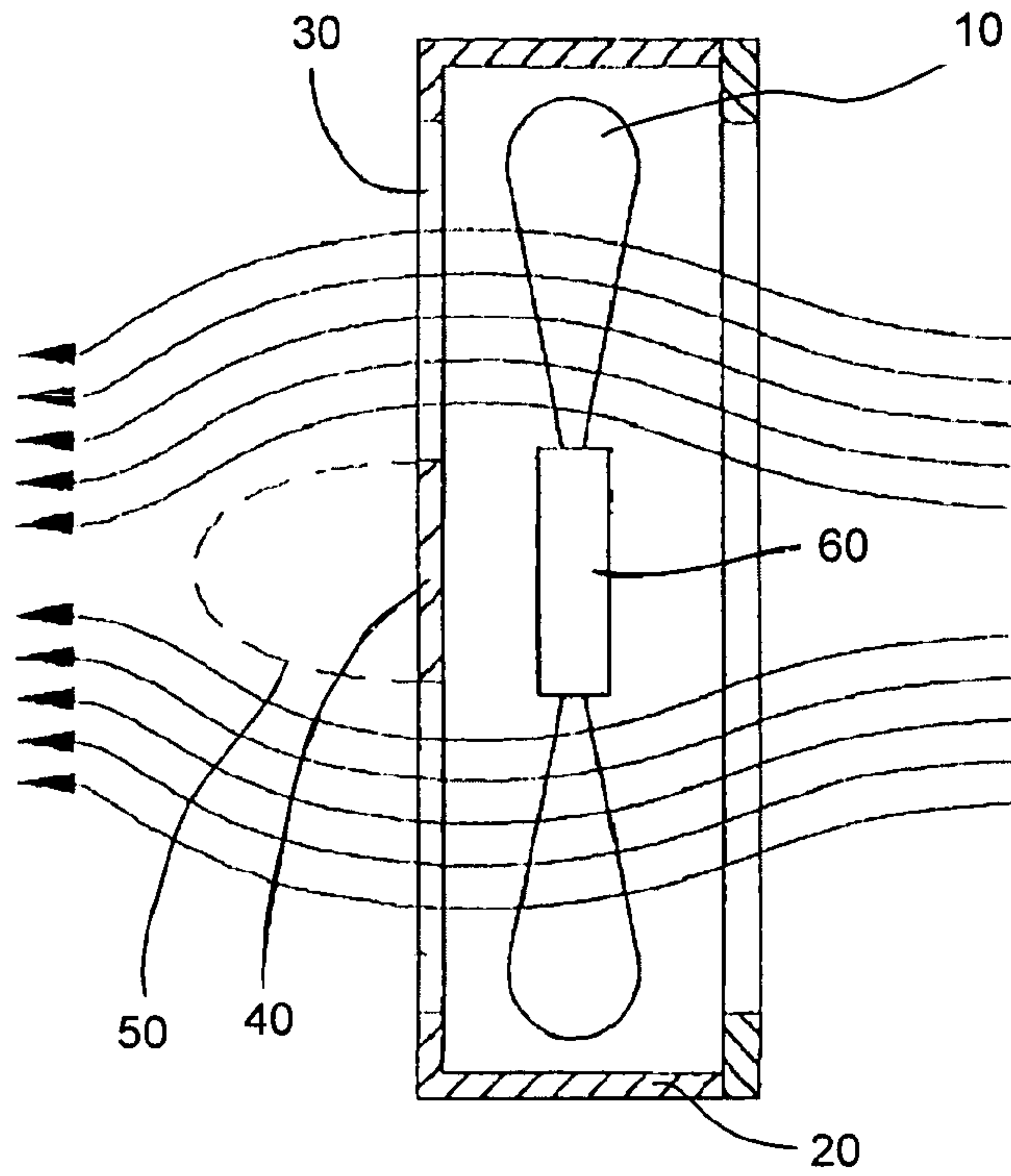
Fig. 3 (prior art)
