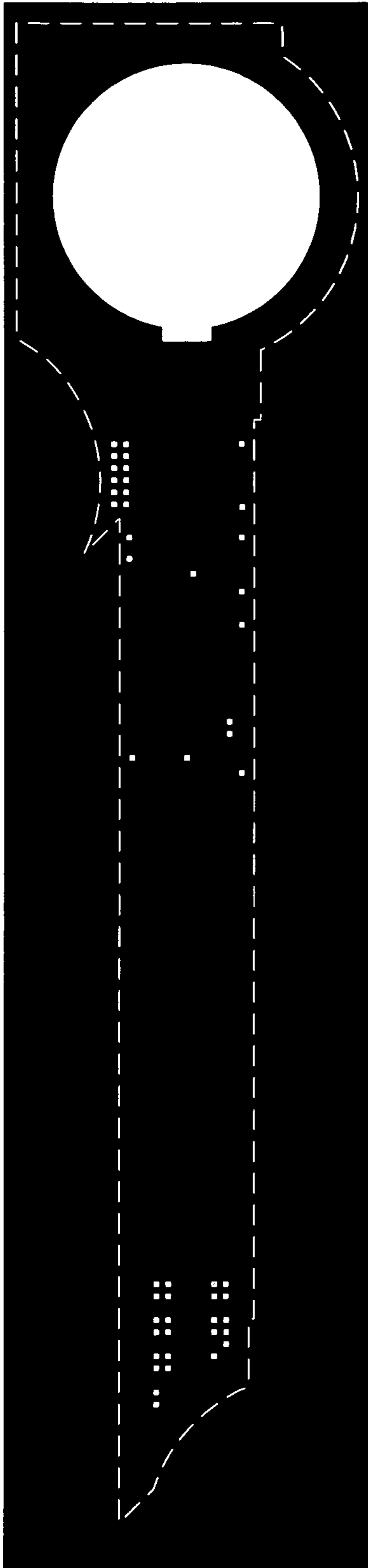
Via 1 mask
