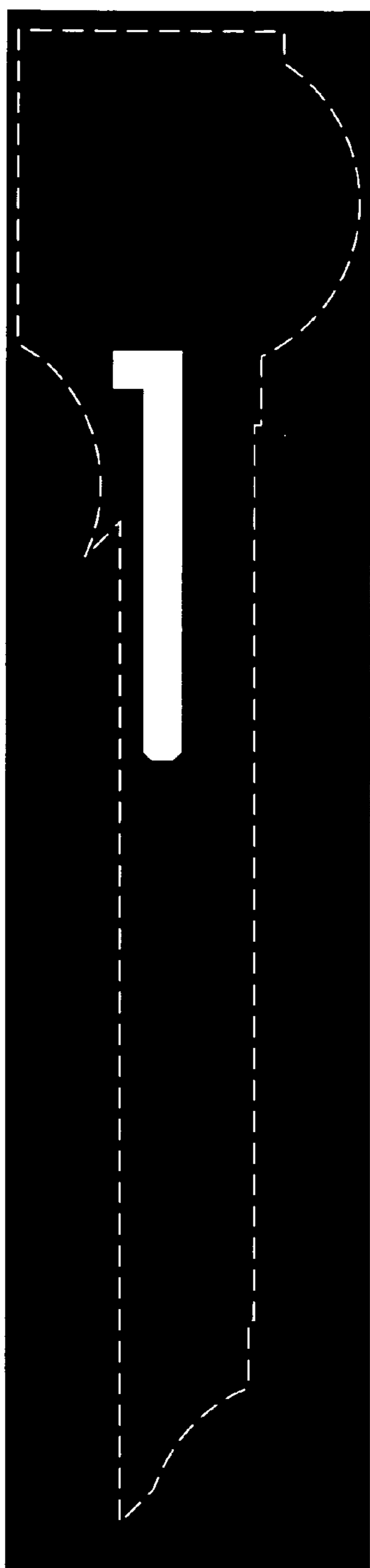
N-Well mask
