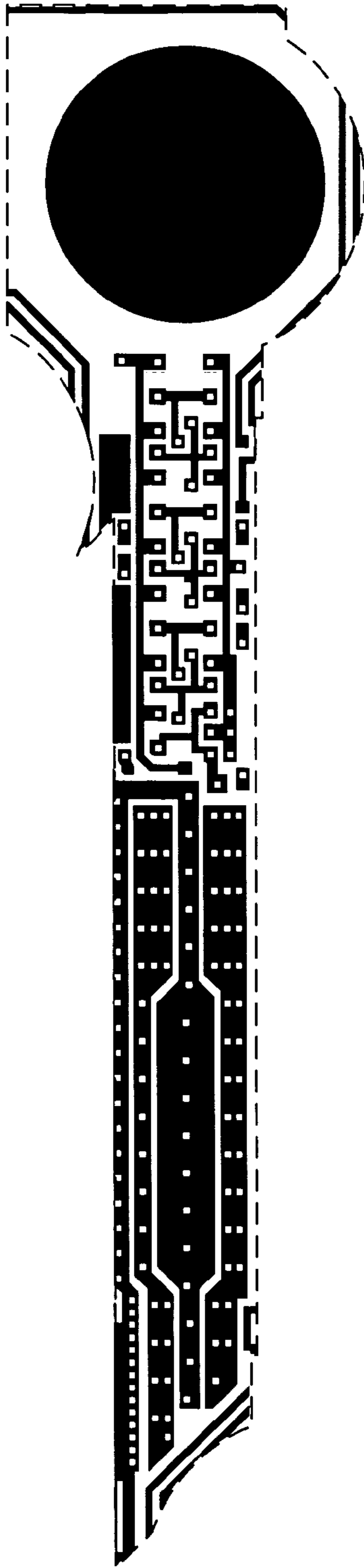
Metal 1 mask
