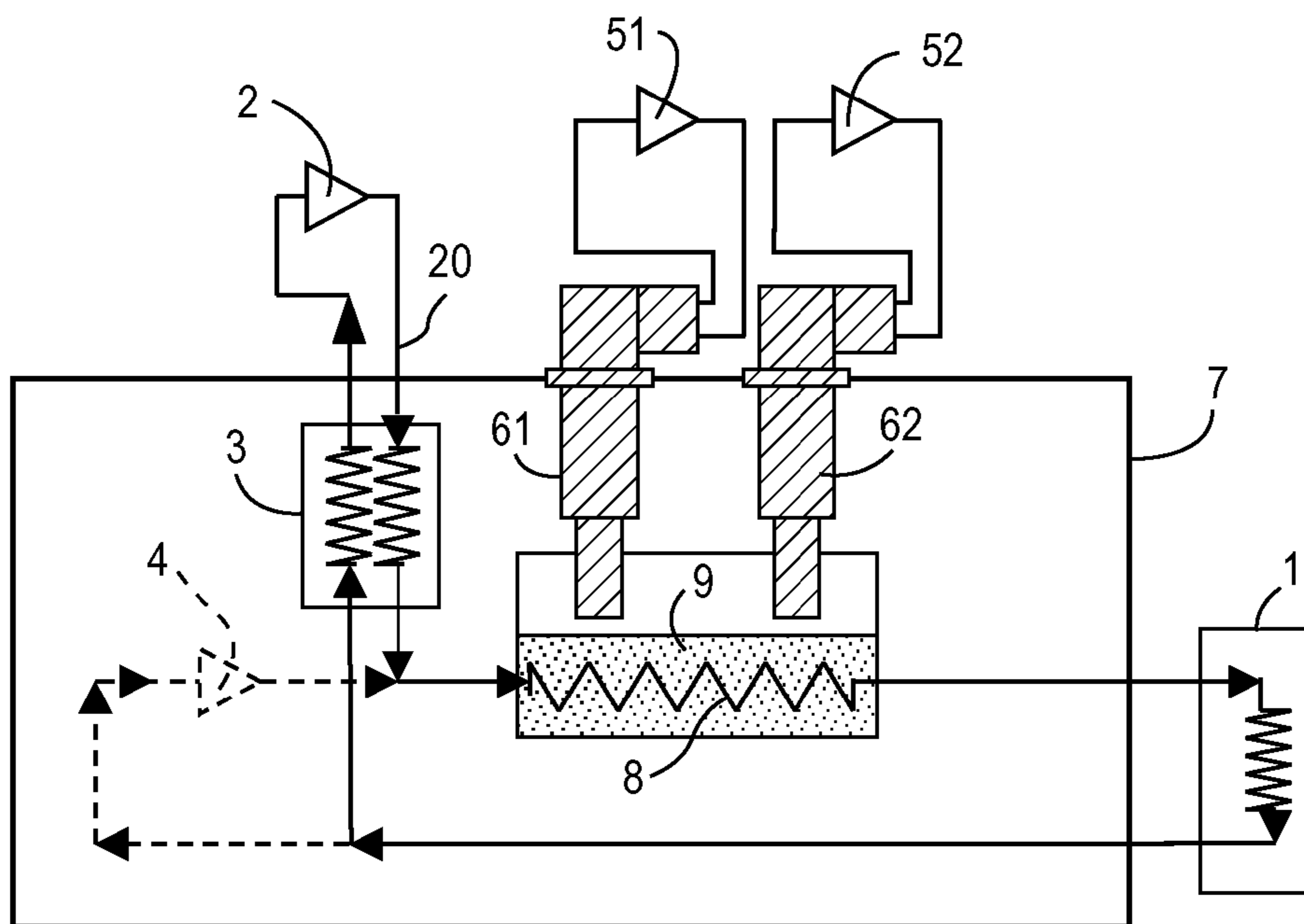
Fig. 6 (Prior Art)
