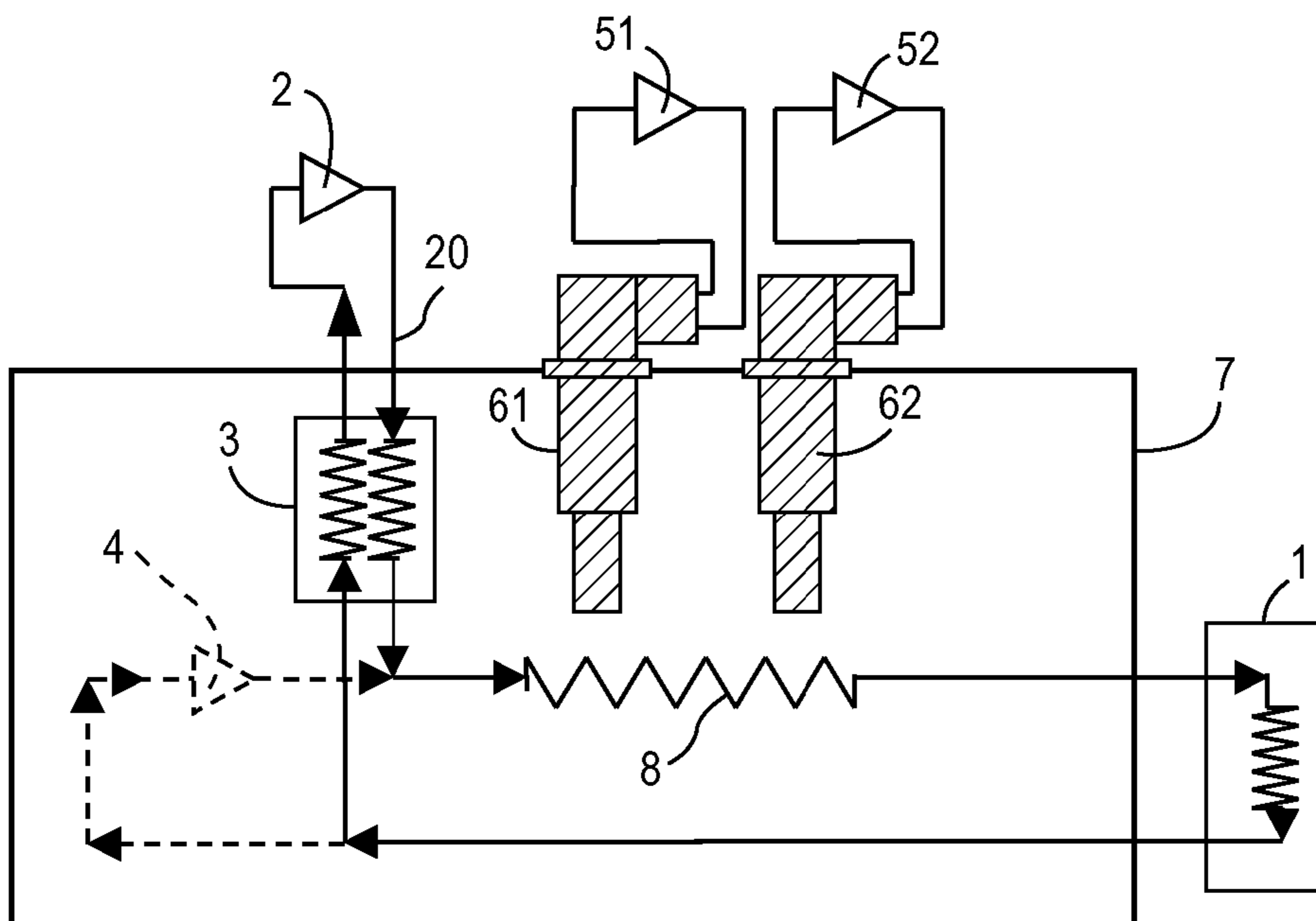
Fig. 5 (Prior Art)
