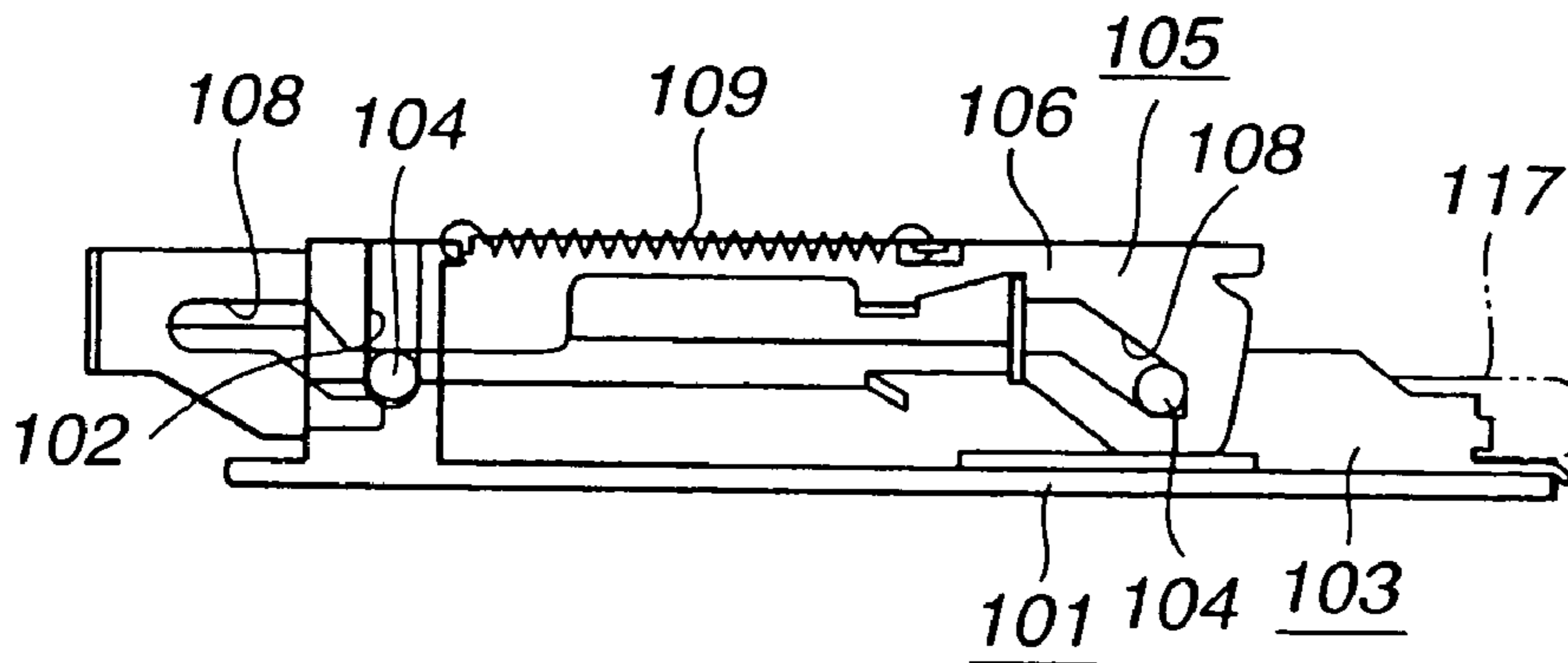
FIG. 5 (PRIOR ART)
