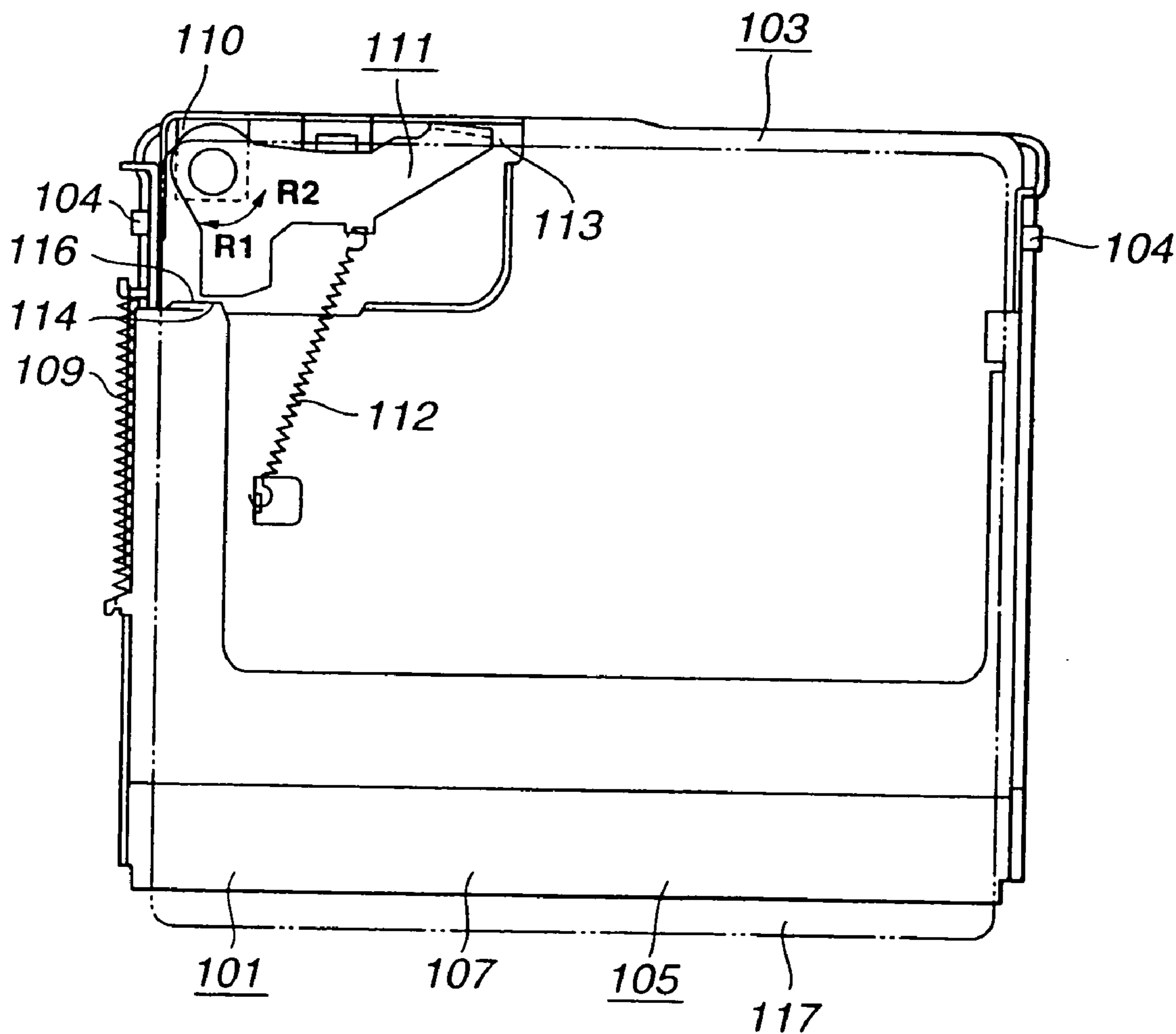
FIG. 3 (PRIOR ART)
