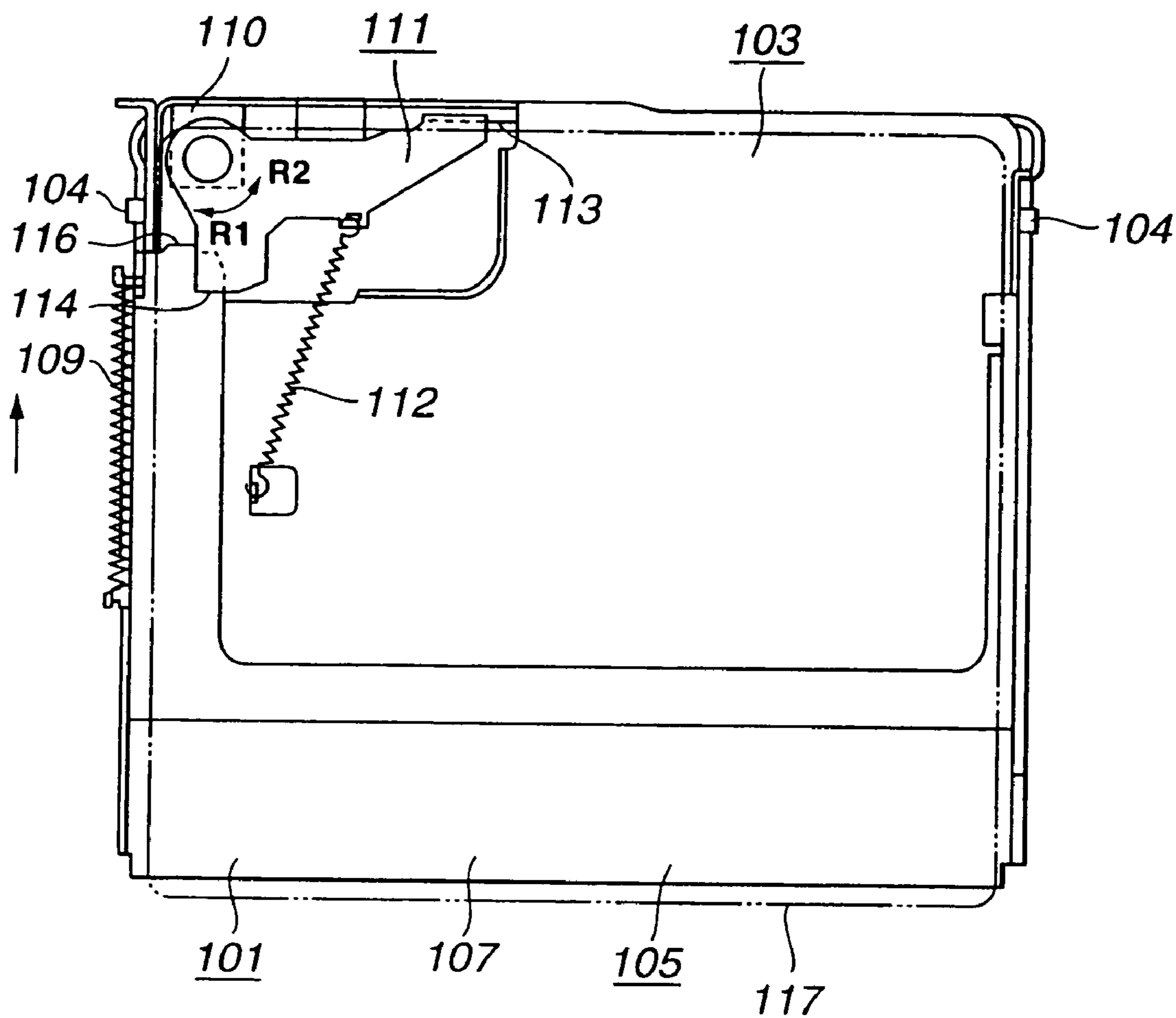
FIG. 4 (PRIOR ART)
