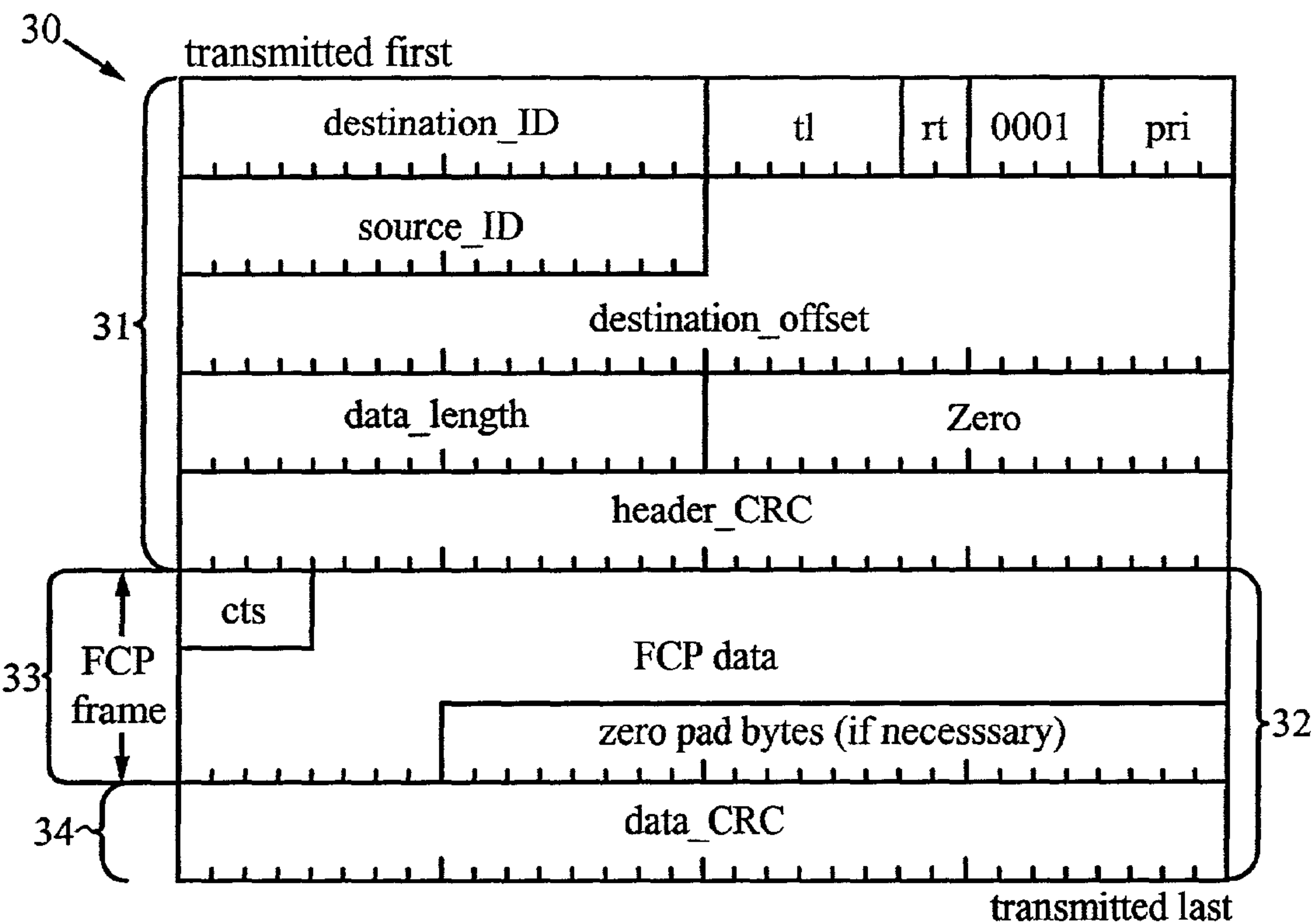
Fig. 2 PRIOR ART
