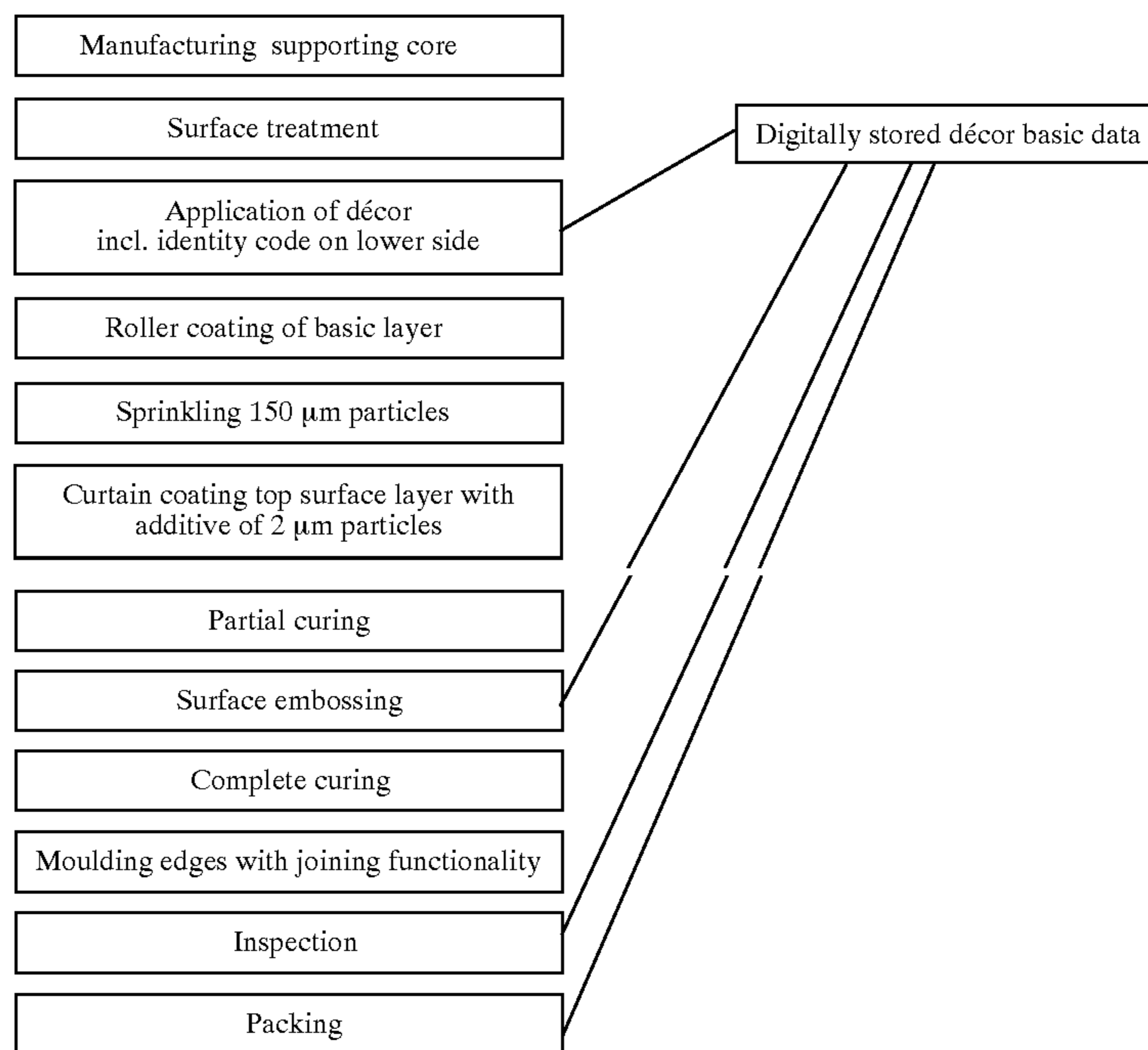
Process scheme 2.
