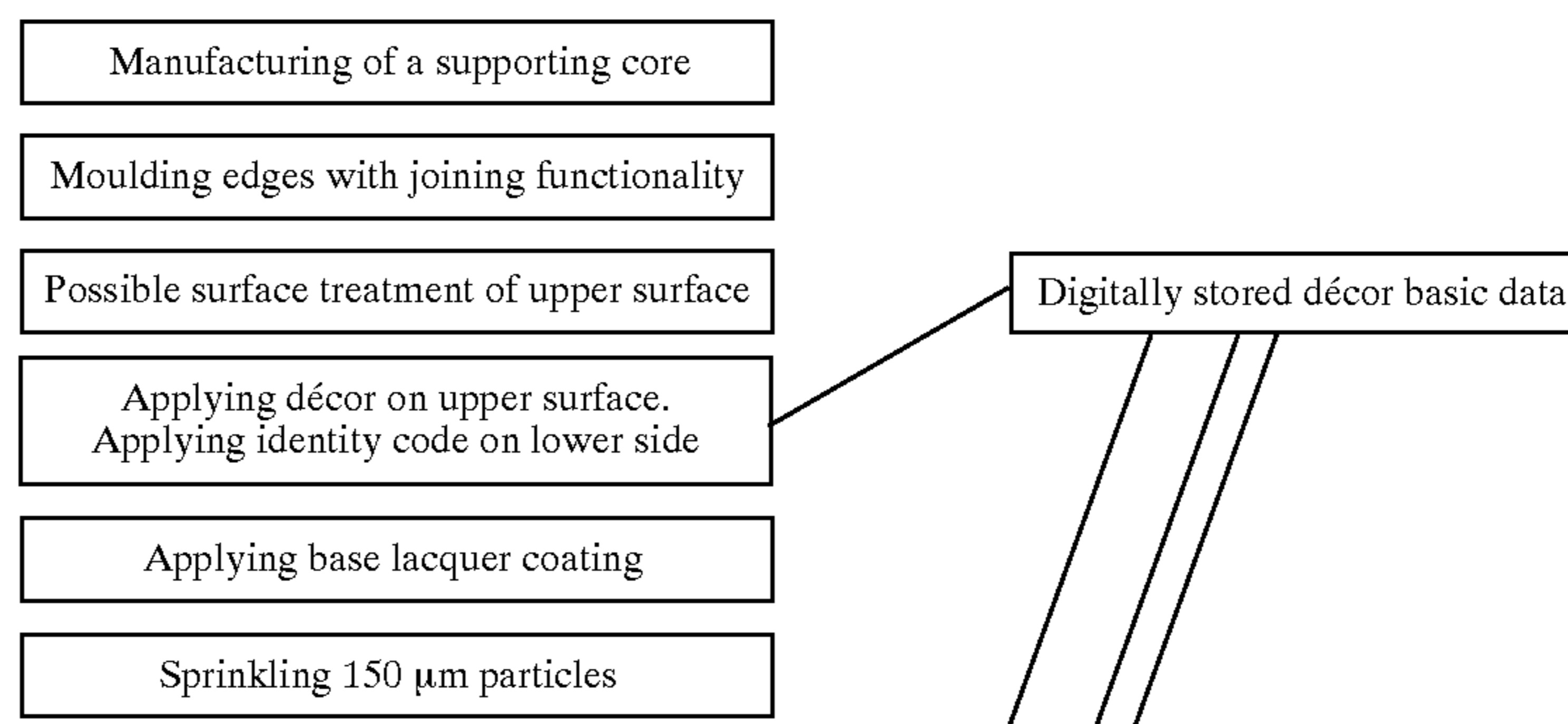
Process scheme 1.
