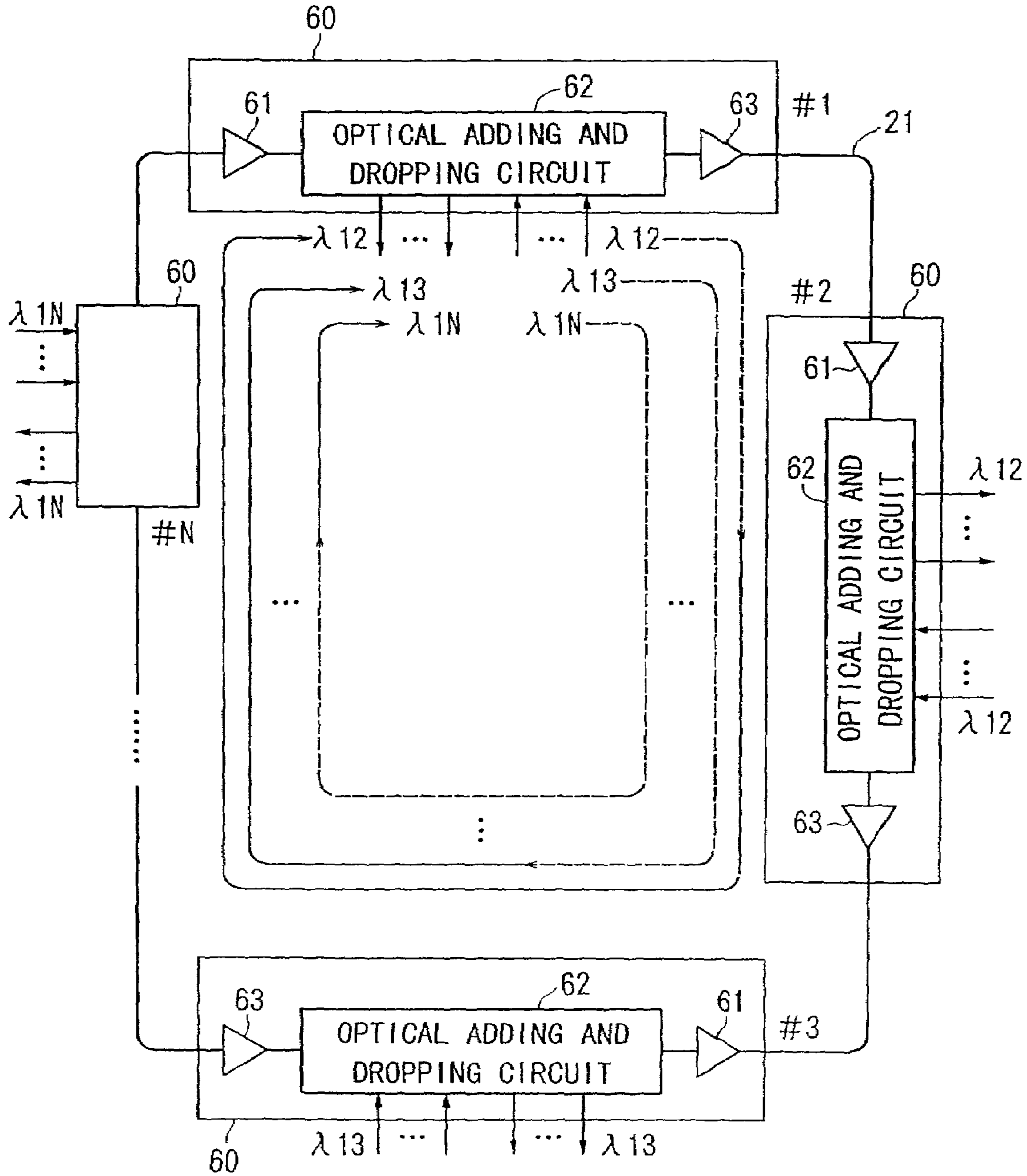
STRUCTURE OF THE FIFTH EMBODIMENT OF THE PRESENT INVENTION
