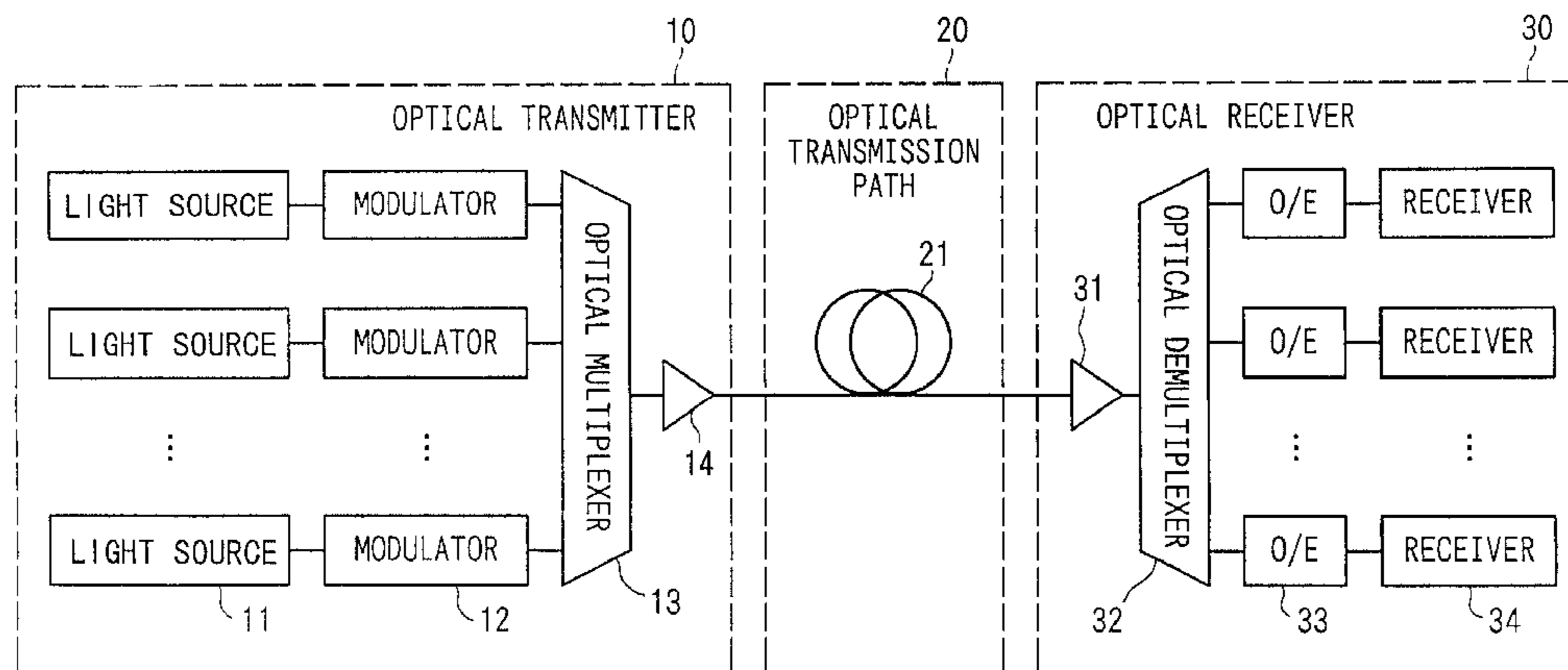
STRUCTURE OF THE FIRST EMBODIMENT OF THE PRESENT INVENTION
