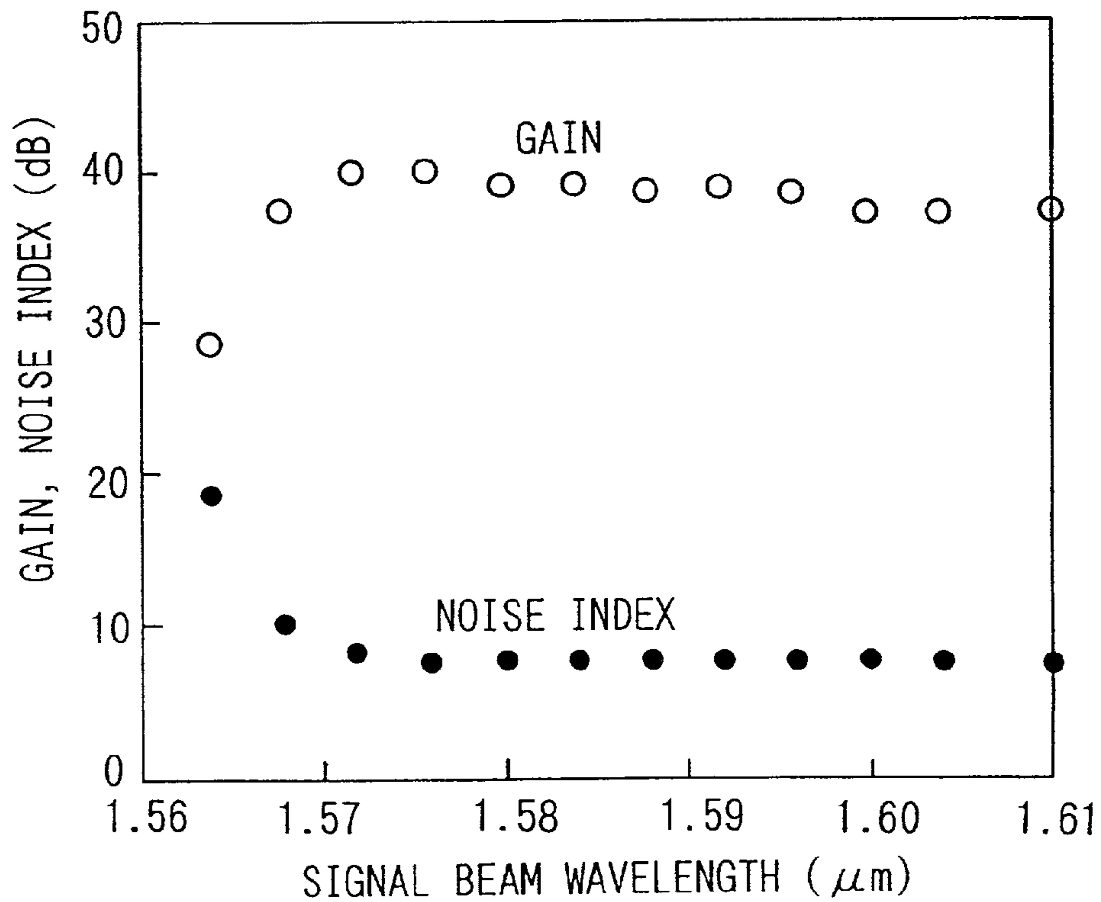
GAIN CHARACTERISTICS OF A Er-DOPED OPTICAL FIBER AMPLIFIER (GS-EDFA)
