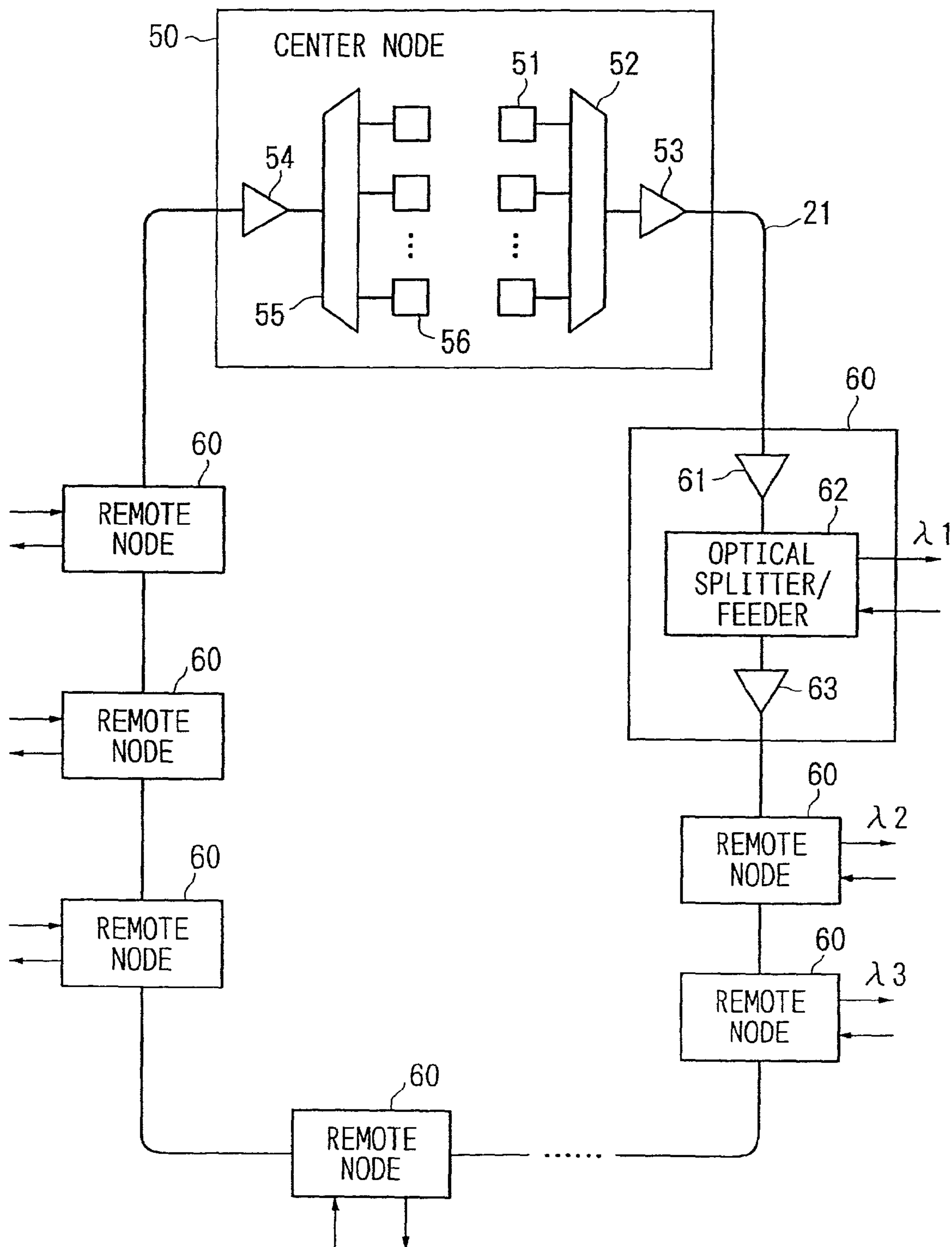
STRUCTURE OF THE FORTH EMBODIMENT OF THE PRESENT INVENTION
