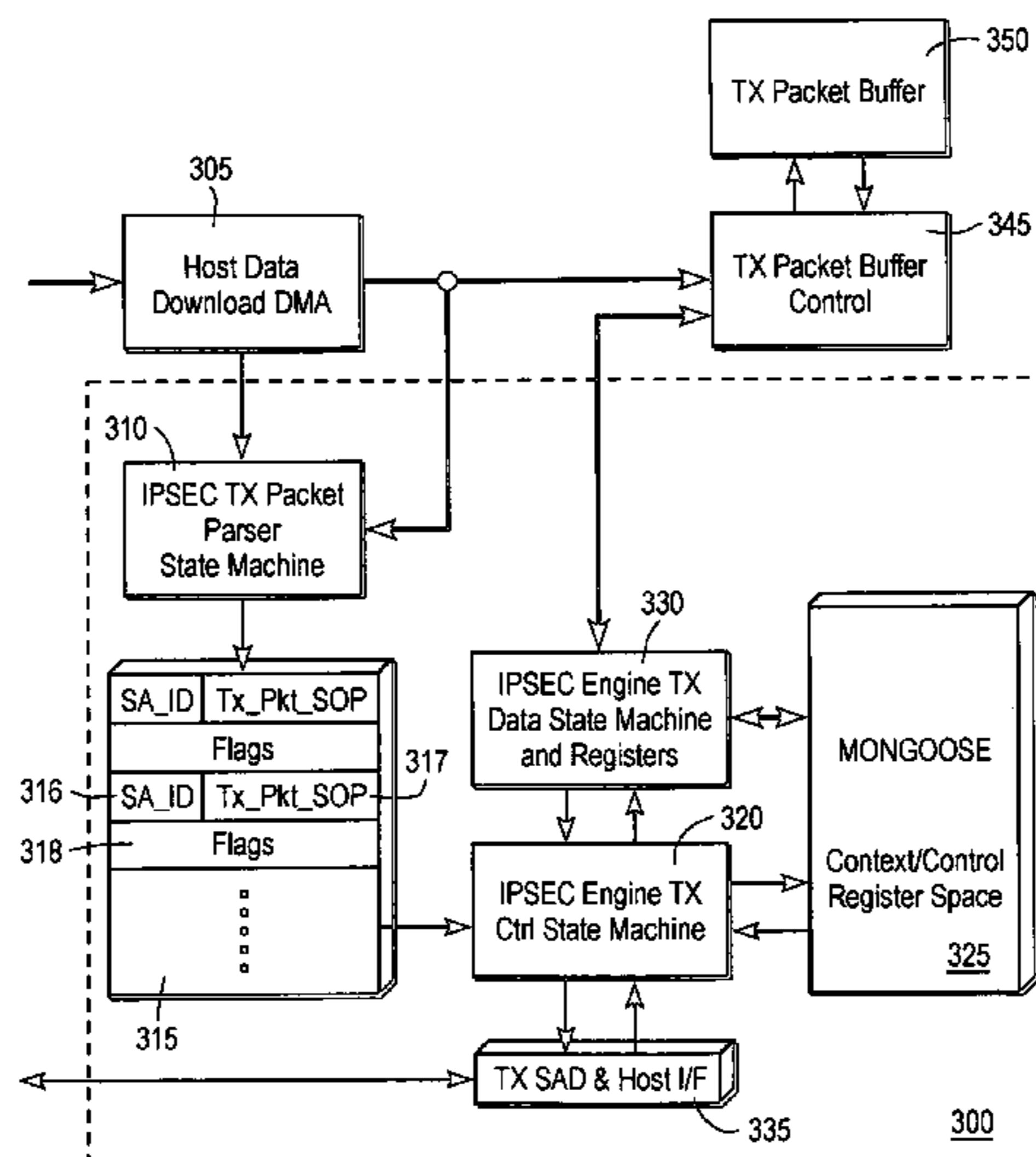
Hardware Architecture for Outbound Traffic
