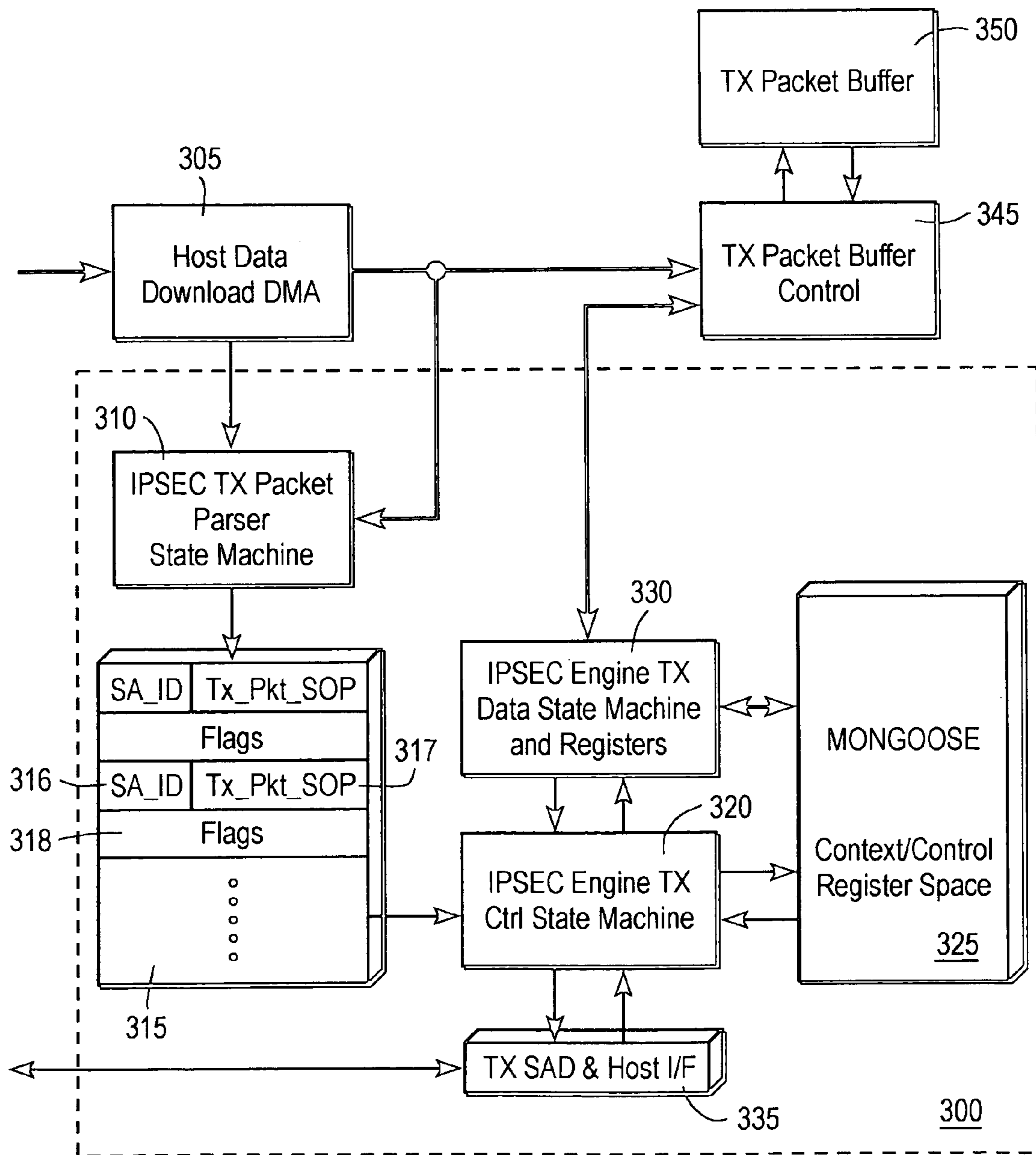
Hardware Architecture for Outbound Traffic
