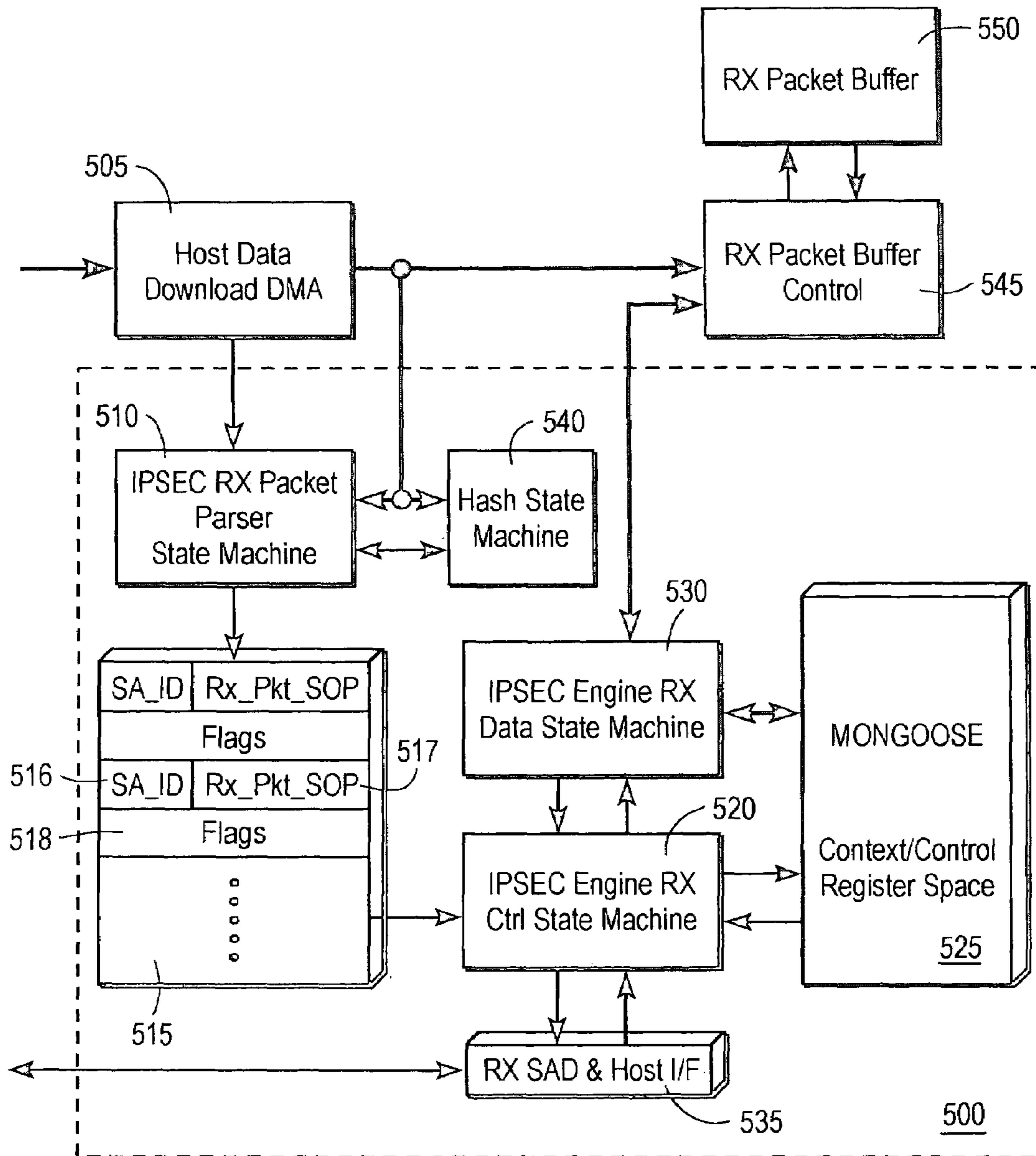
Hardware Architecture For Inbound Traffic
