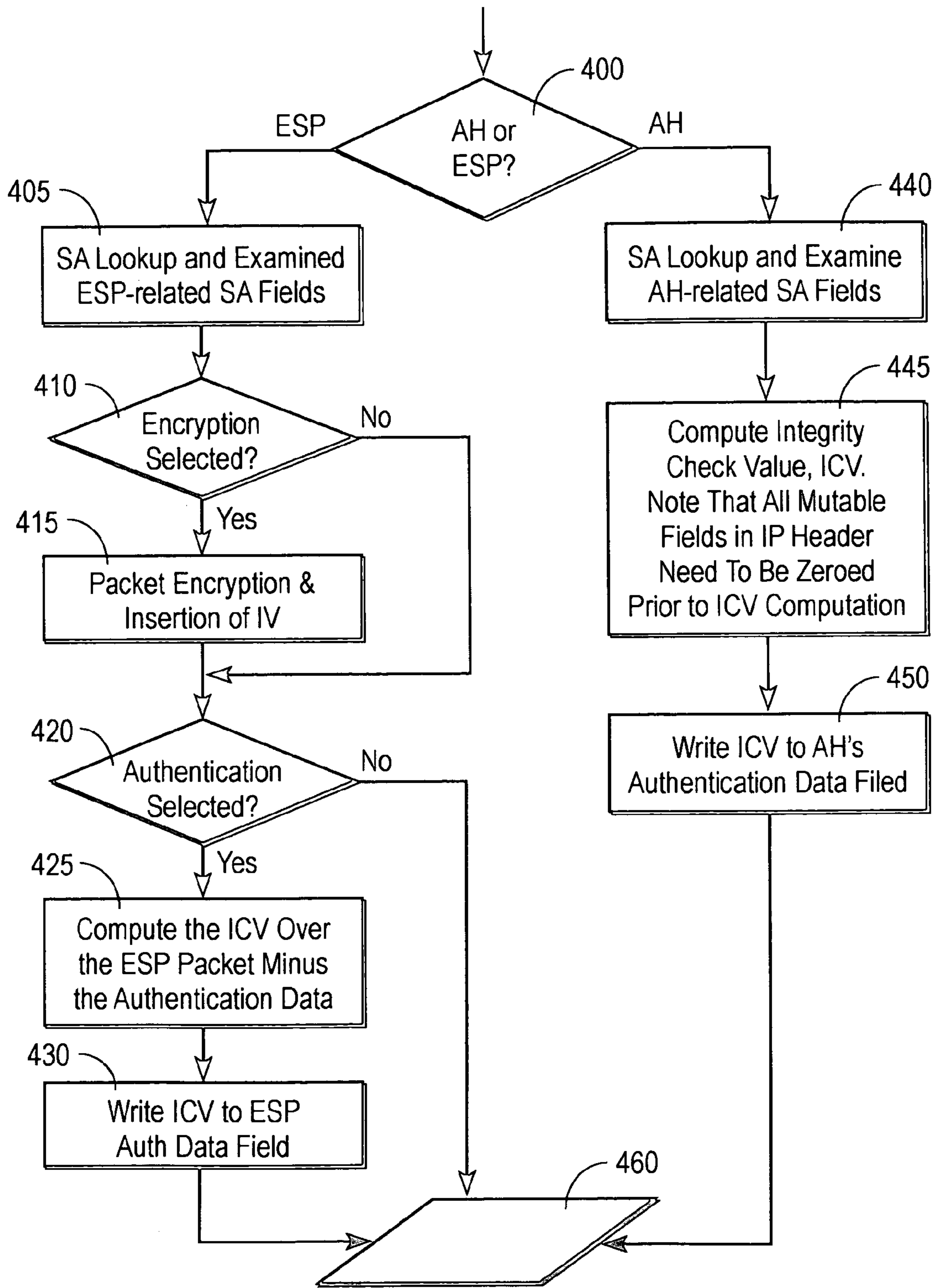
Outbound IP Traffic Processing Flow
