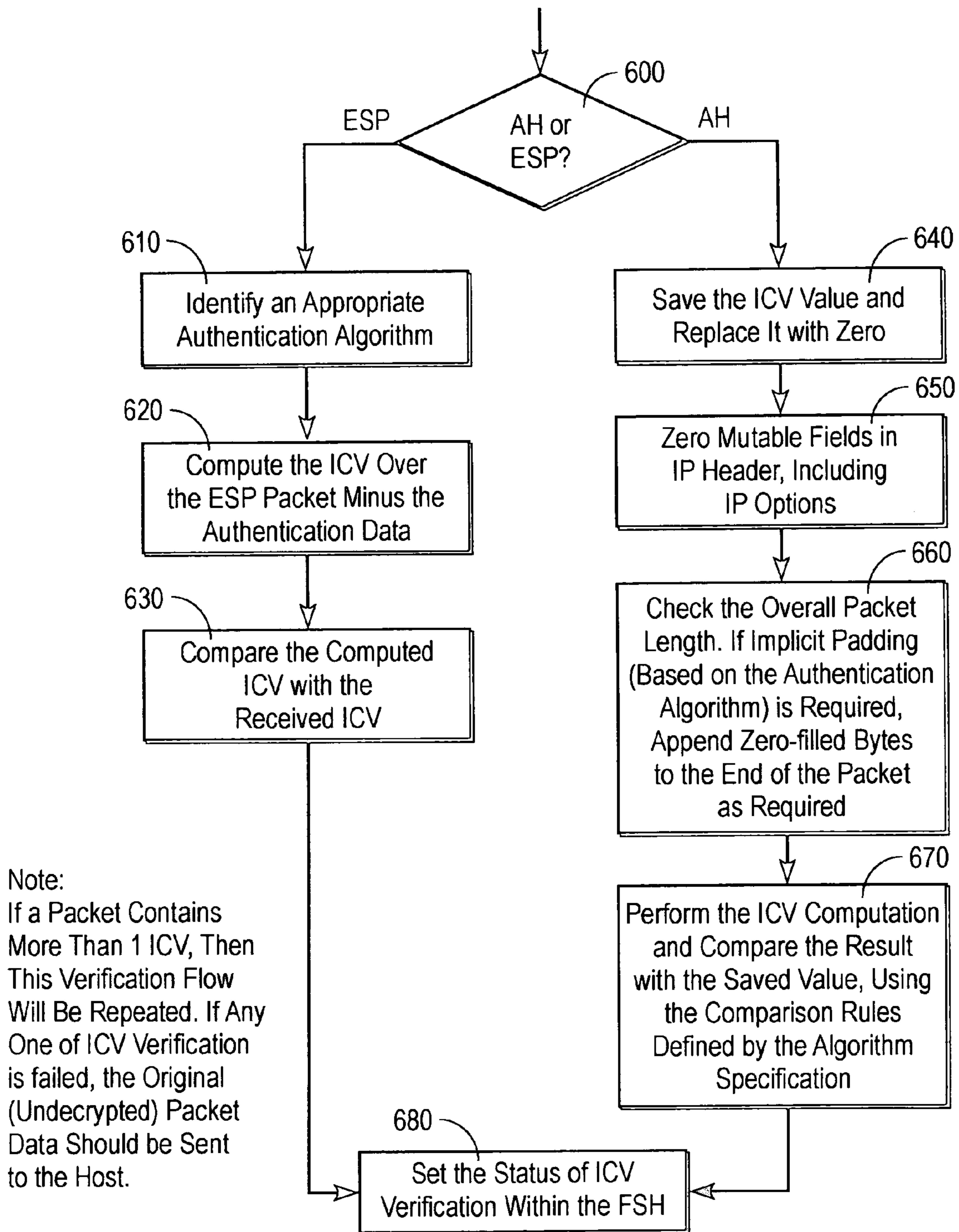
Verification For Inbound Traffic
