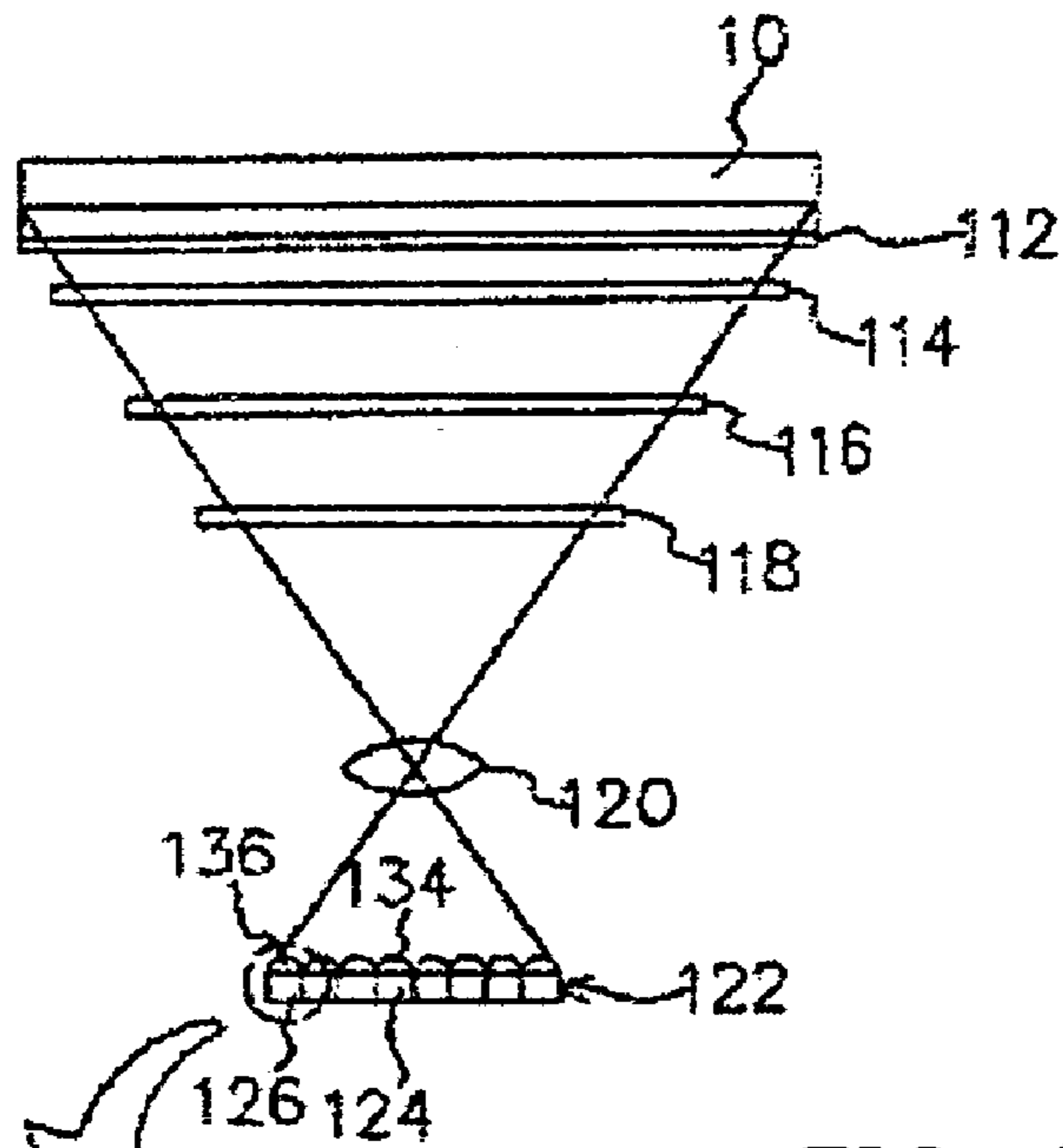
FIG. 2 (PRIOR ART)
