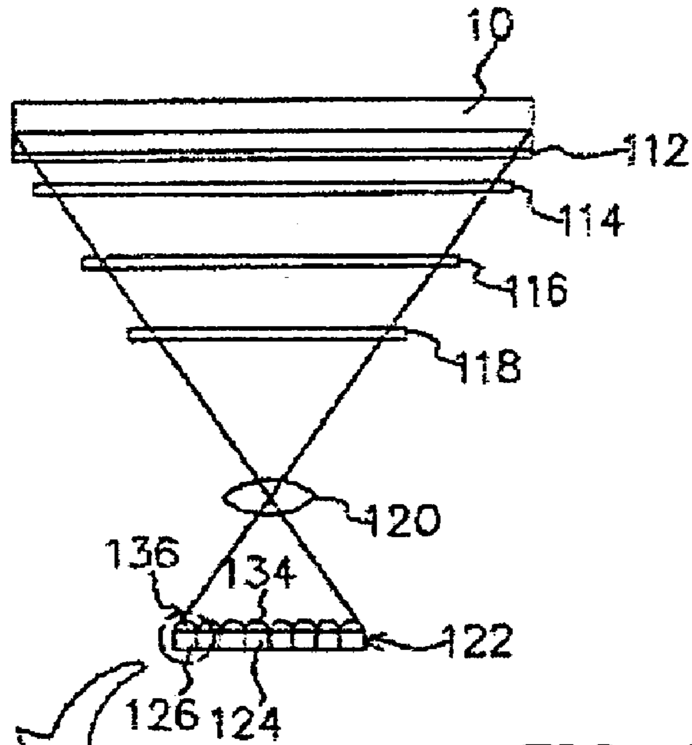
FIG. 2 (PRIOR ART)
