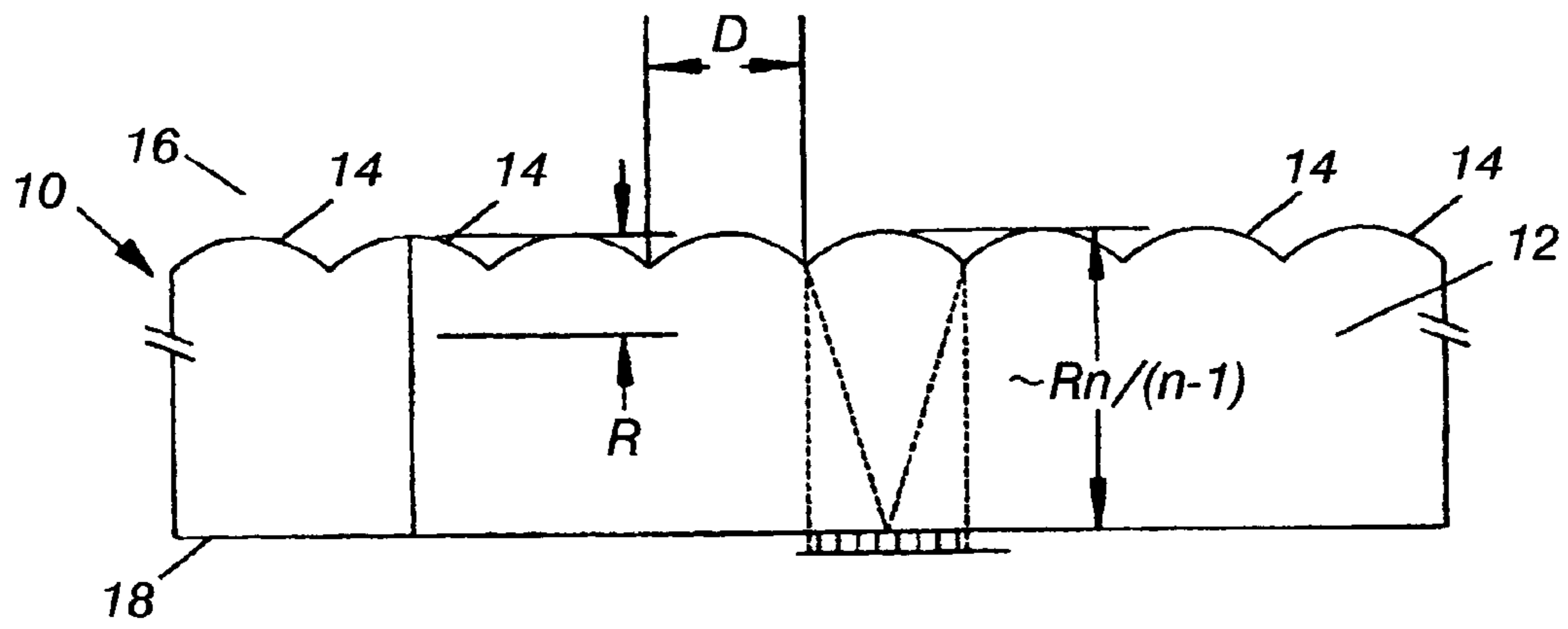
Fig. 2 (PRIOR ART)
