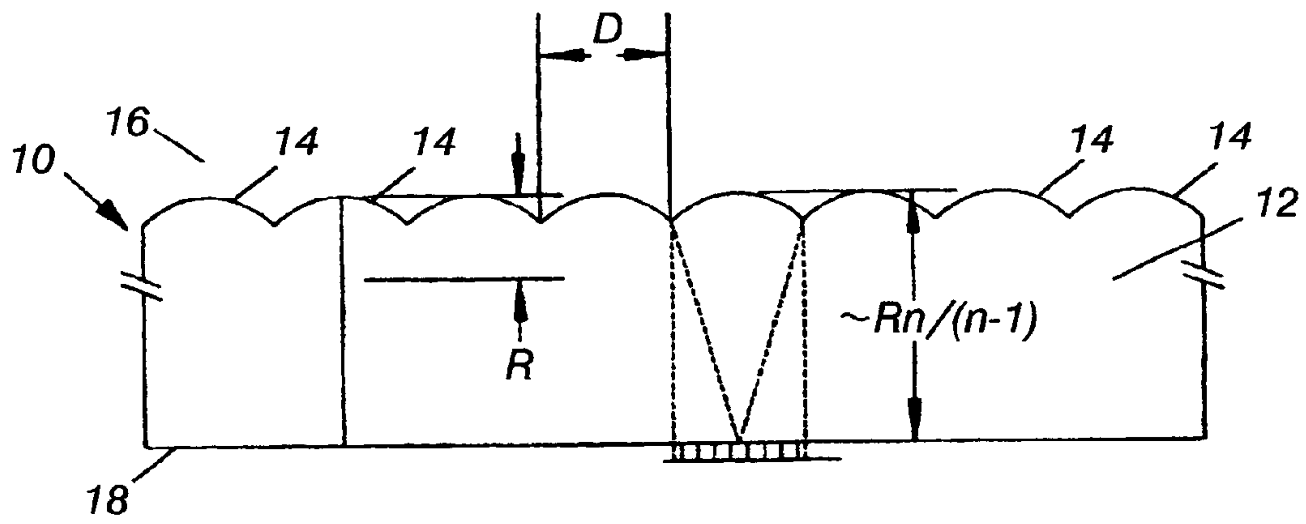
Fig. 2 (PRIOR ART)
