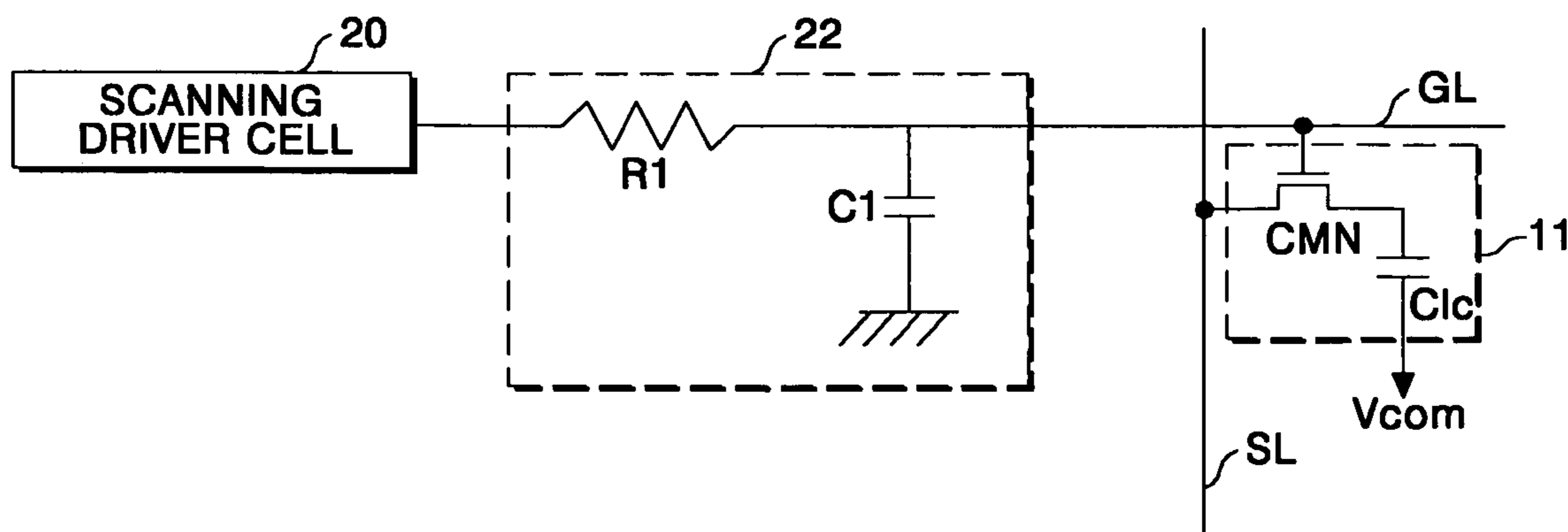
FIG. 3 PRIOR ART
