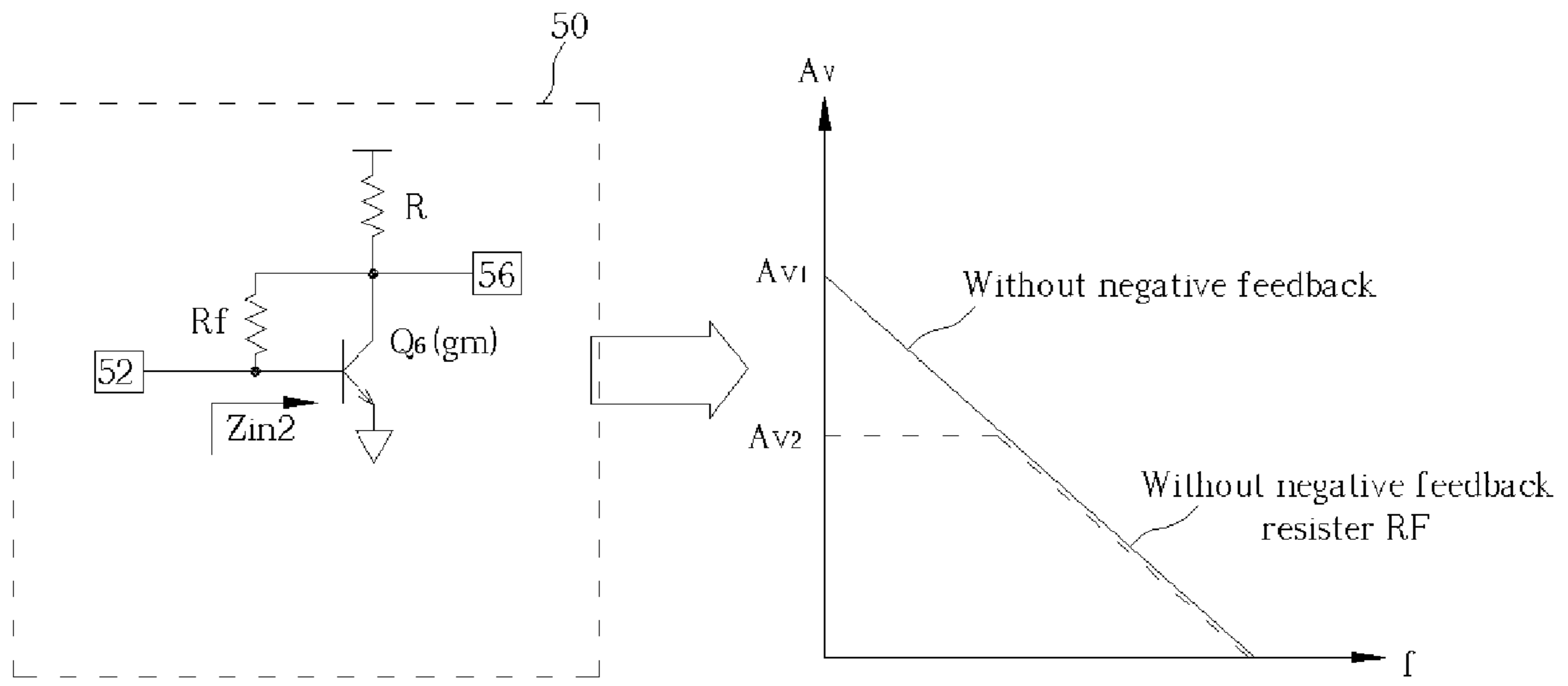
Fig. 4 Prior Art
