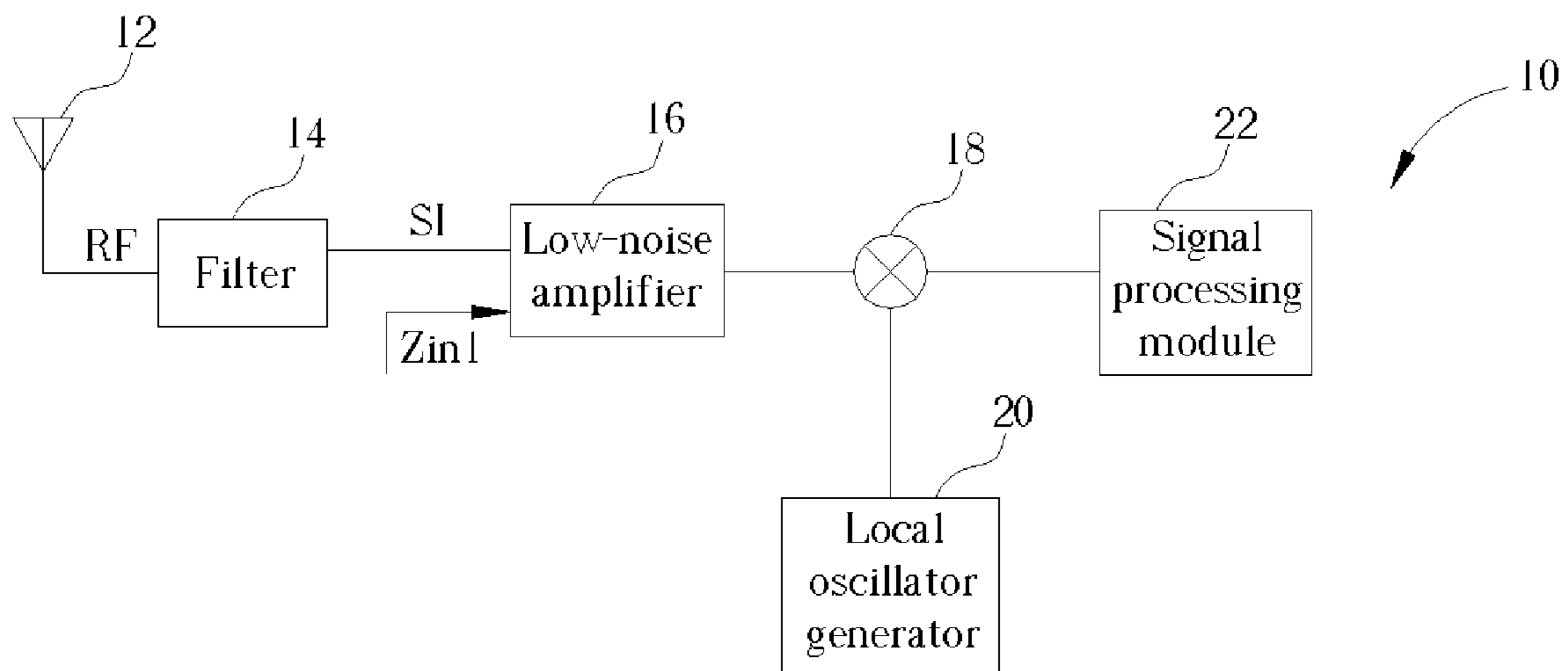
Fig. 1 Prior Art
