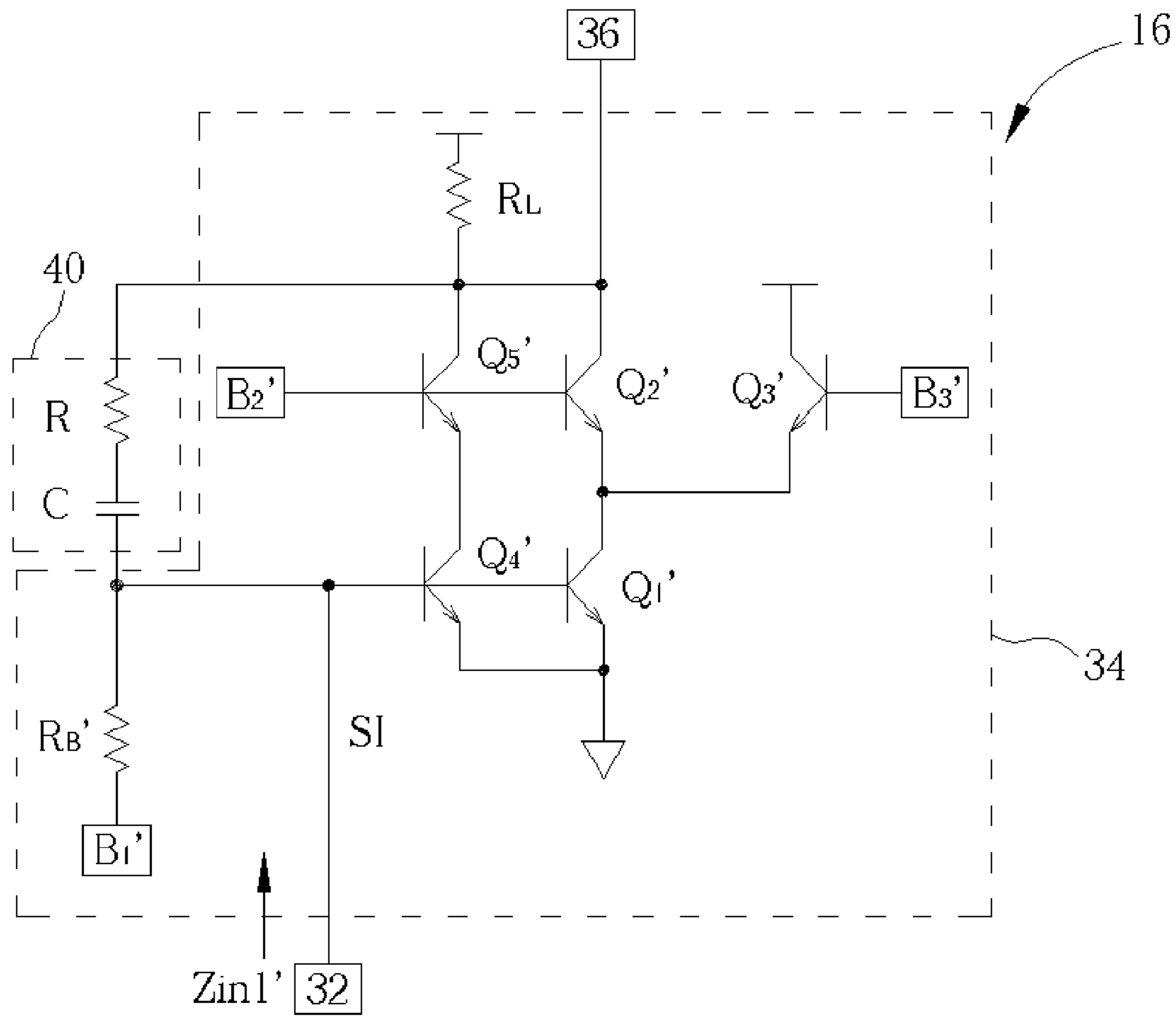
Fig. 3 Prior Art
