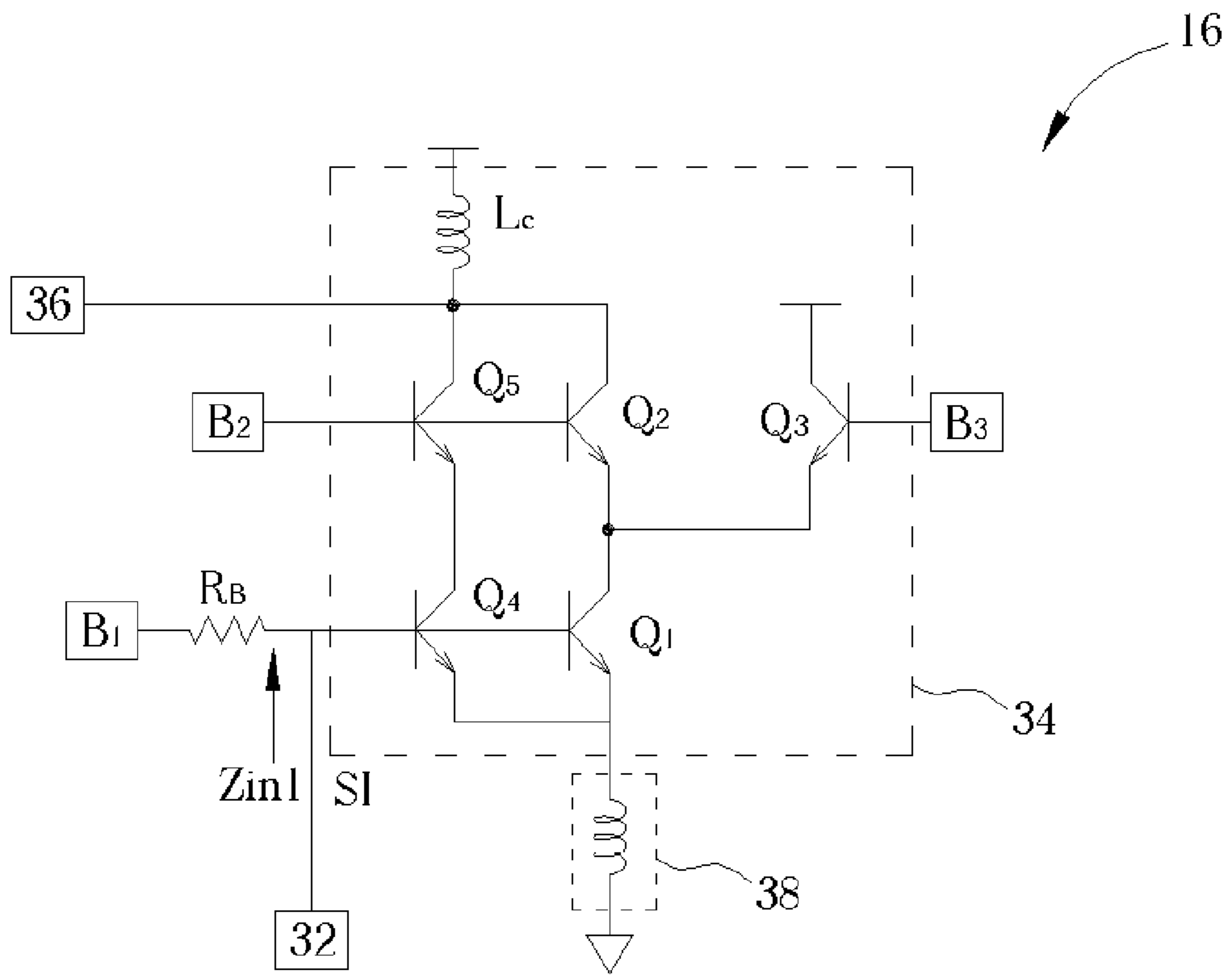
Fig. 2 Prior Art
