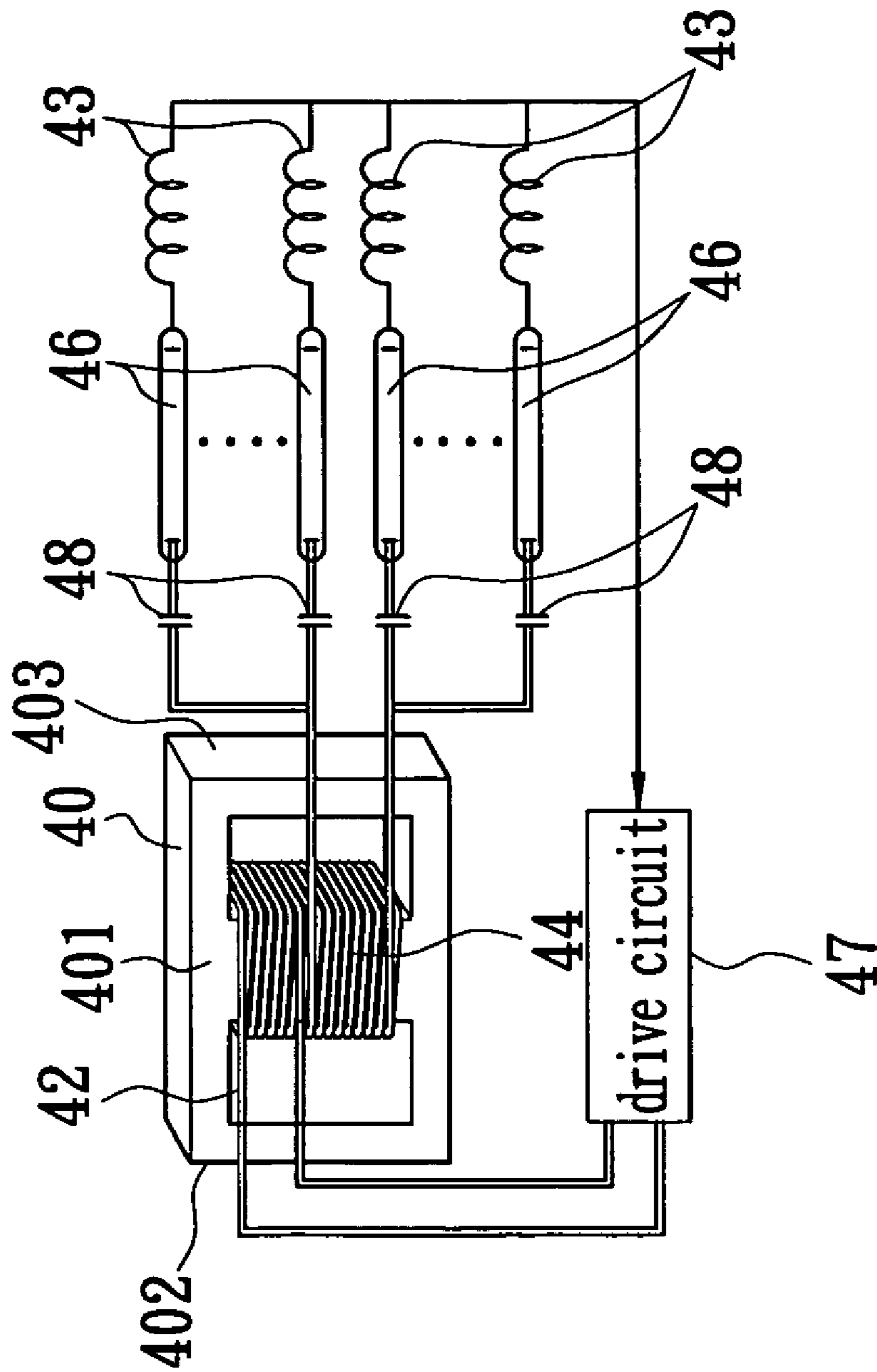
FIG. 1 PRIOR ART
