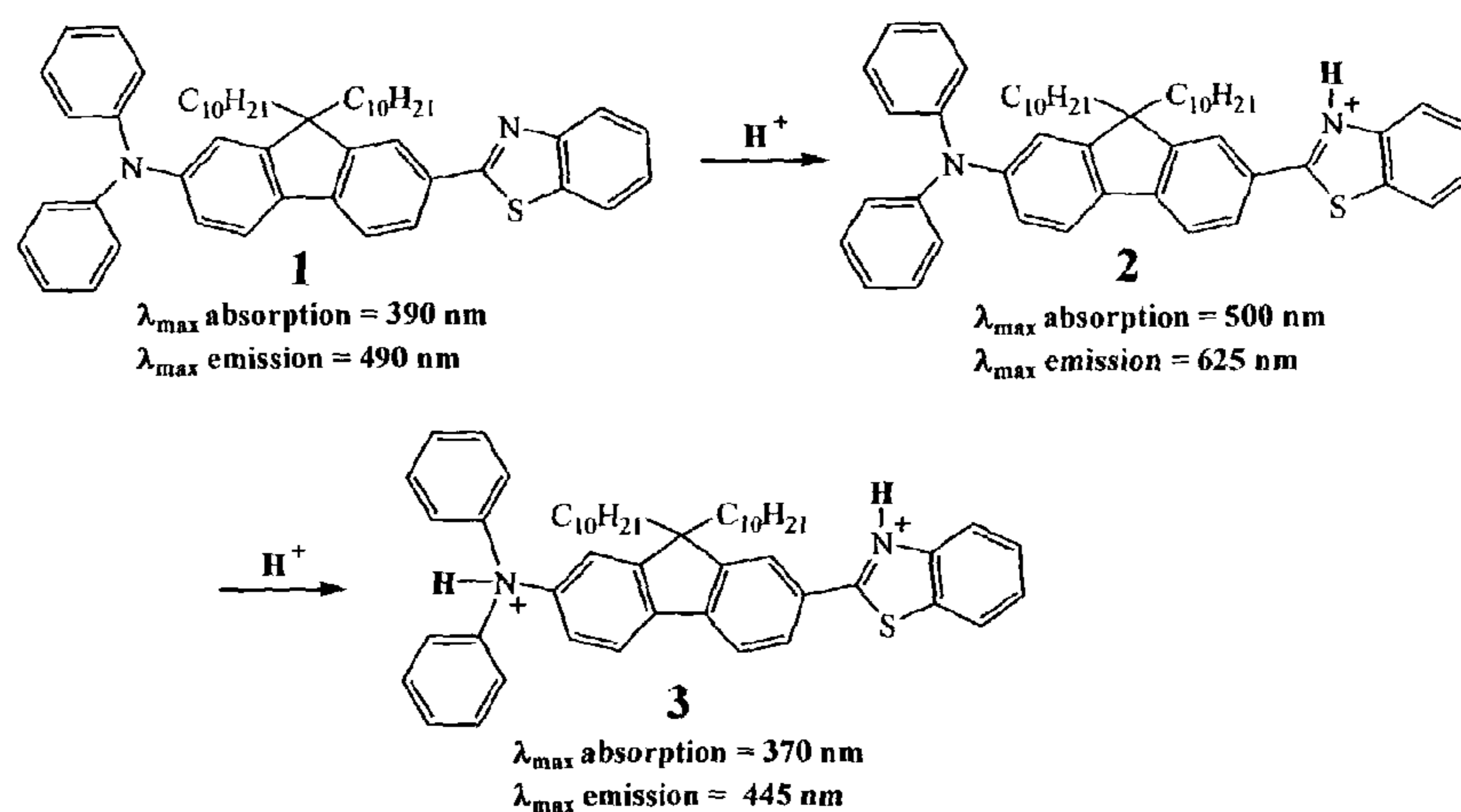
Figure 1 shows the reaction of fluorene dye 1 with acid resulting in the formation of monoprotinated 2 and diprotonated 3 products.
