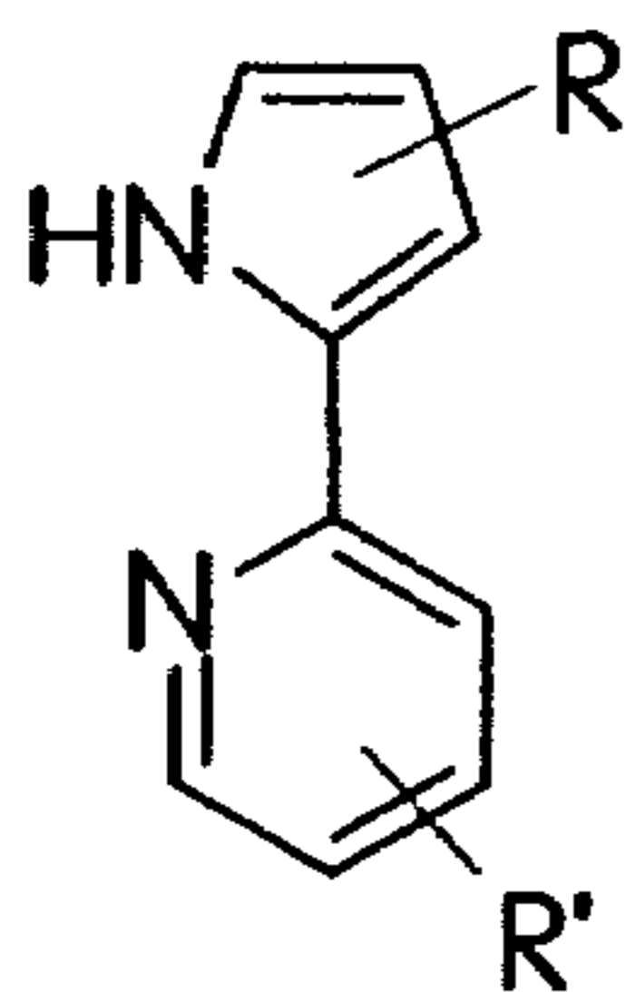
pyridylpyroles
