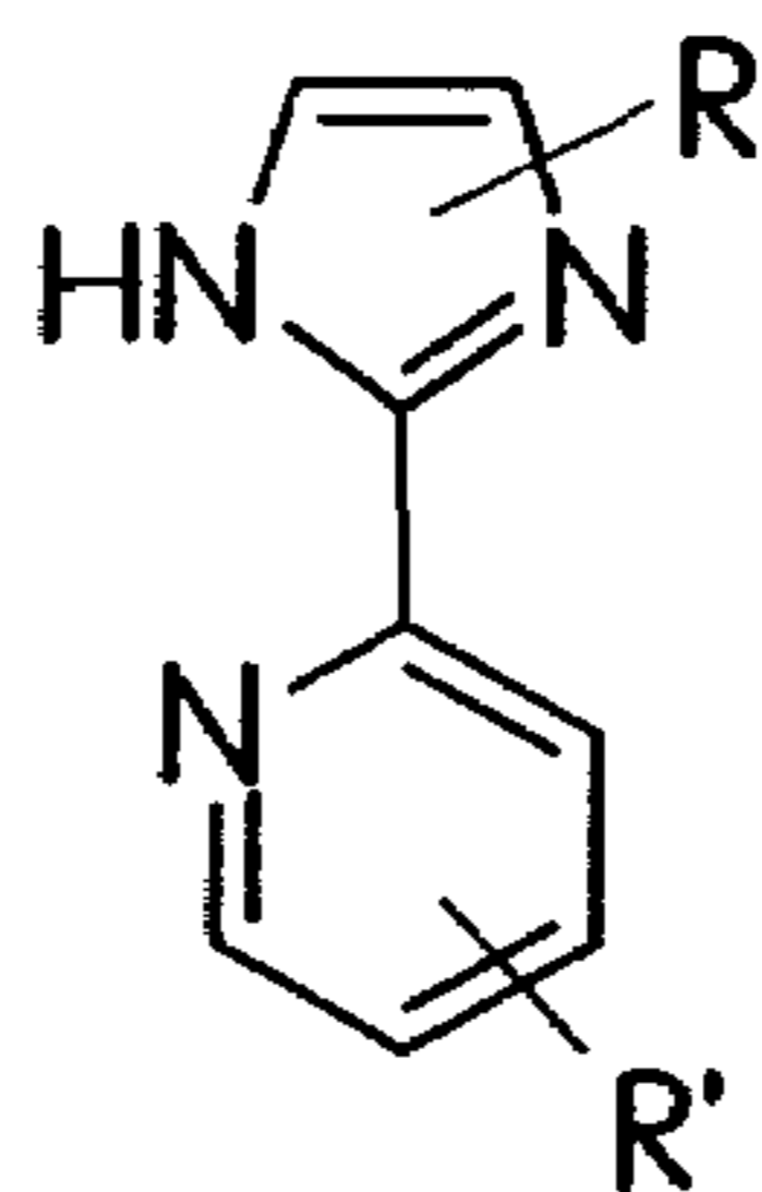
pyridylimidazoles
