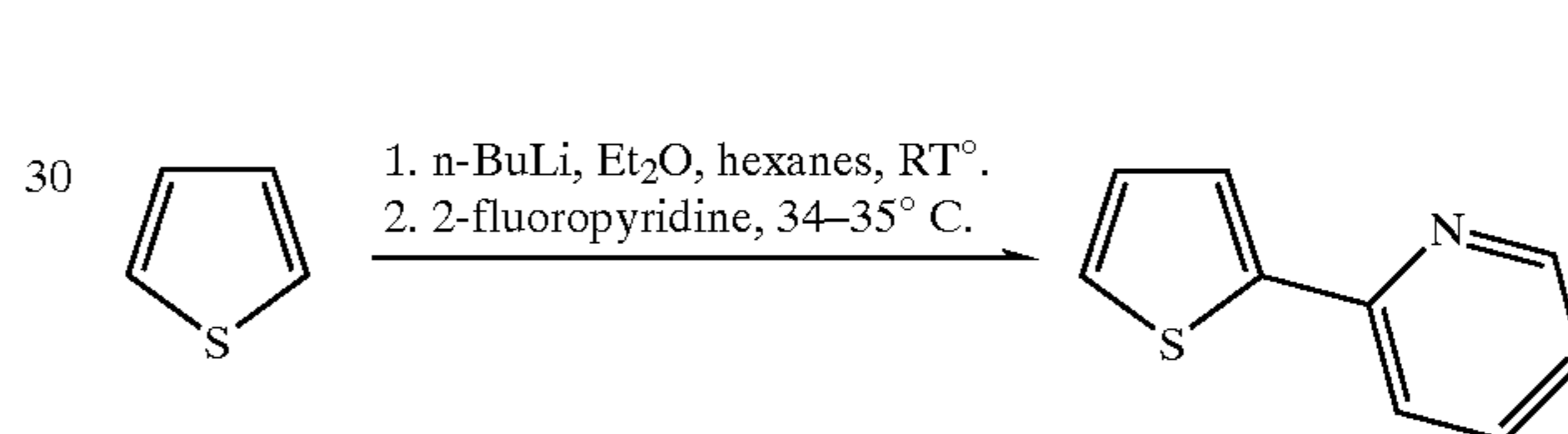
(3) Scheme 2: Synthesis of 2-(2-thienyl)pyridine.
