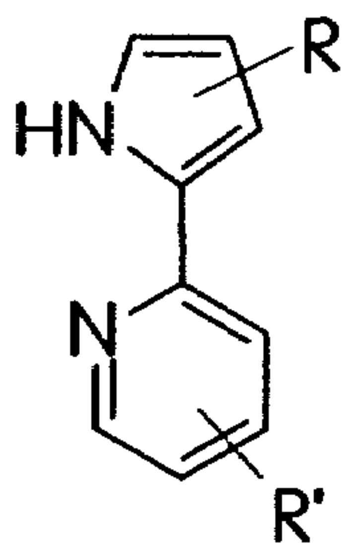
pyridylpyroles
