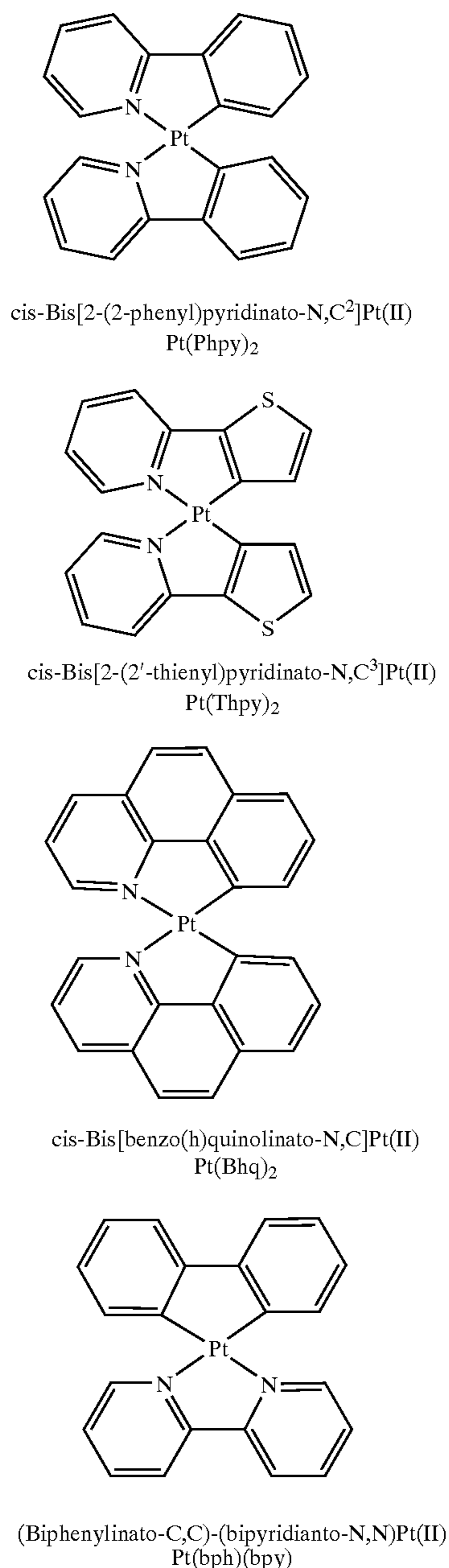
Scheme 1: Explanations for abbreviations used in table 1.
