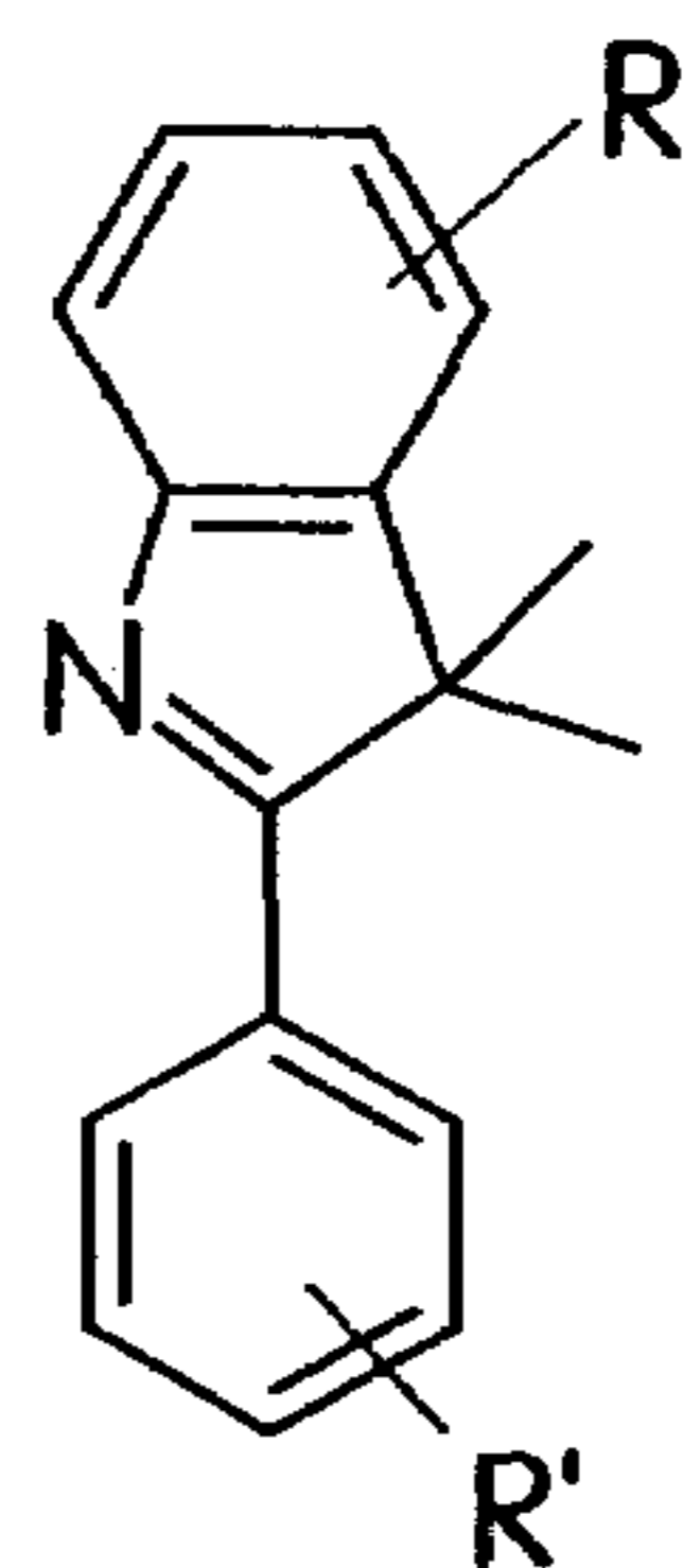
phenylindoles
