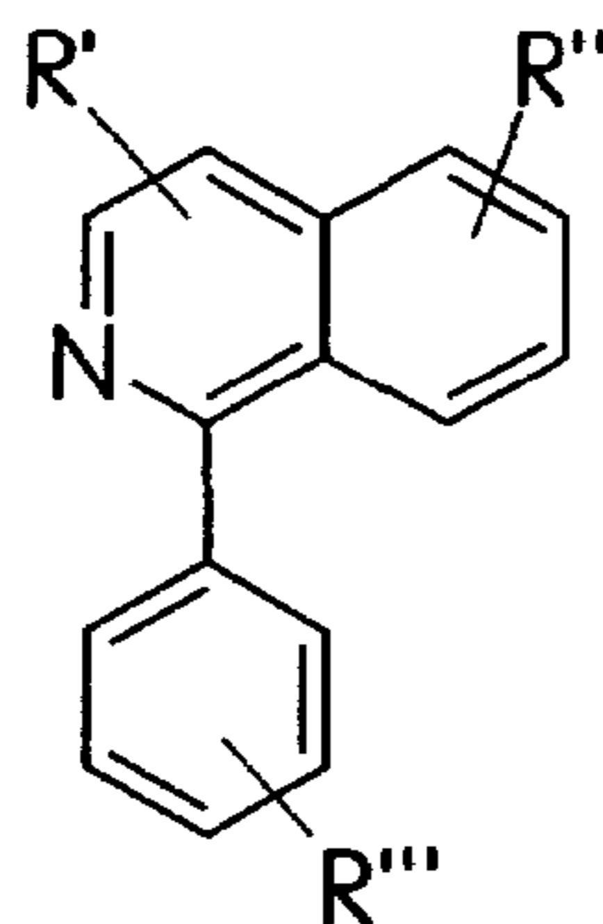
arylquinolines
