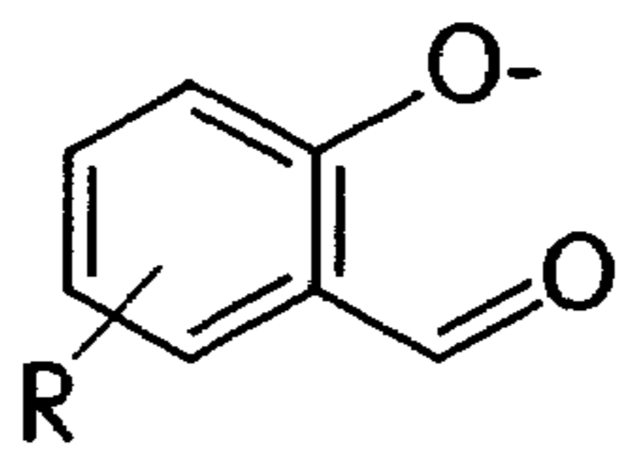
salicylaldehydes
