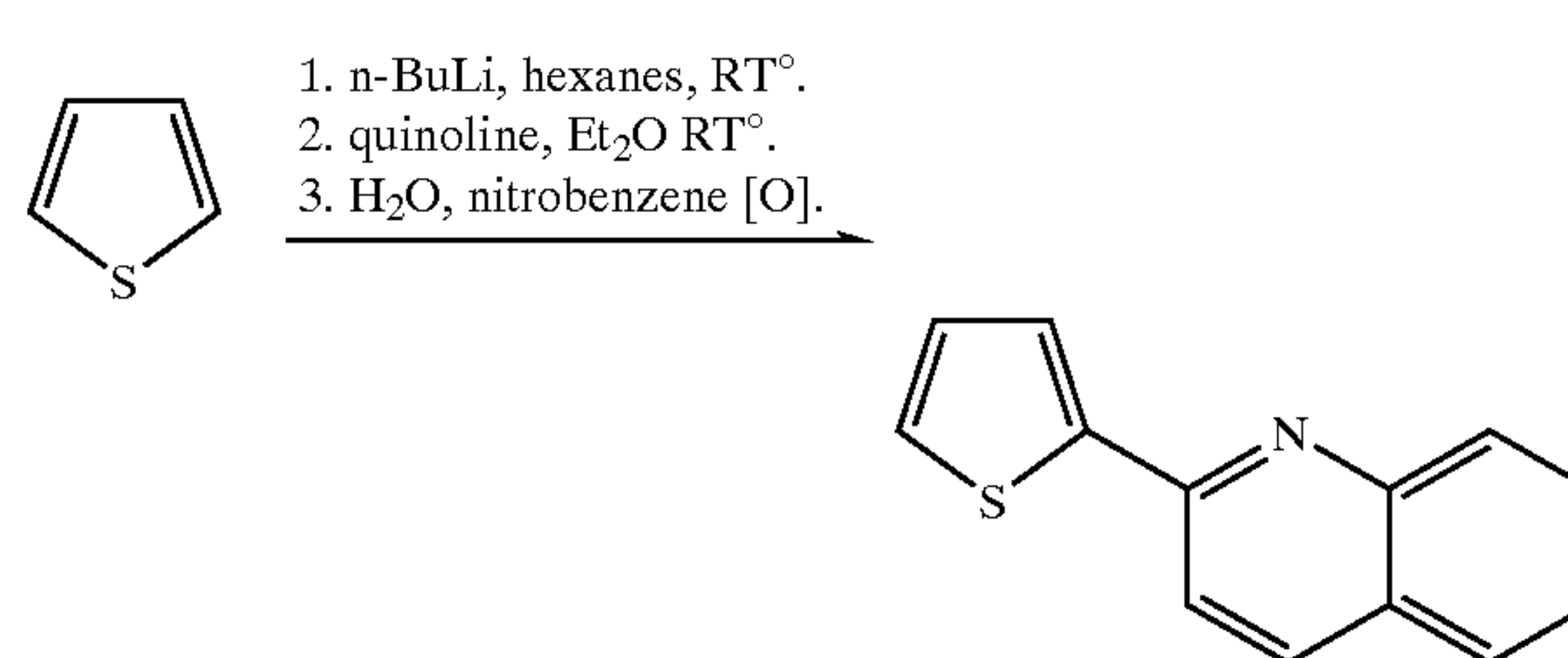
Scheme 3: Synthesis of 2-(2-thienyl)quinoline.
