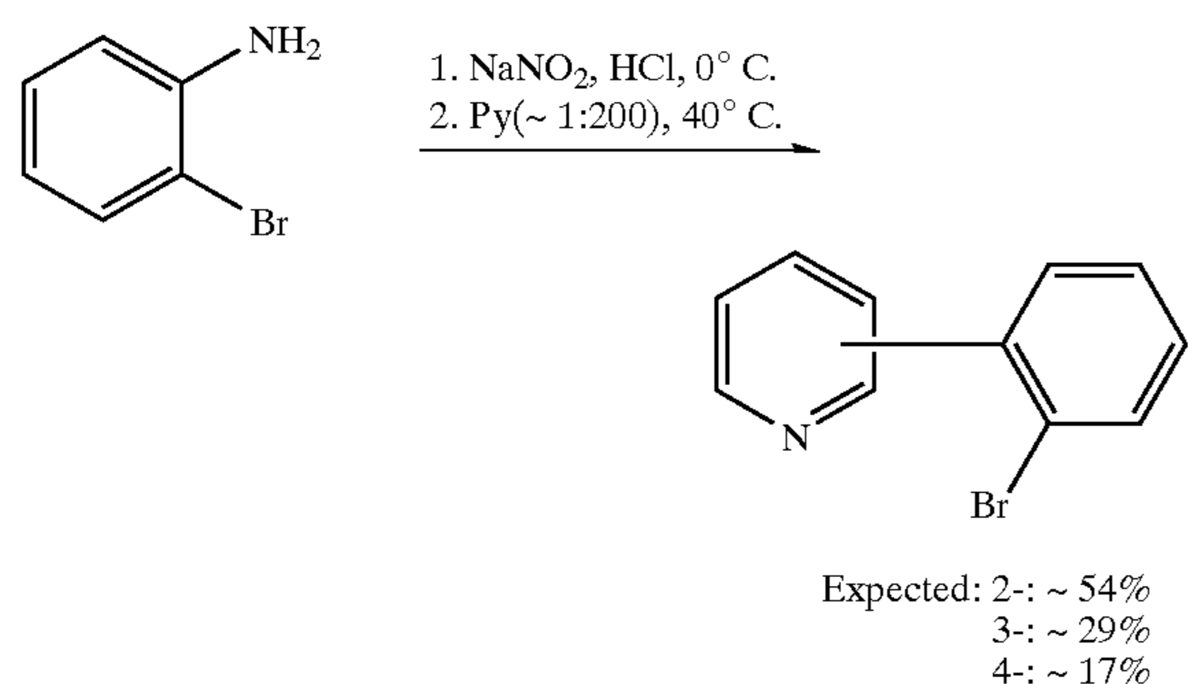
Scheme 4: Synthesis of n-(2'-bromophenyl)pyridines.
