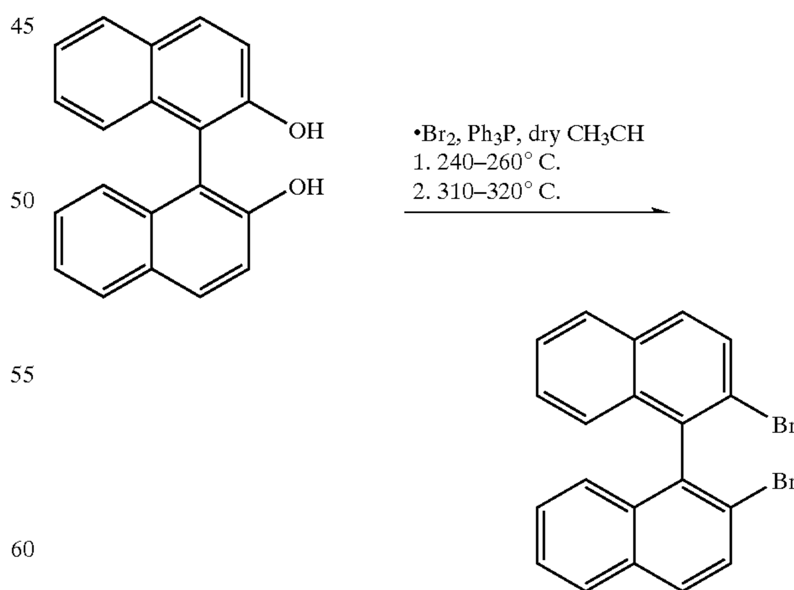
Scheme 7: Synthesis of 2,2'-dibromo-1,1'-binaphthyl.
