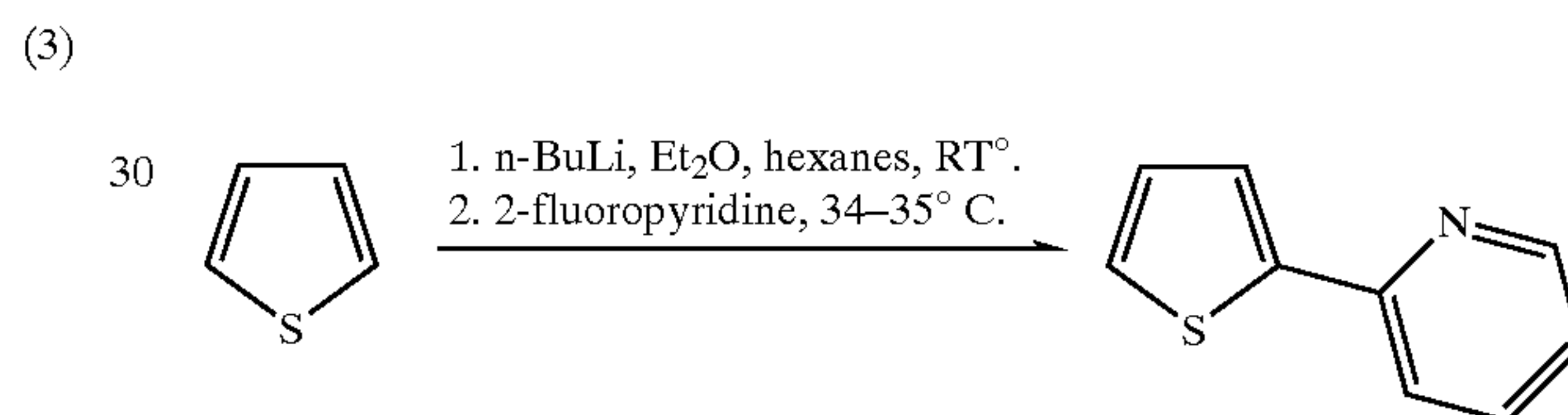
Scheme 2: Synthesis of 2-(2-thienyl)pyridine.
