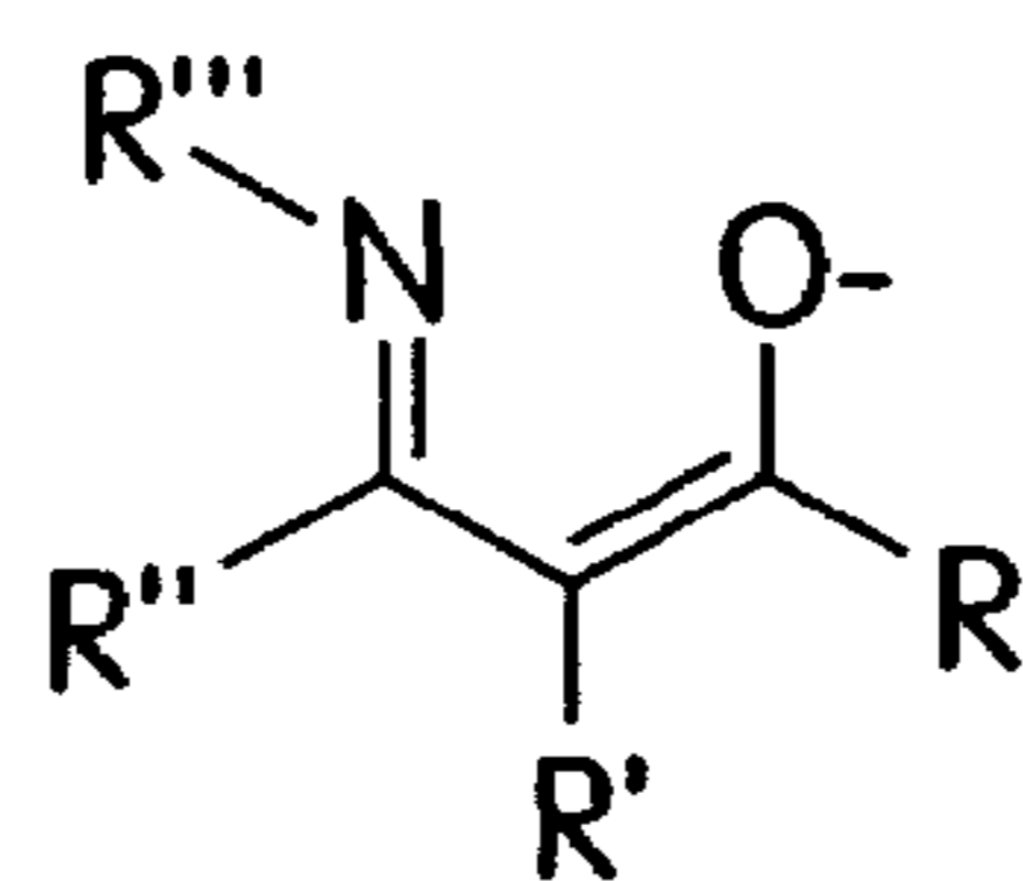
iminoacetates
