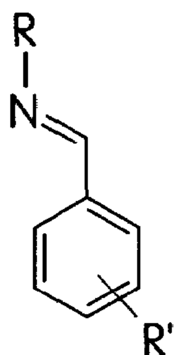
phenylimines
