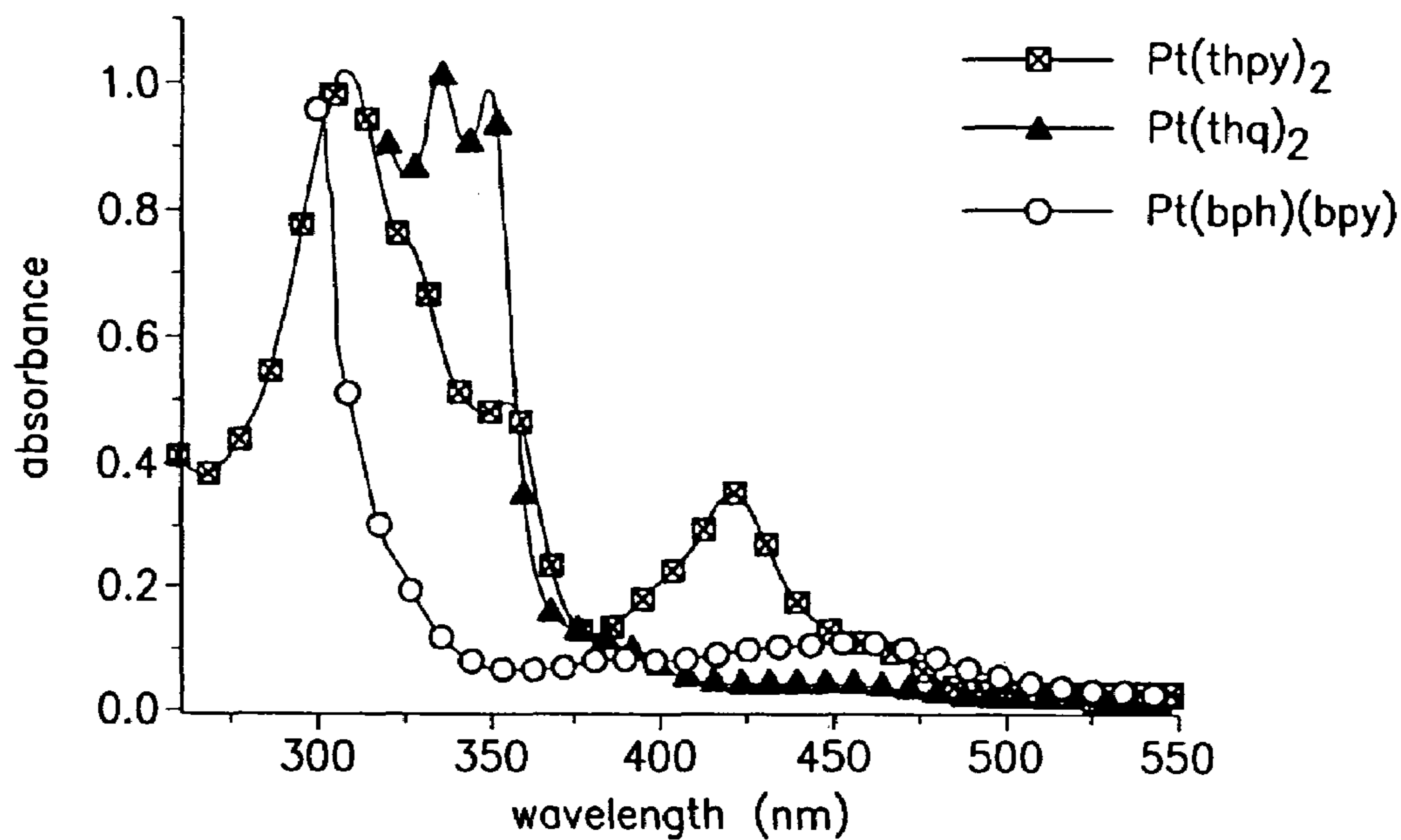
Electronic absorbance spectra of Pt(thpy) 2 , Pt(thq) 2 , Pt(bph)(bpy).
