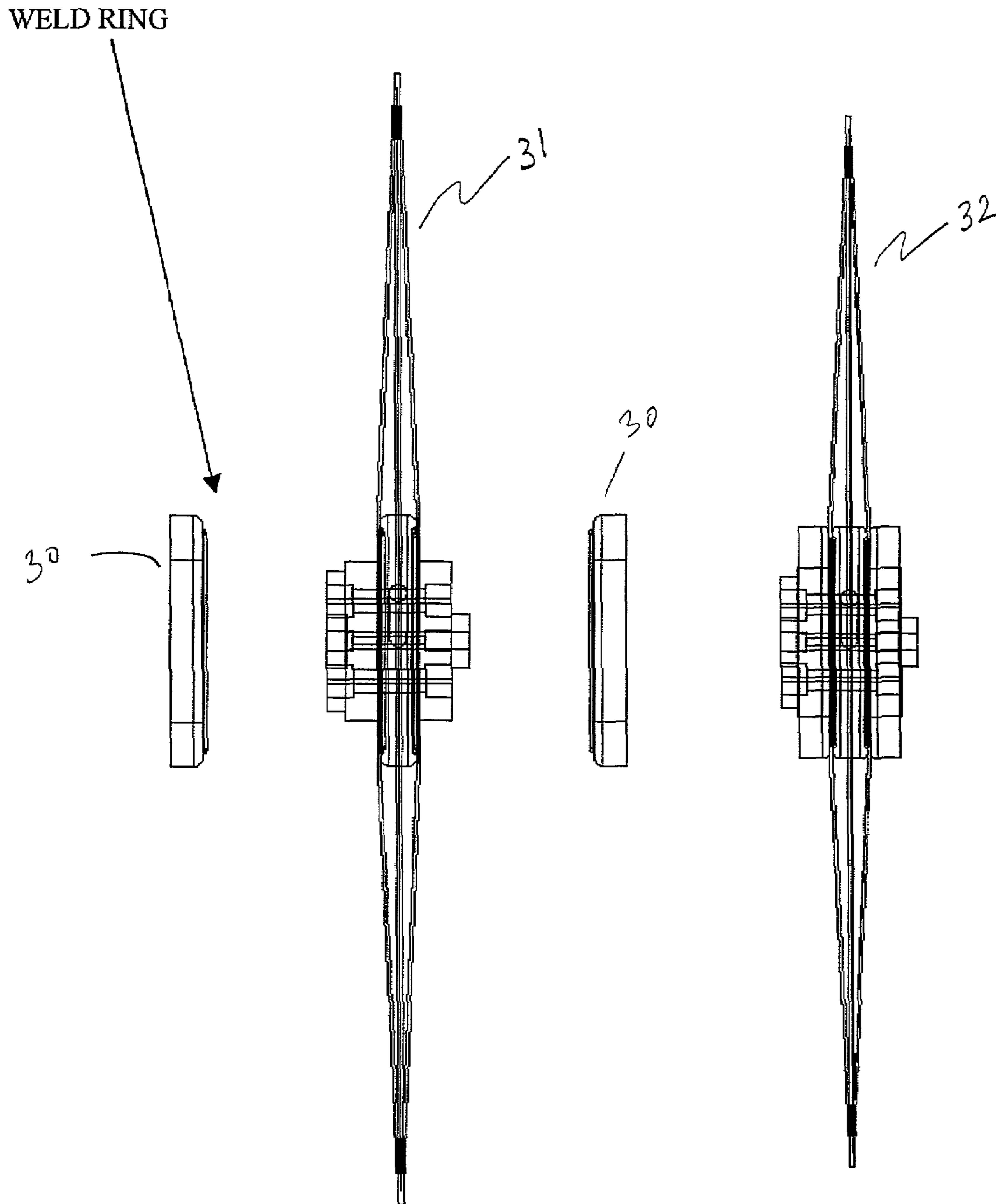
FIGURE 3 EXPRESSOR BAG ASSEMBLY
