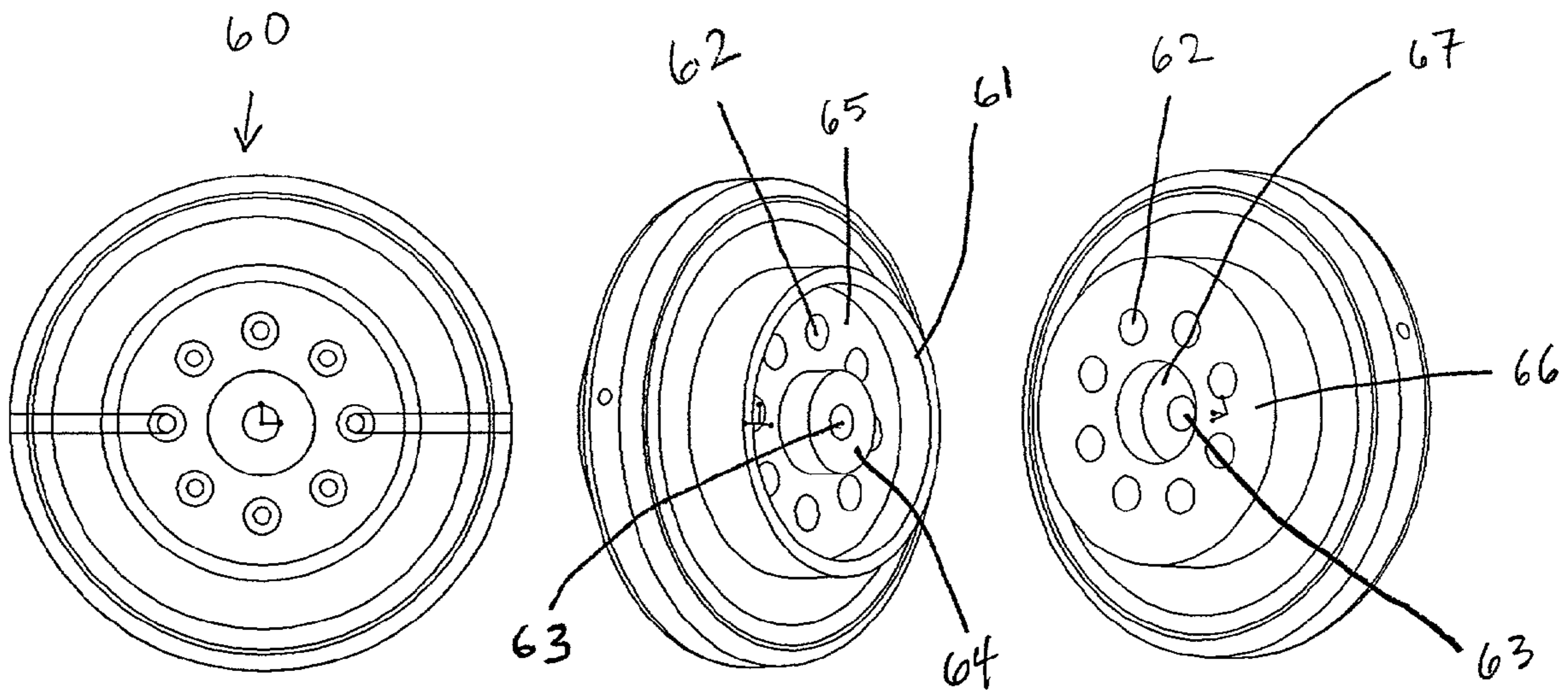
FIGURE 6 PROCESSING CENTRAL HUB
