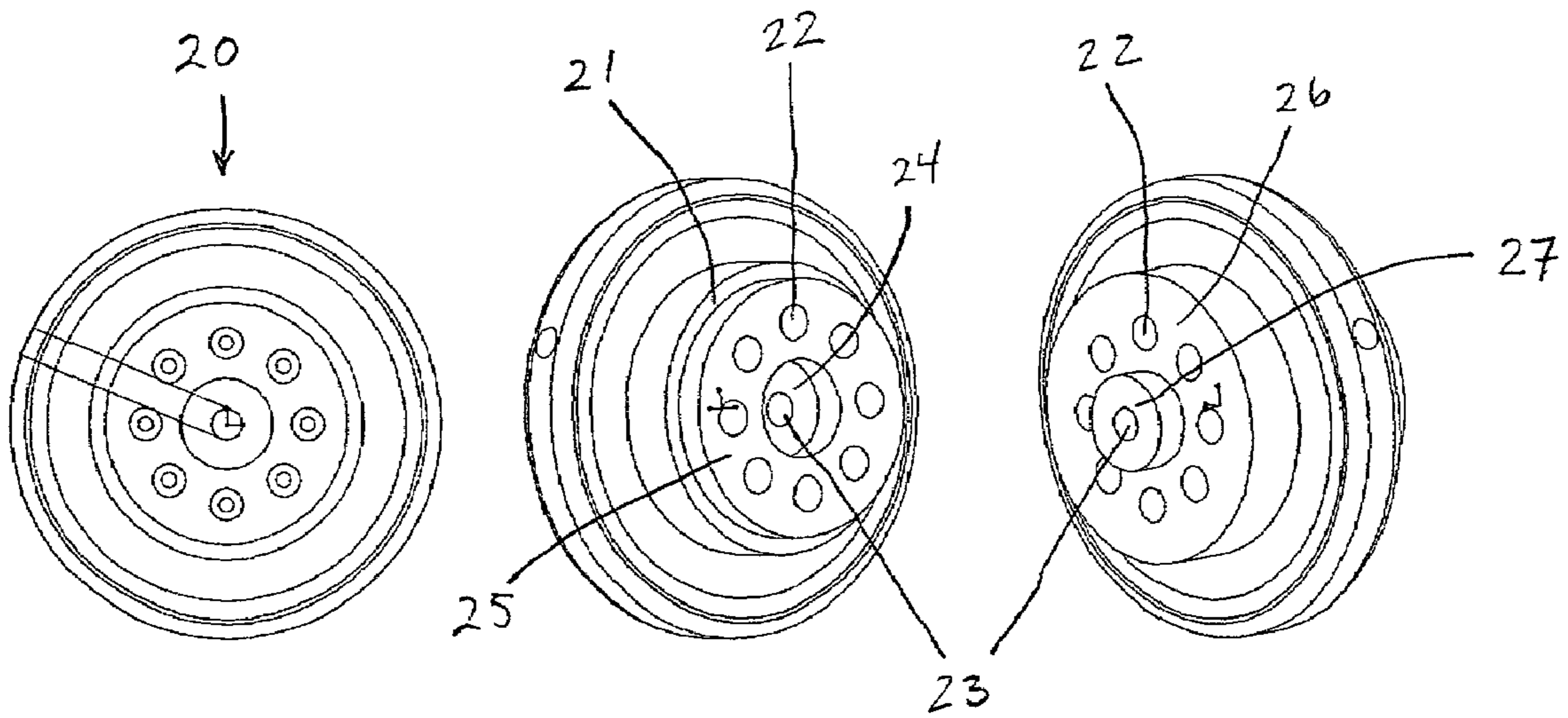
FIGURE 2 EXPRESSOR CENTRAL HUB
