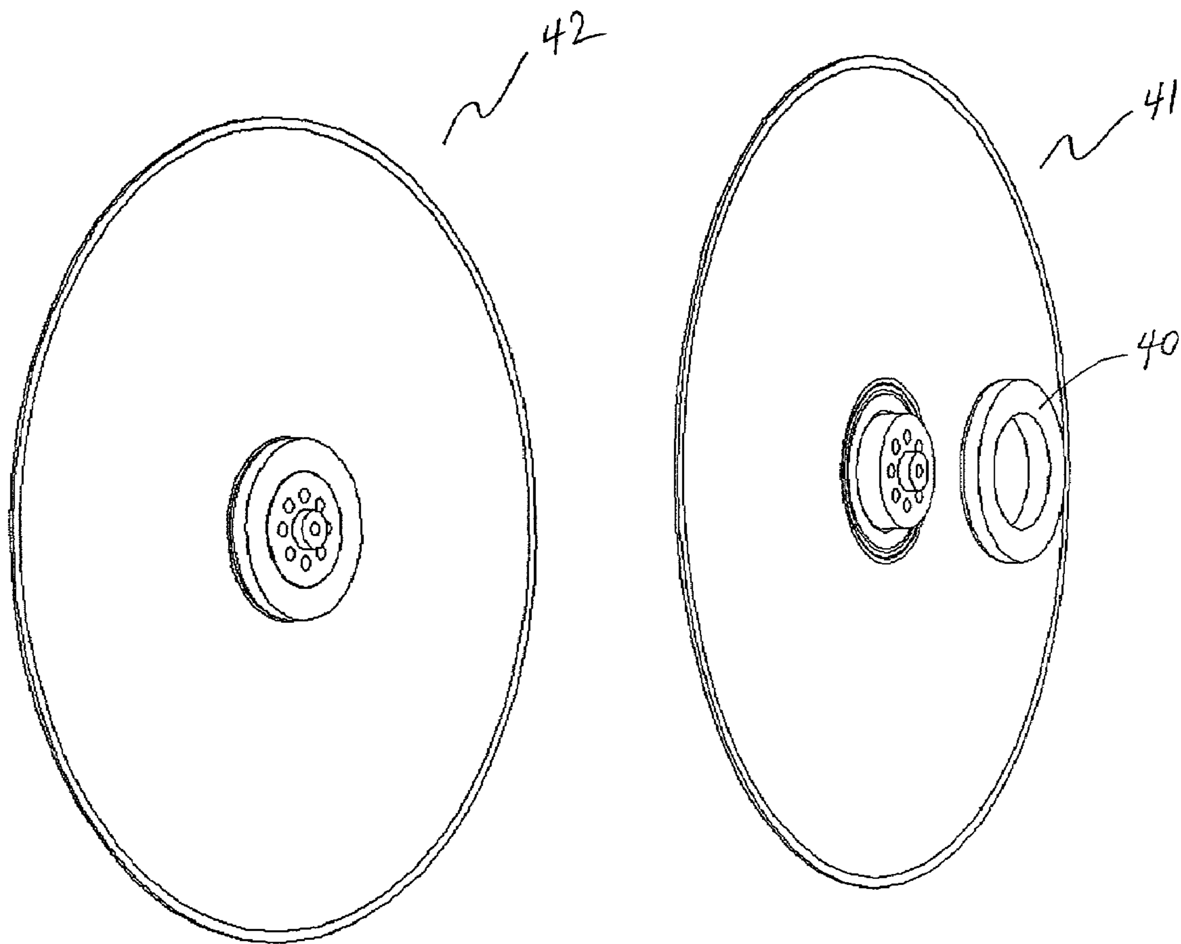
FIGURE 4 EXPRESSOR BAG ASSEMBLY
