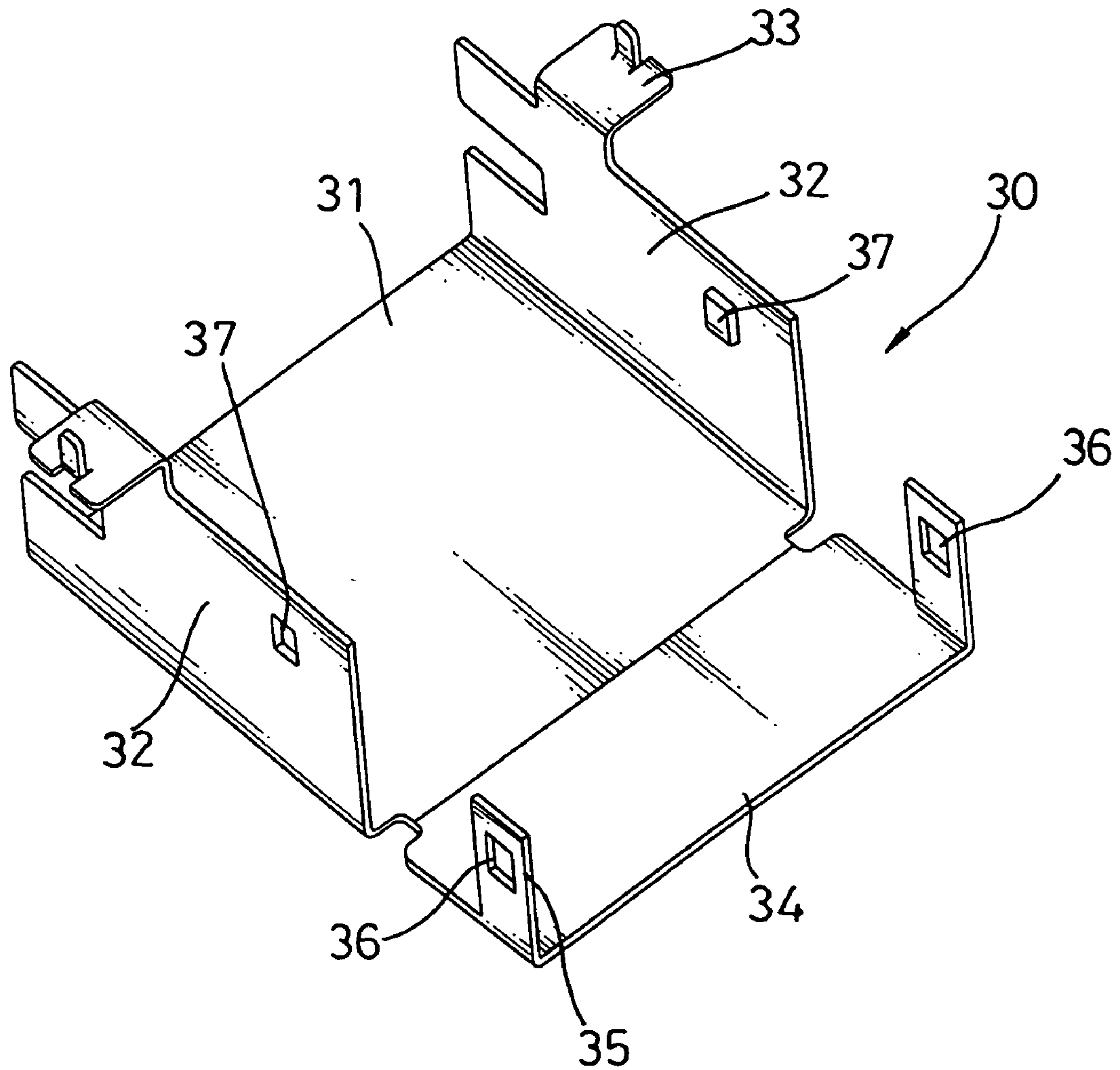
FIG. 4 PRIOR ART
