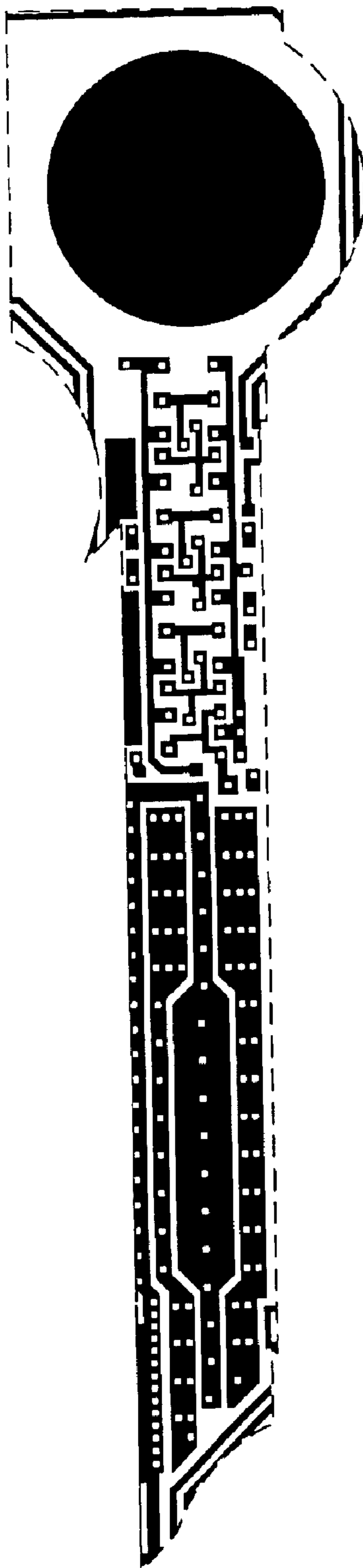
Metal 1 mask
