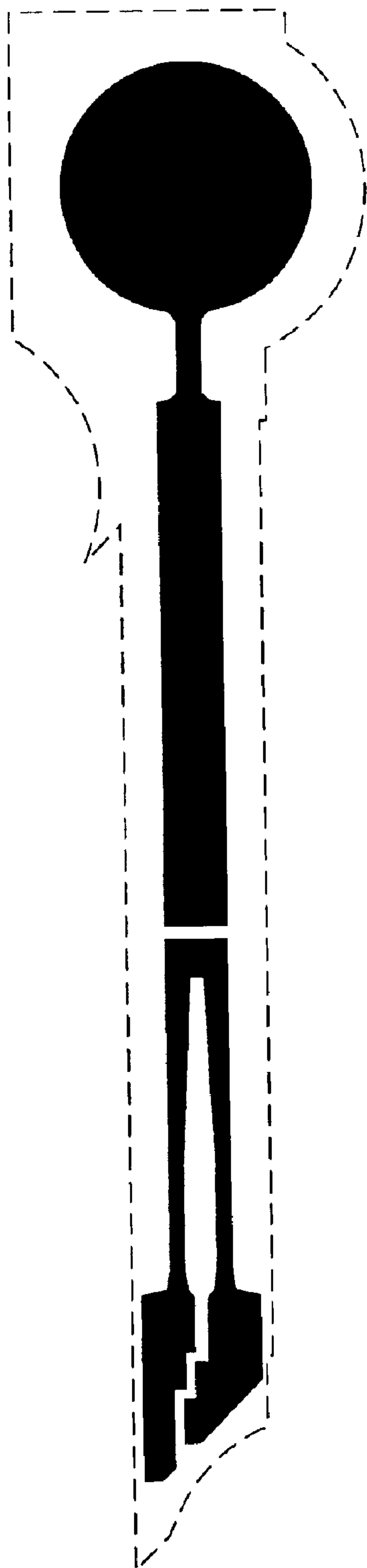
Heater mask
