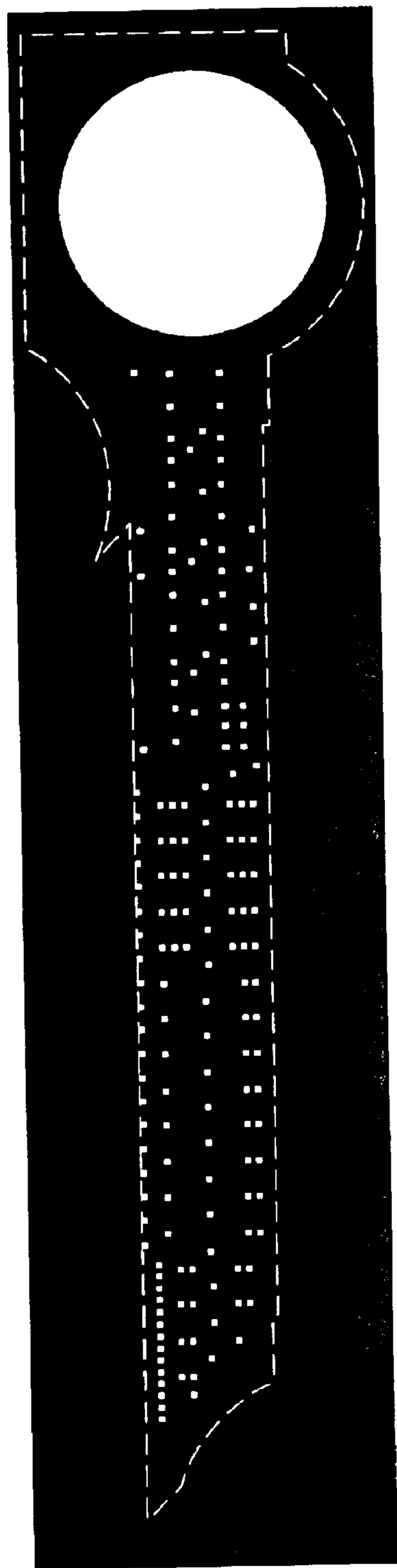
Contacts mask
