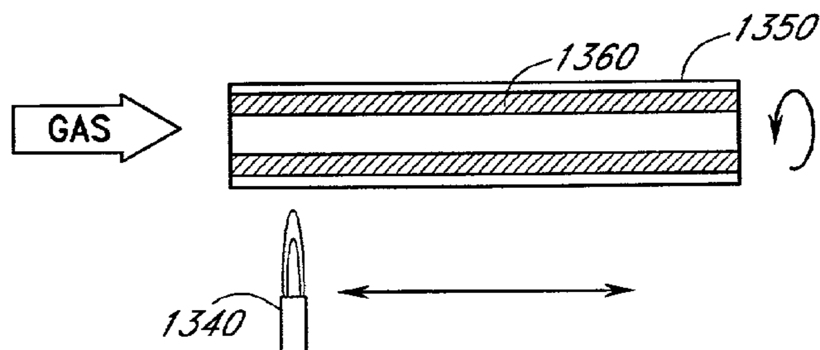
FIG. 28C (PRIOR ART)
