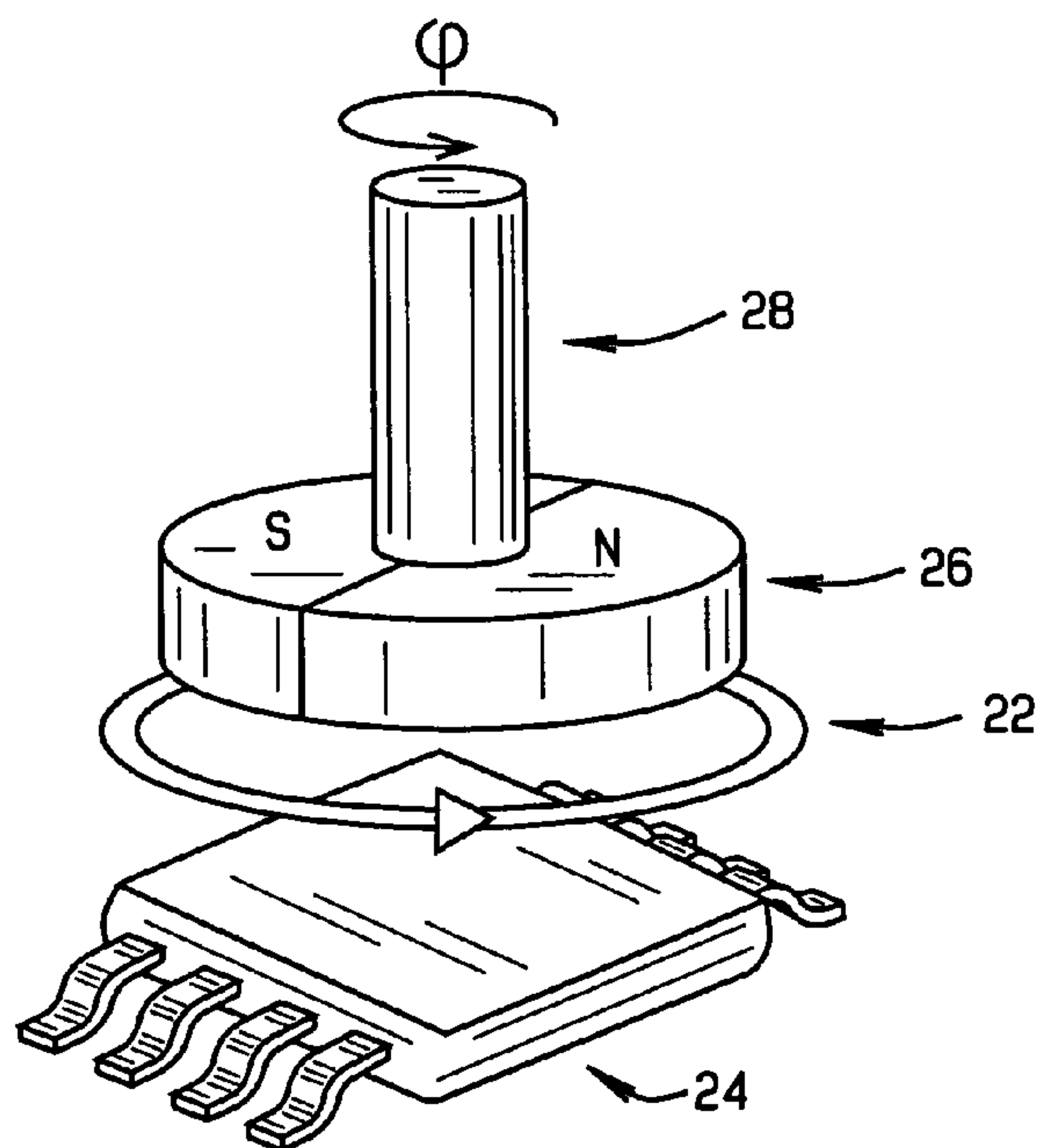
FIG. 3 PRIOR ART
