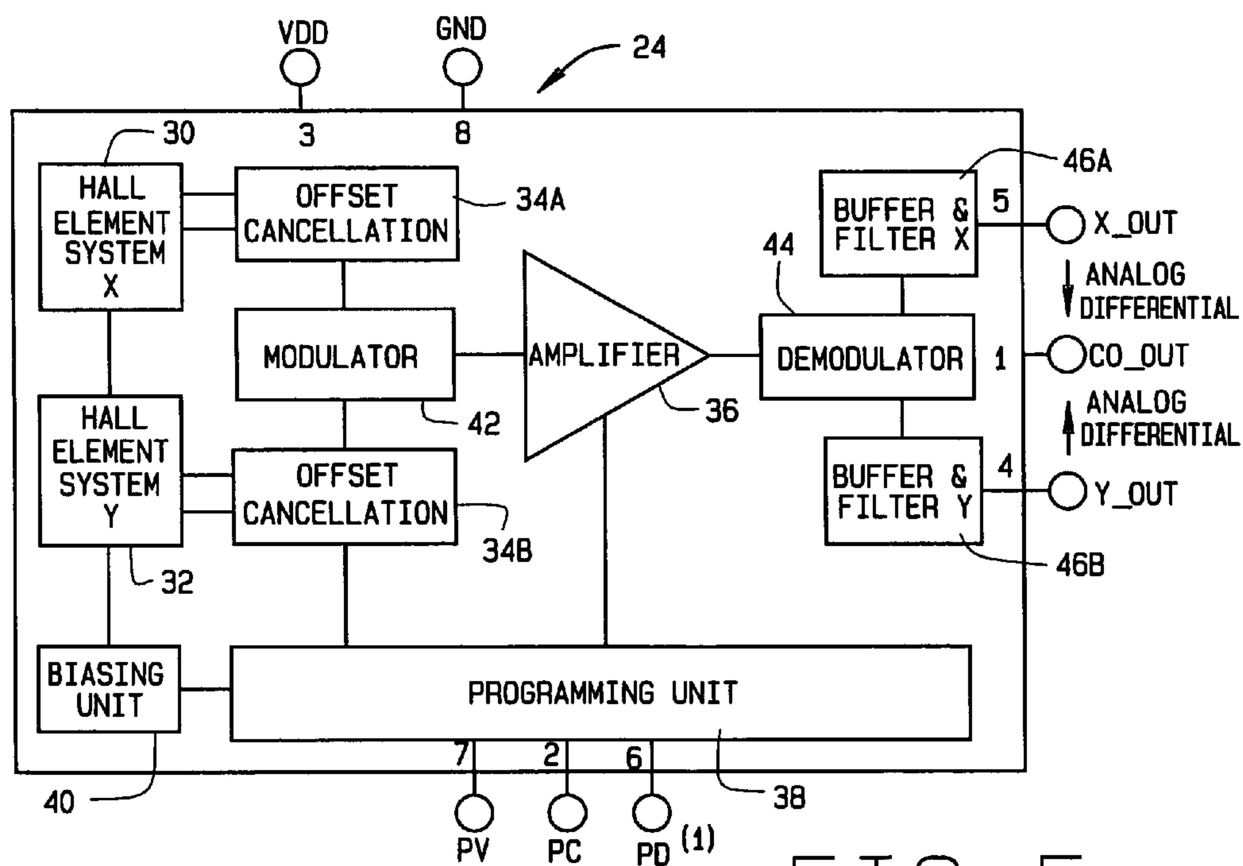
FIG. 5 PRIOR ART
