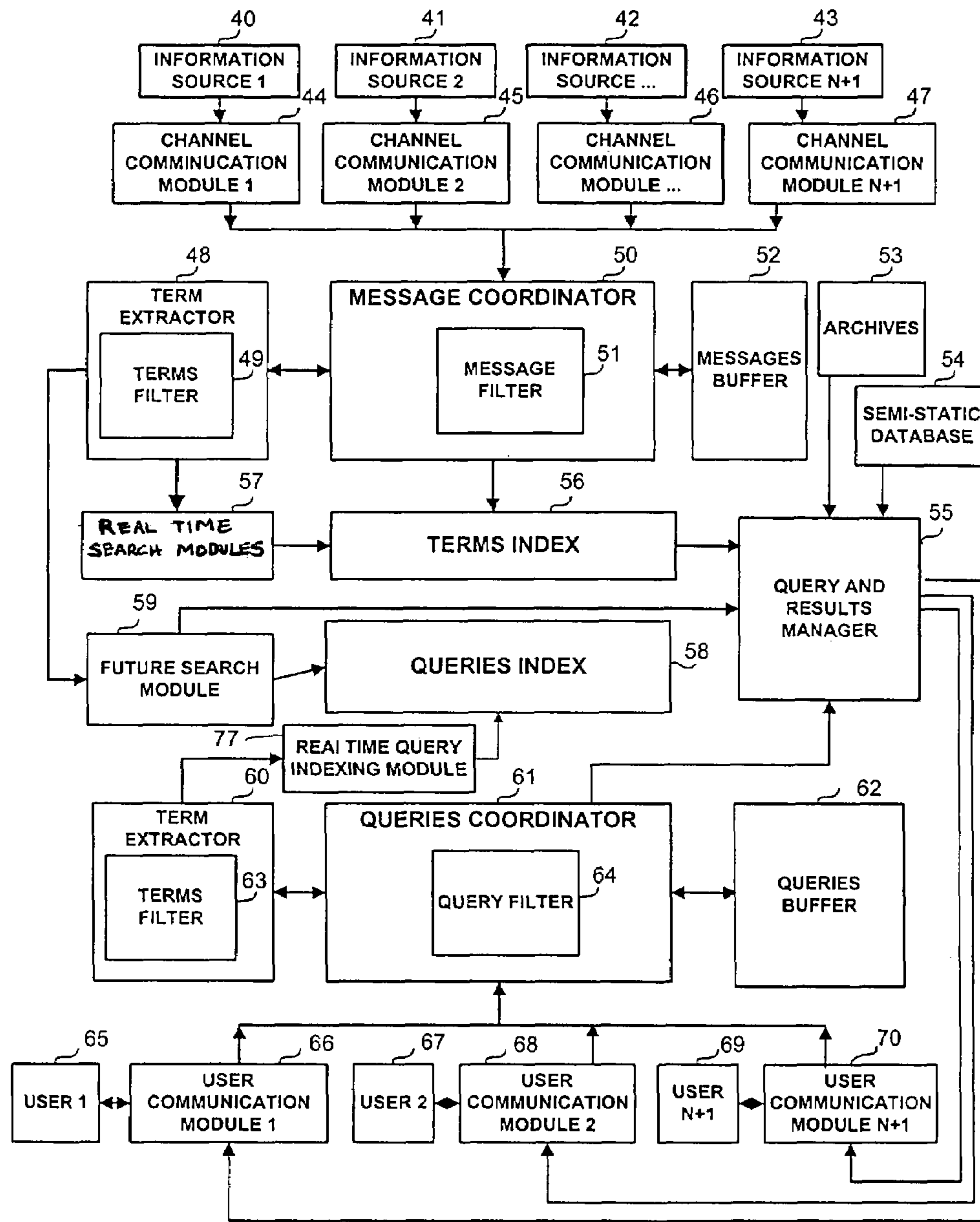
SEARCH ENGINE
