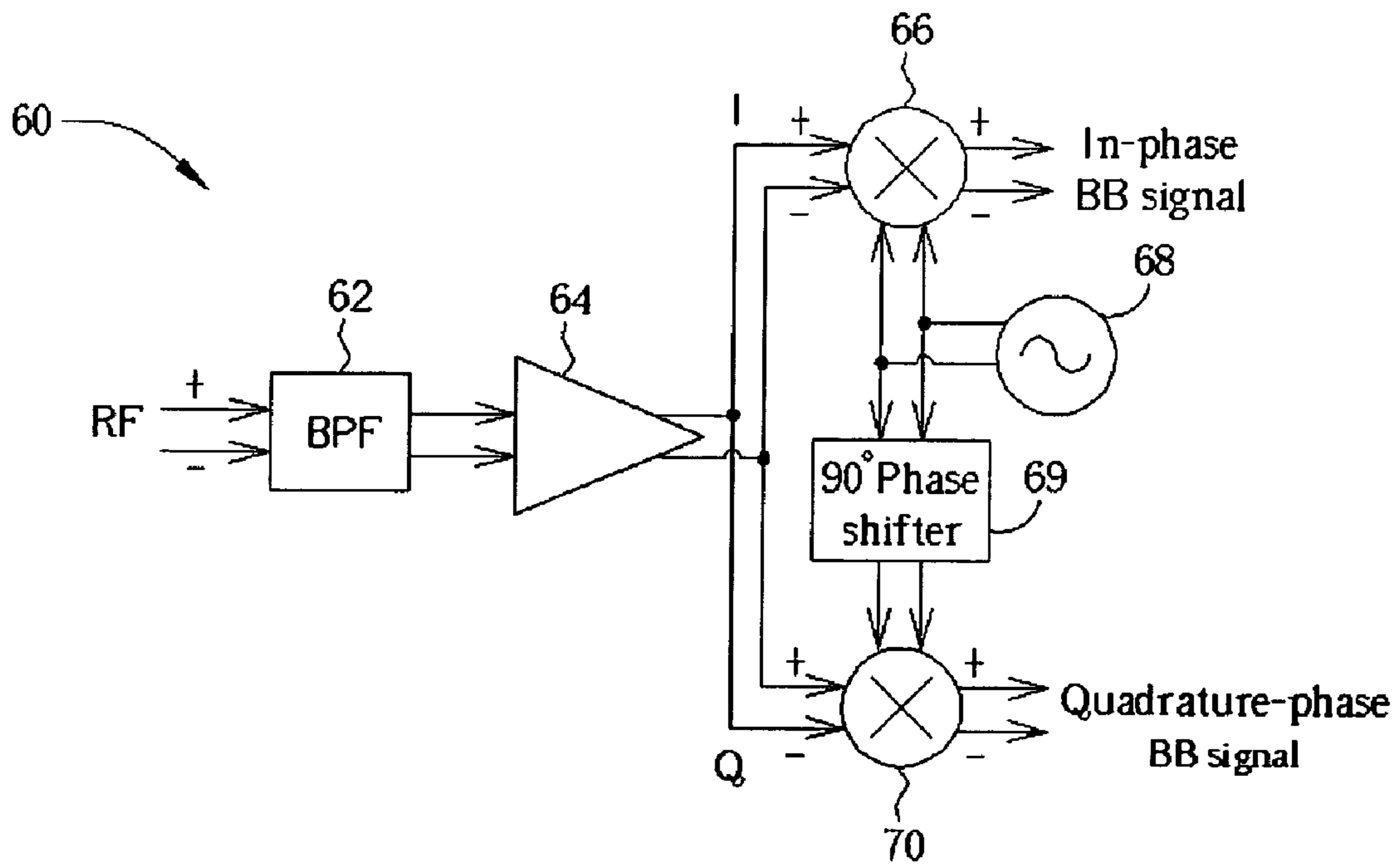
Fig. 4 Prior art
