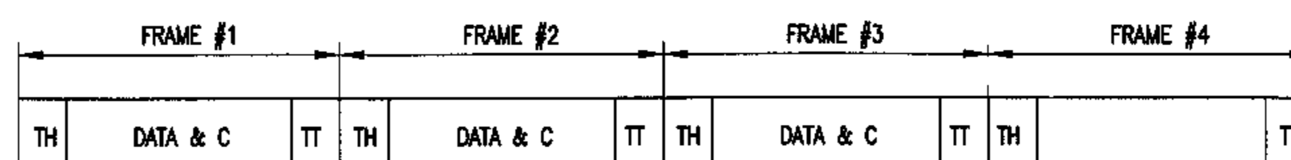
NORMAL FRAME FORMAT STREAM
