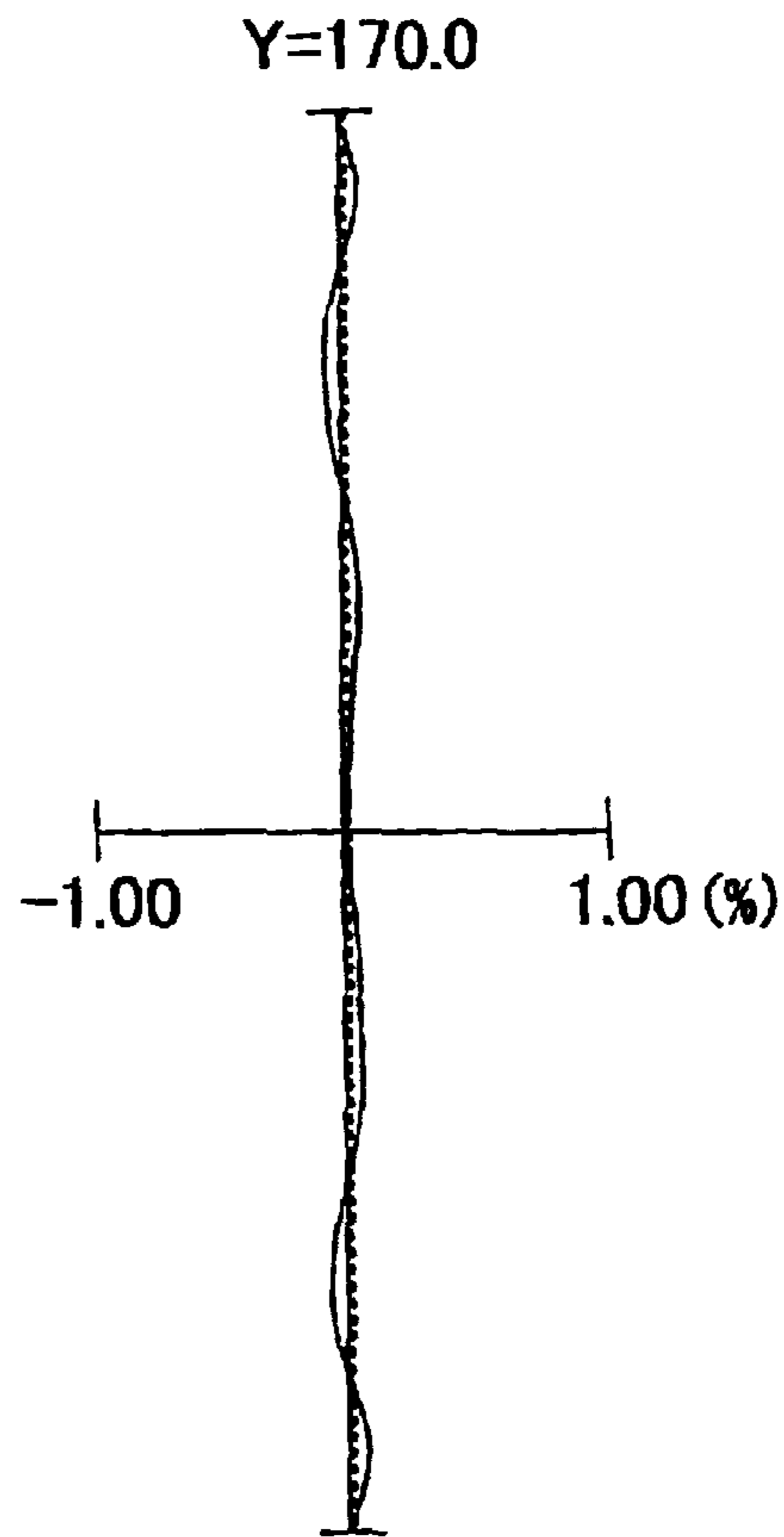
LINEARITY fθ CHARACTERISTIC
