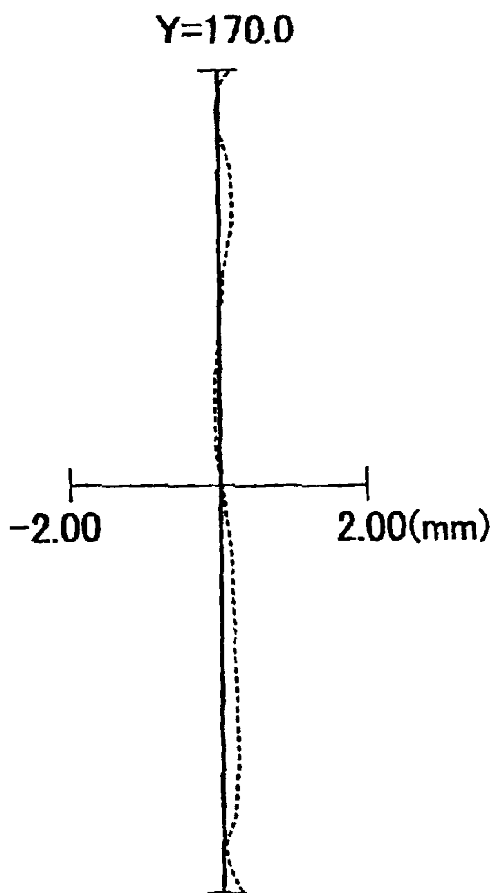
IMAGE SURFACE CURVATURE
