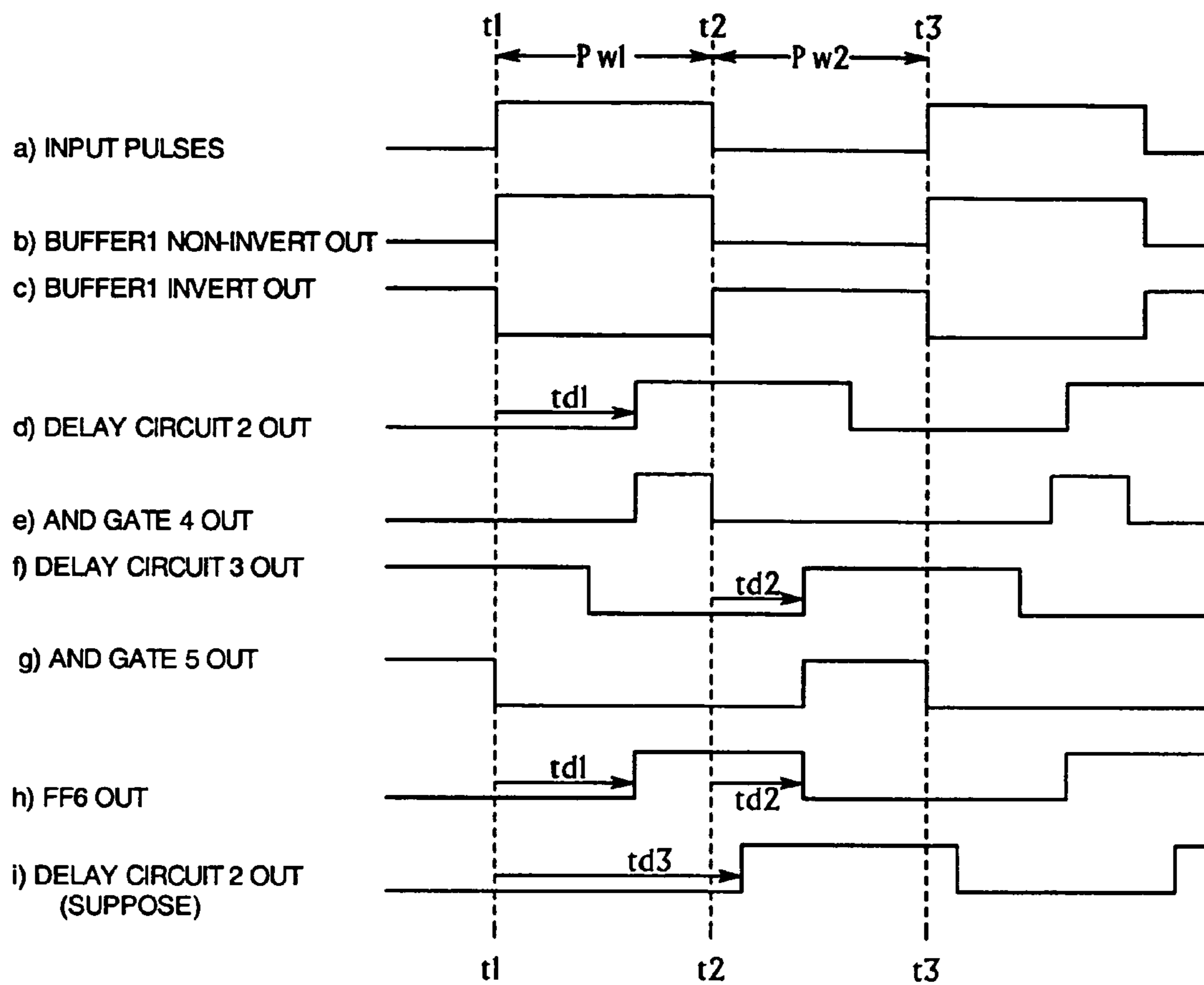
FIG. 2(Prior Art)
