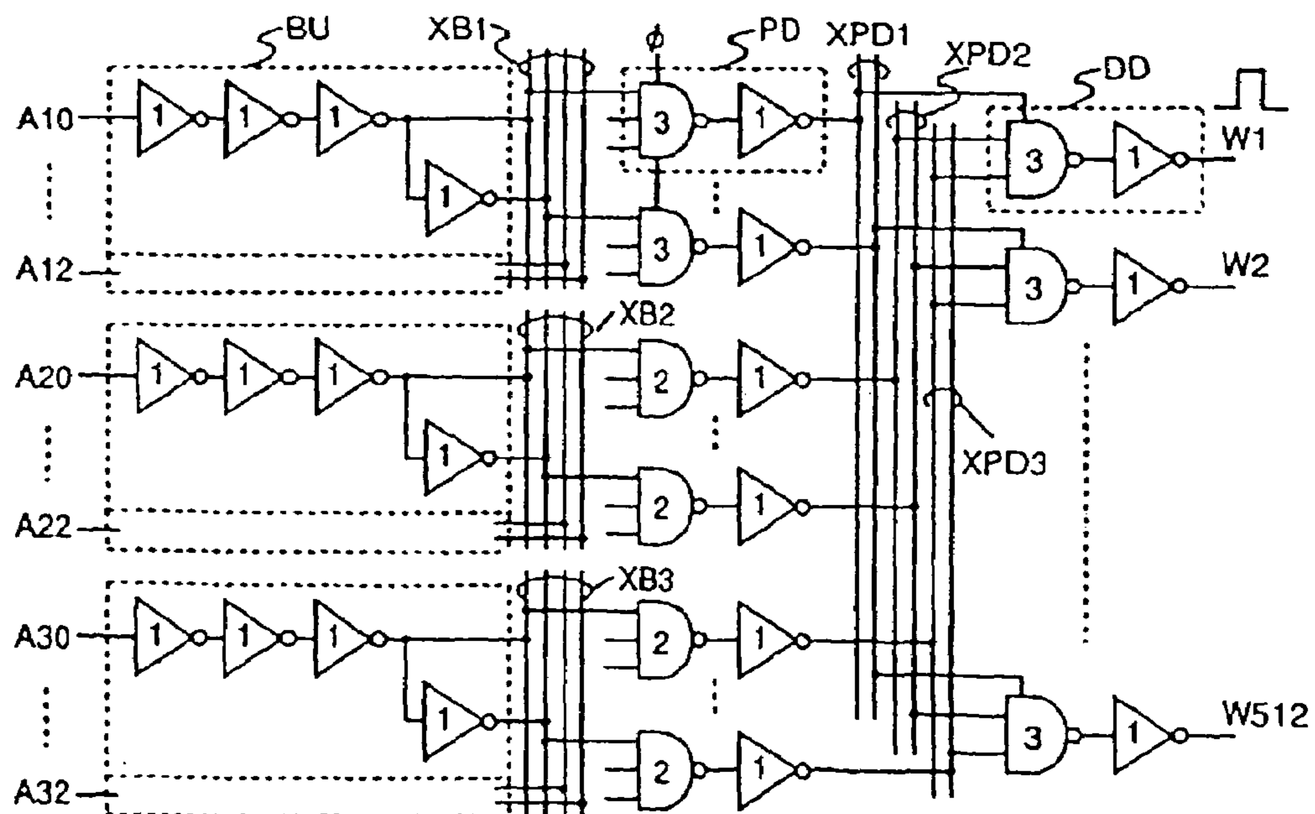
FIG. 16 PRIOR ART
