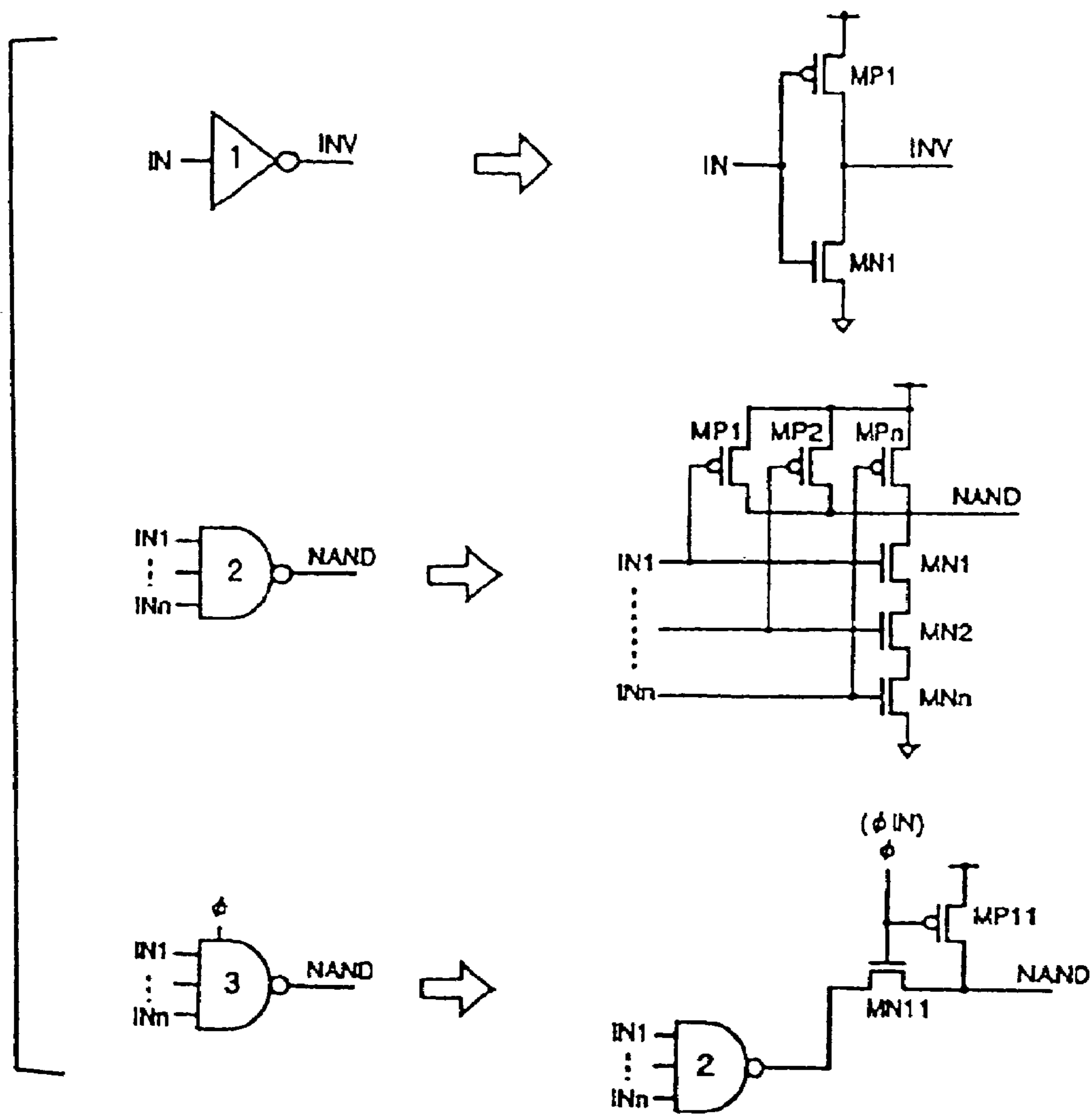
FIG. 17 PRIOR ART
