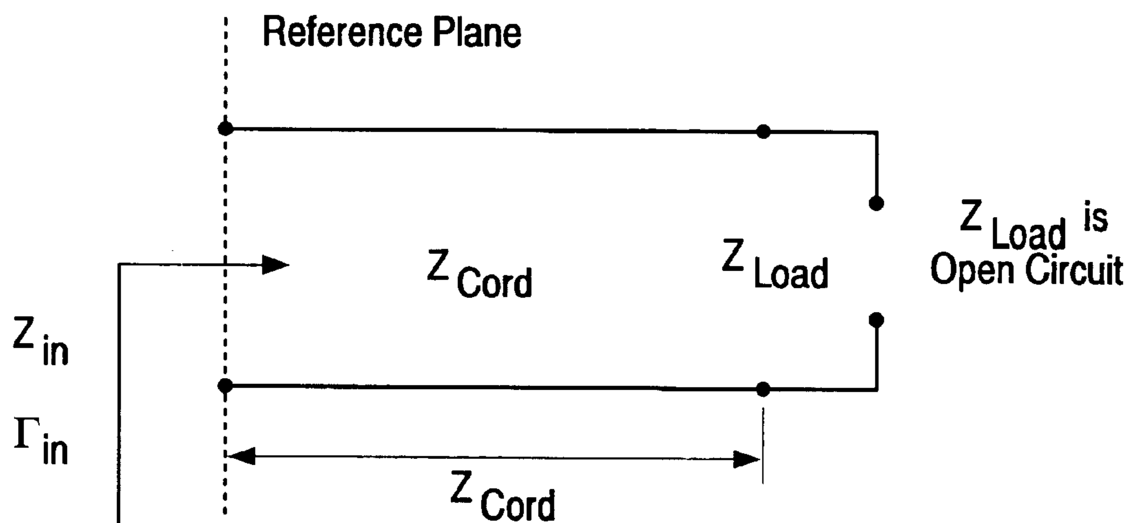
Fig. 23 Patch Cord with Open-Circuit Load
