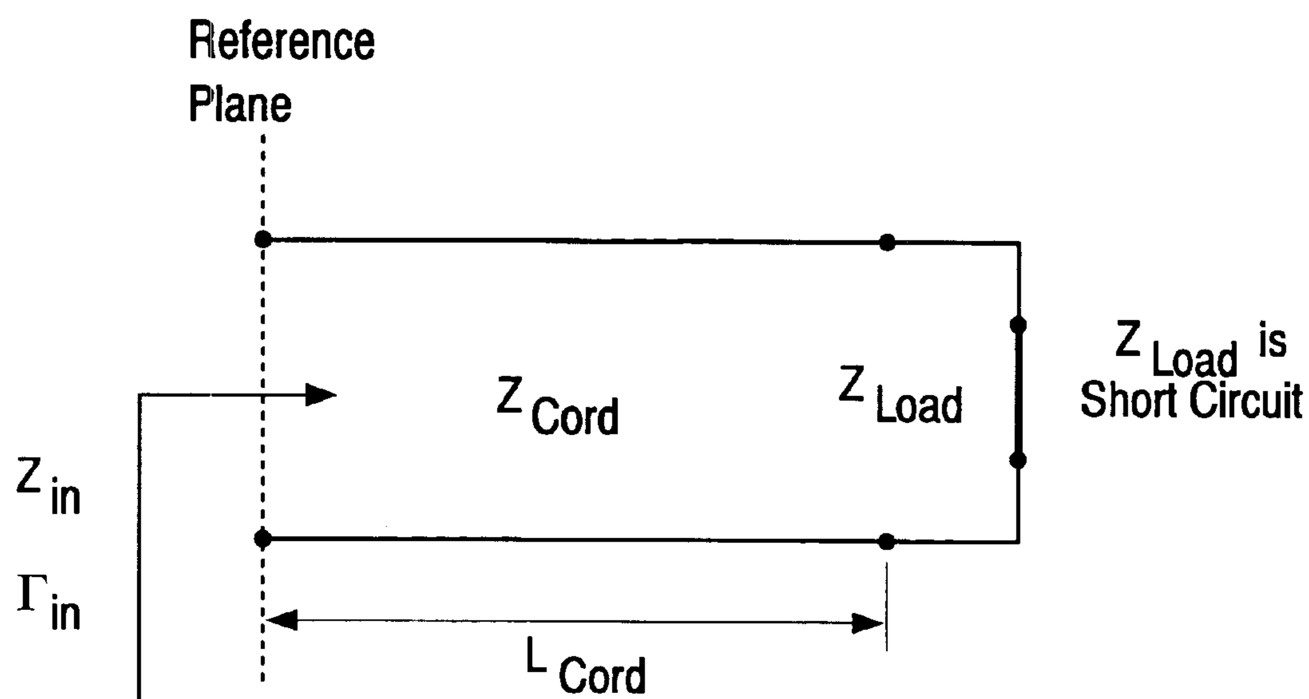
Fig. 22 Patch Cord with Short-Circuit Load
