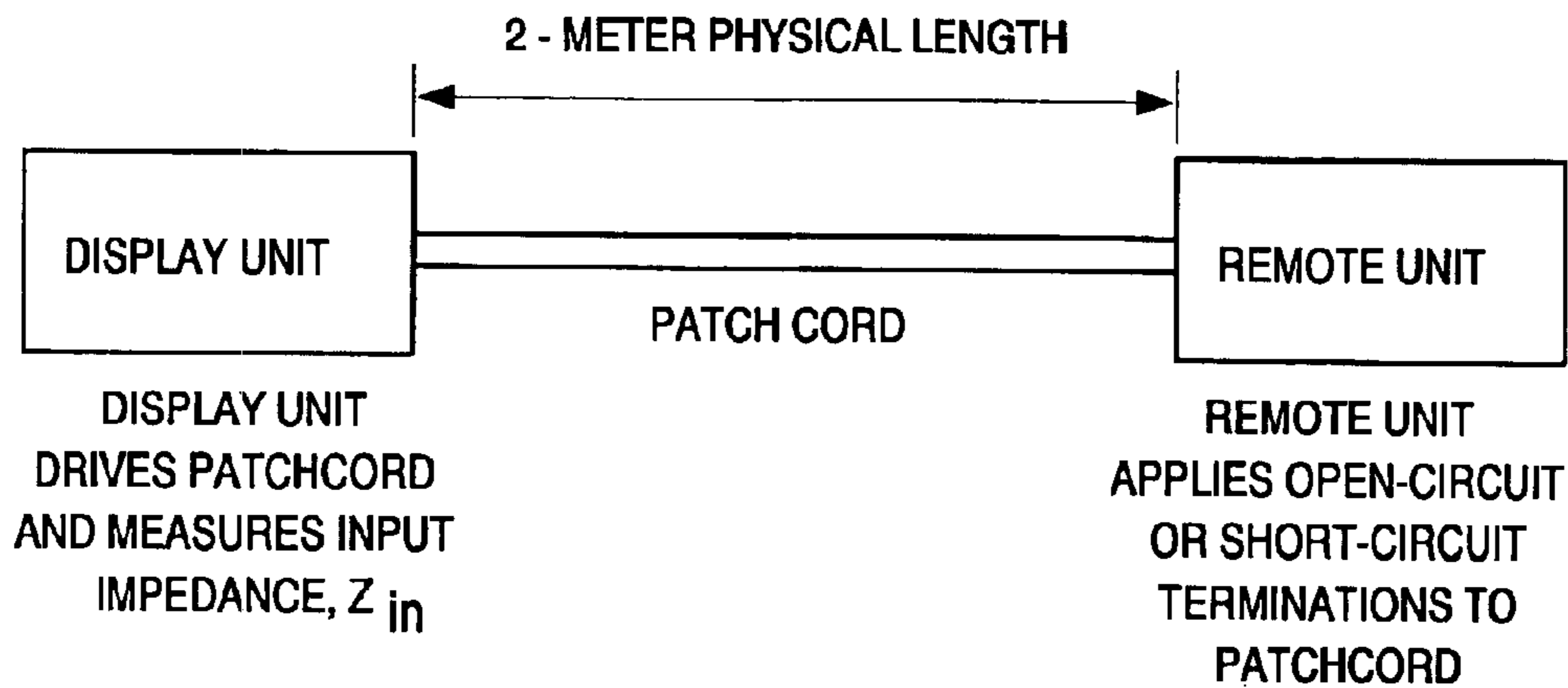
Fig. 24 PATCHCORD PHYSICAL LENGTH MEASUREMENT TEST CONFIGURATION
