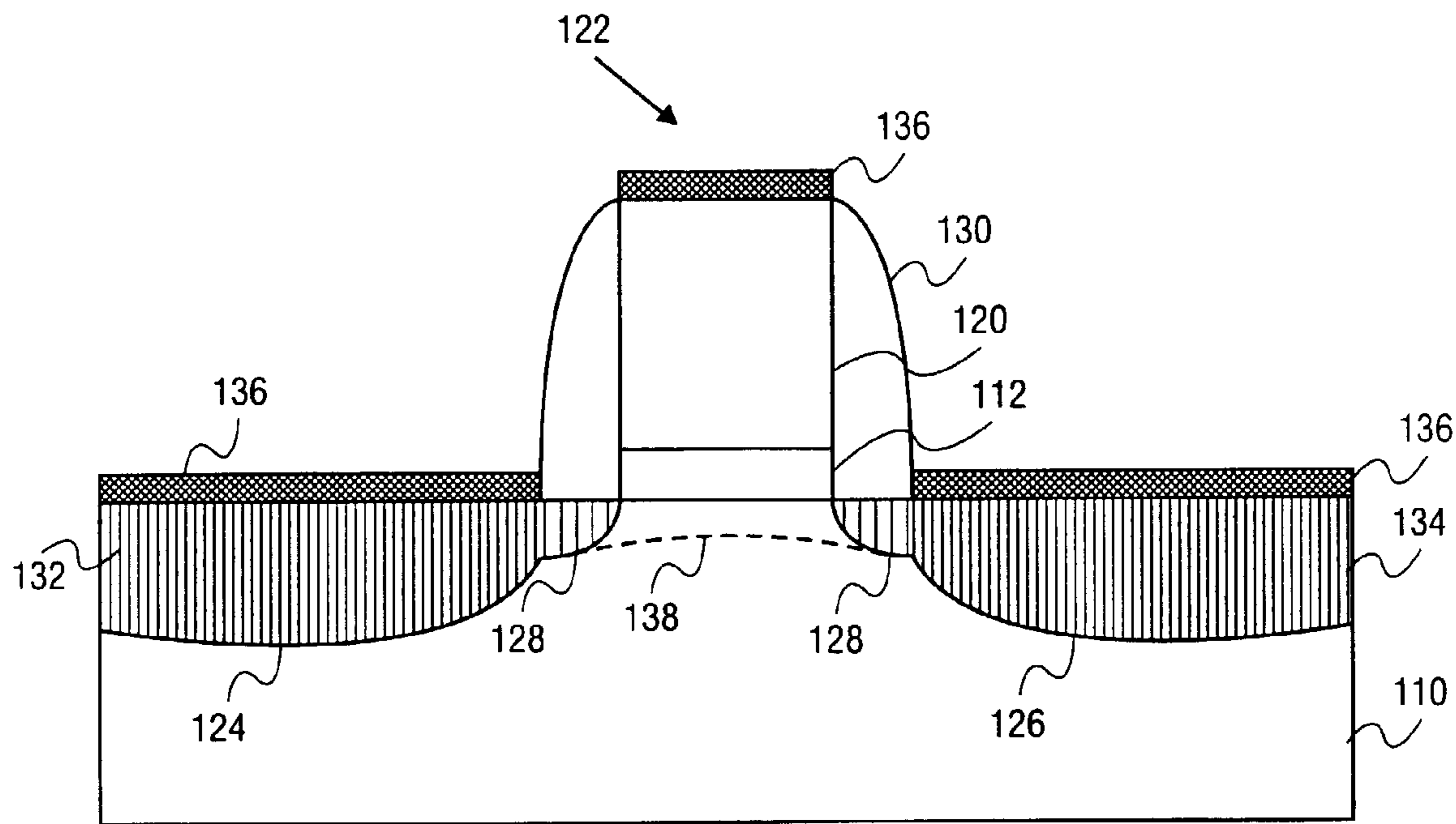
FIG. 1 (PRIOR ART)
