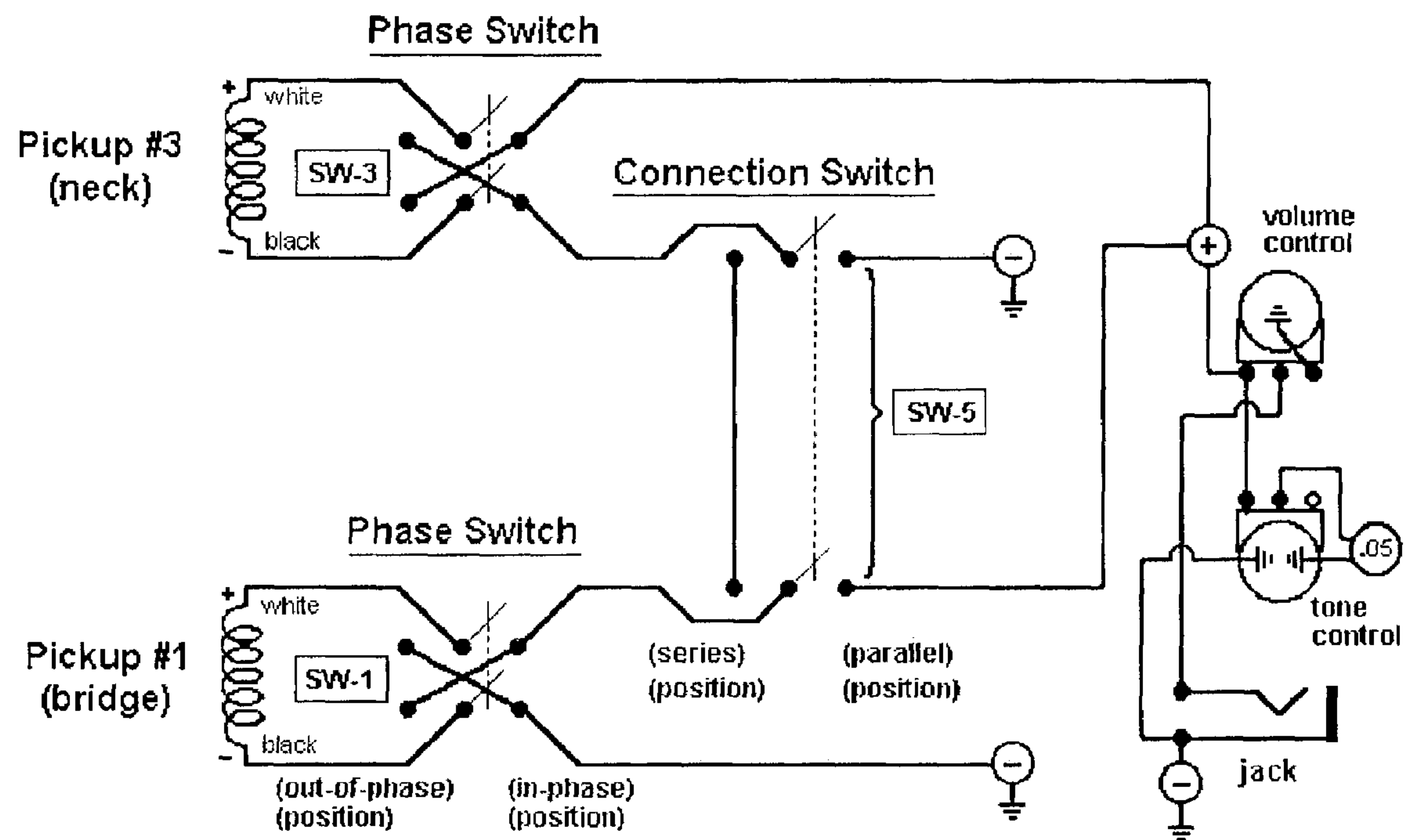
FIG. 3 - Revised Schematic For 2-Pickups
