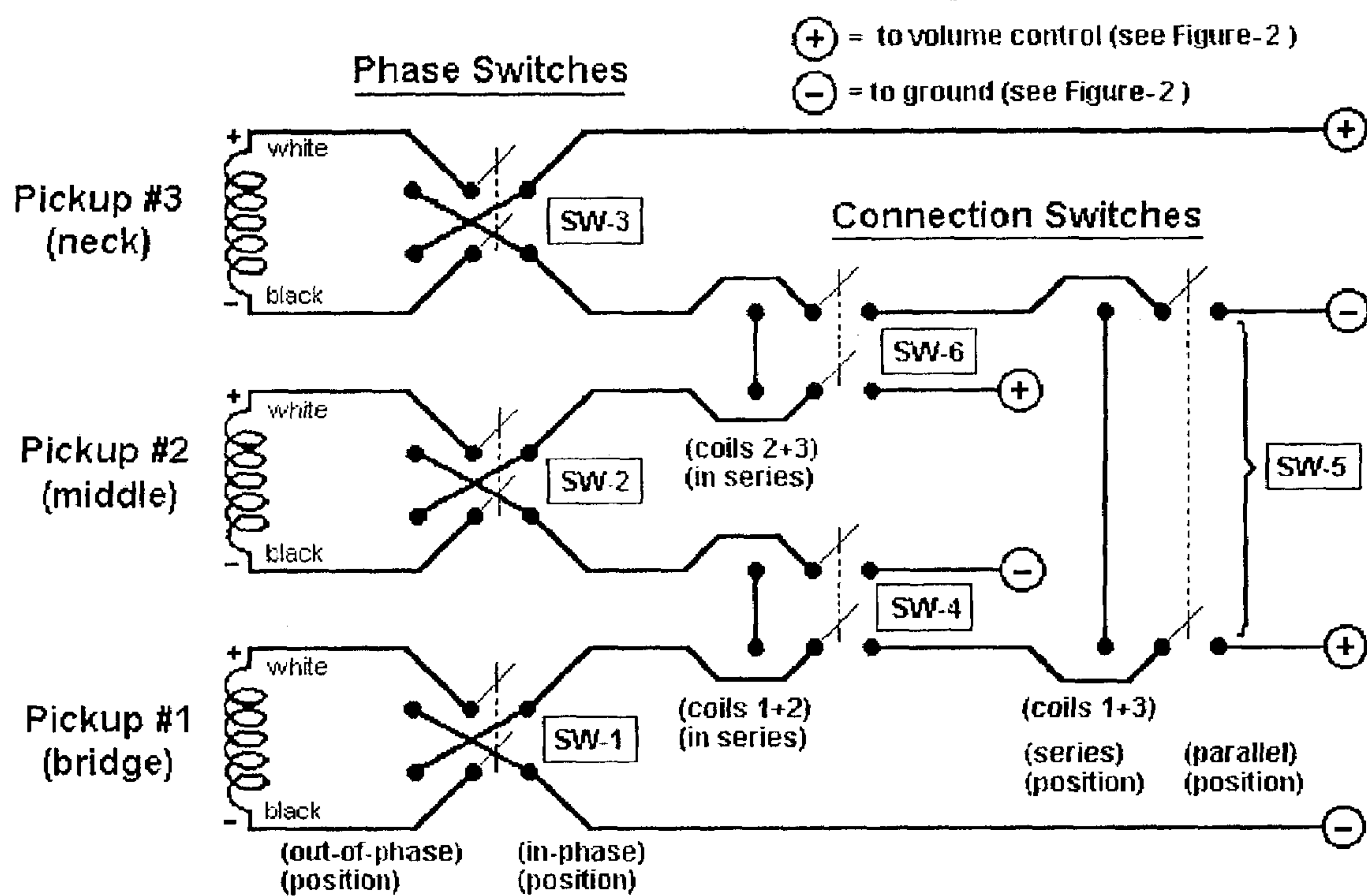
FIG. 1 - Revised Schematic For 3-Pickups
