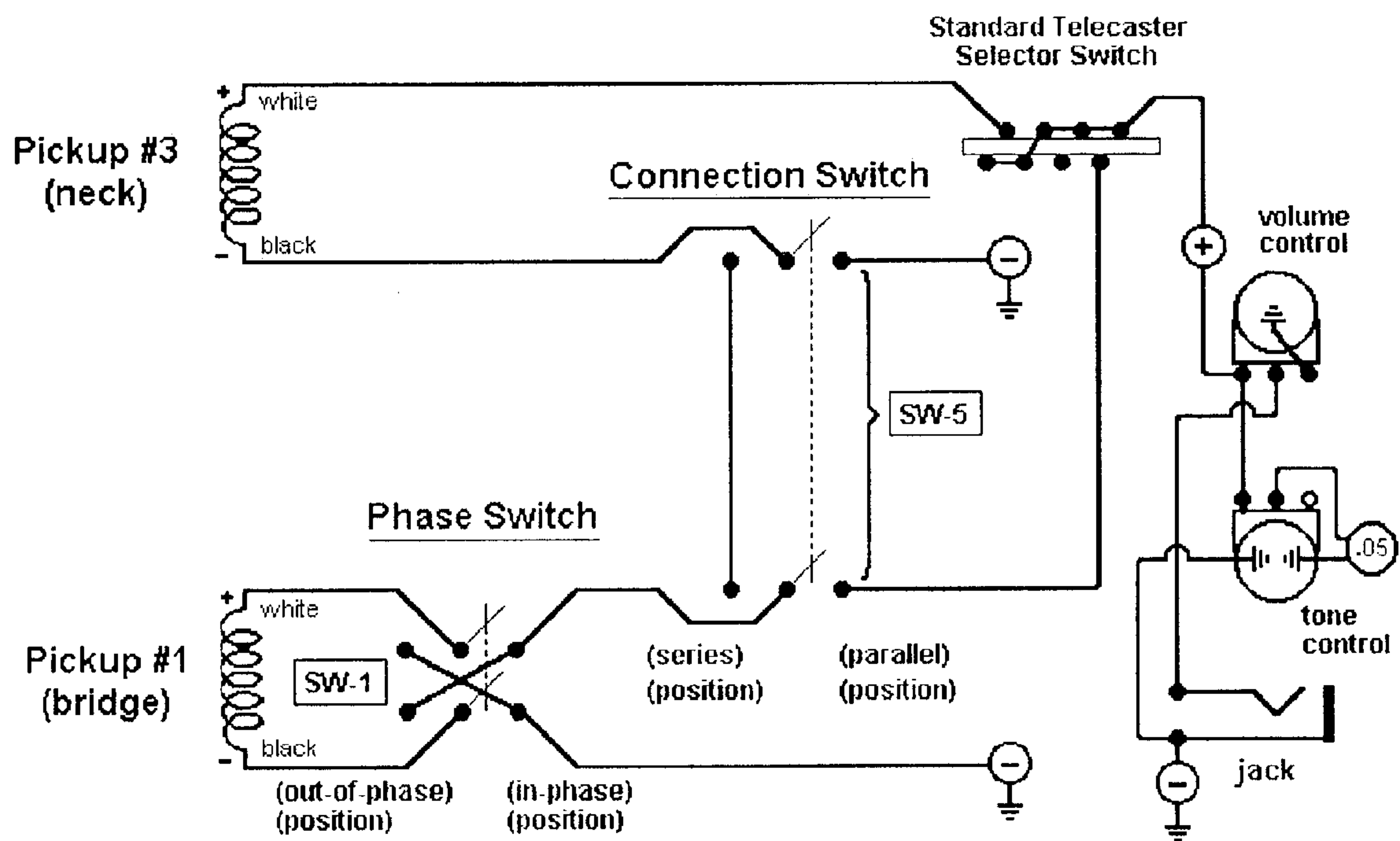
FIG. 5 – Revised Schematic For 2-Pickups Using existing 3-way switch
