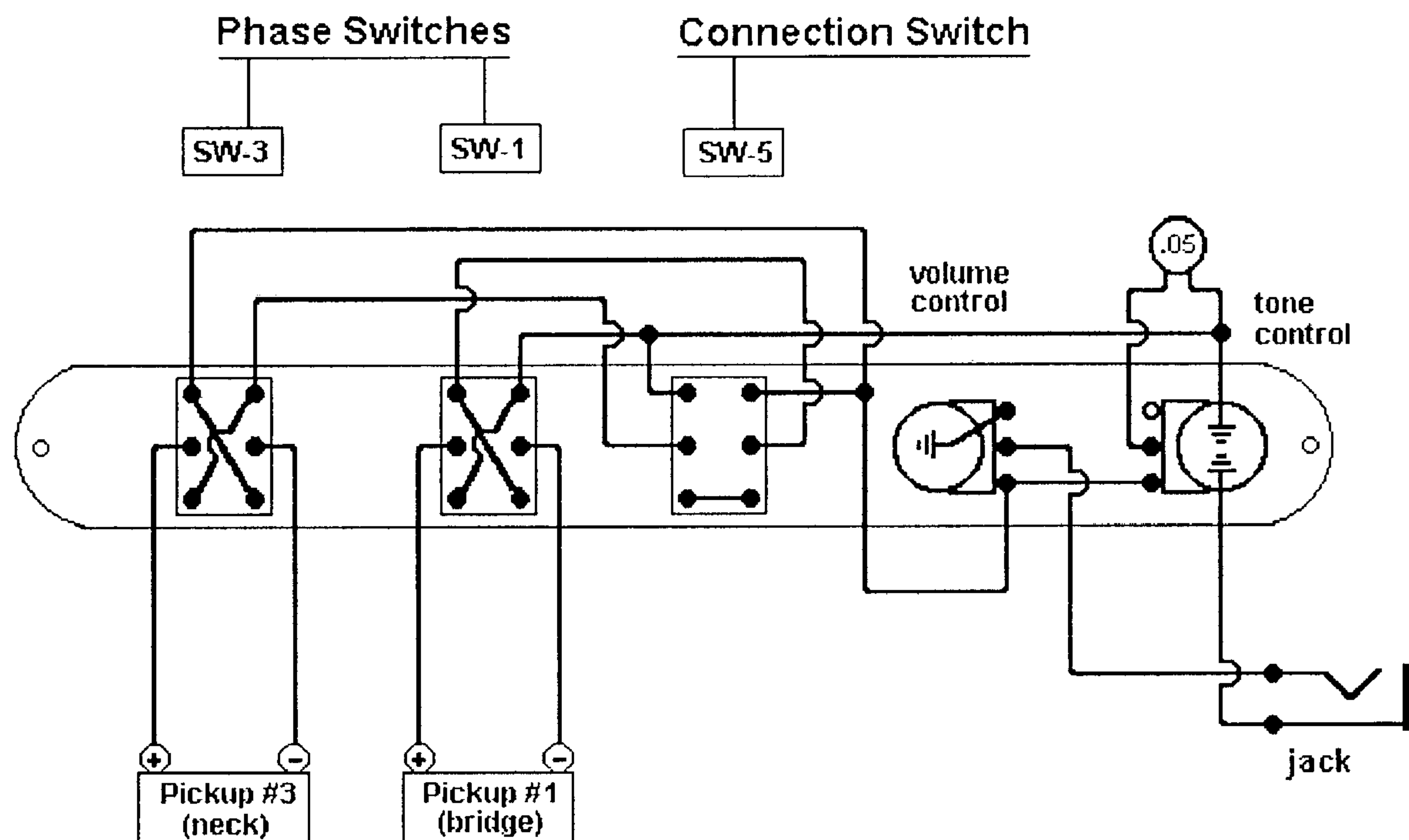
FIG. 4 – Wiring Diagram for 2-Pickups (Control Plate - rear view)
