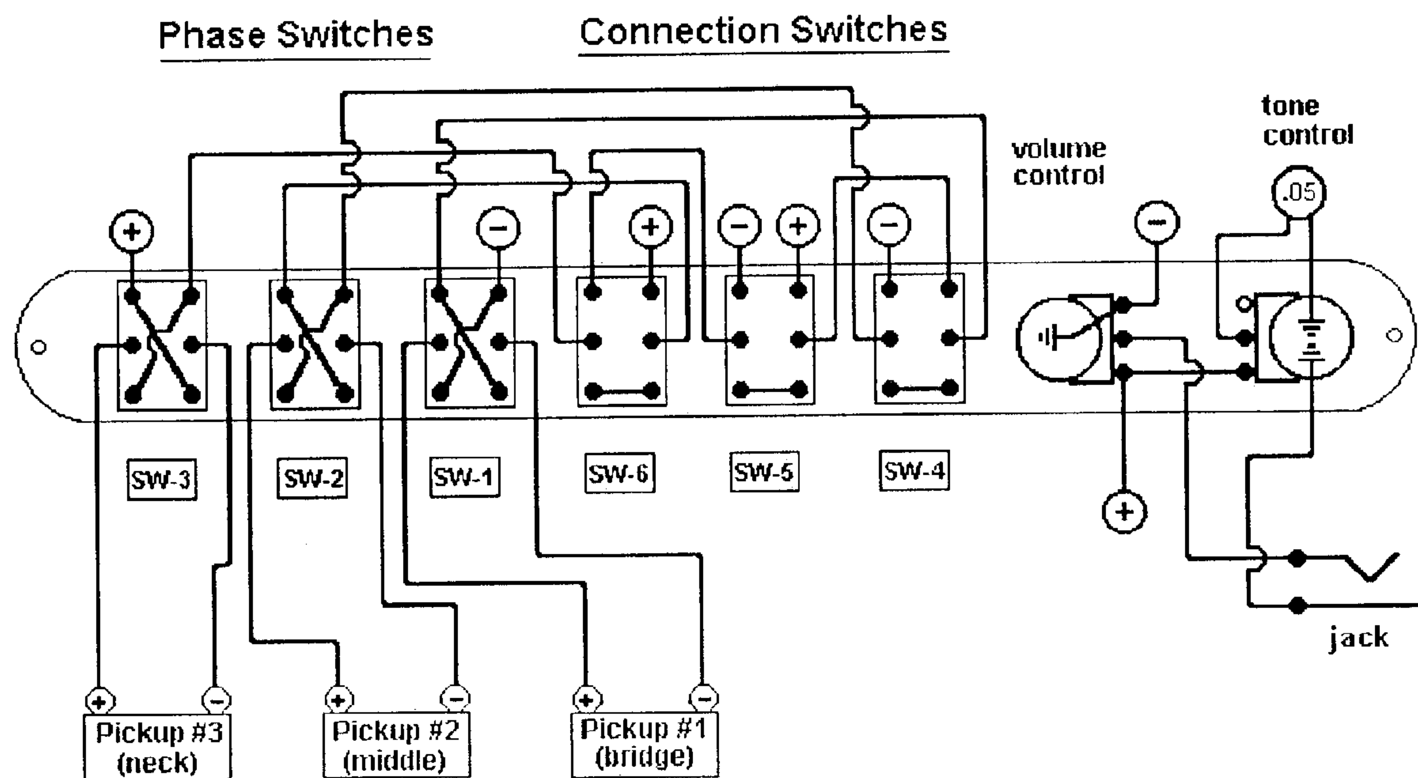
FIG. 2 – Wiring Diagram for 3-Pickups (Control Plate - rear view)
